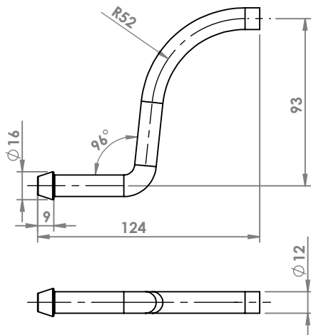
VW CADDY ATTACCO COD. AT 861306
