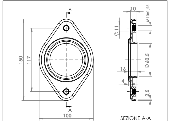
TOYOTA RAV4 FLANGIA COD. FL 801604
