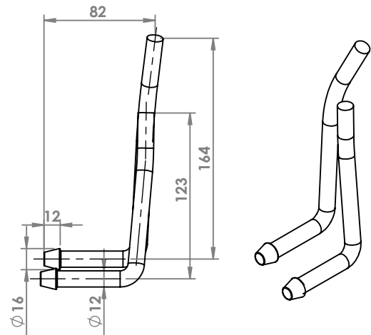
MITSUBISHI SPACE STAR ATTACCO COD. AT 460307
