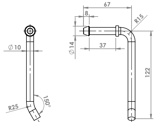
PEUGEOT 207 ATTACCO COD. AT 541503
