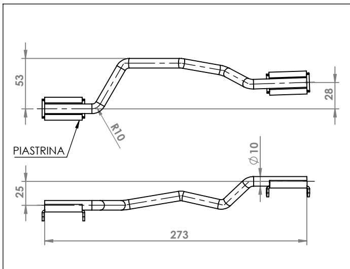
CITROEN XSARA ATTACCO COD. AT 141202
