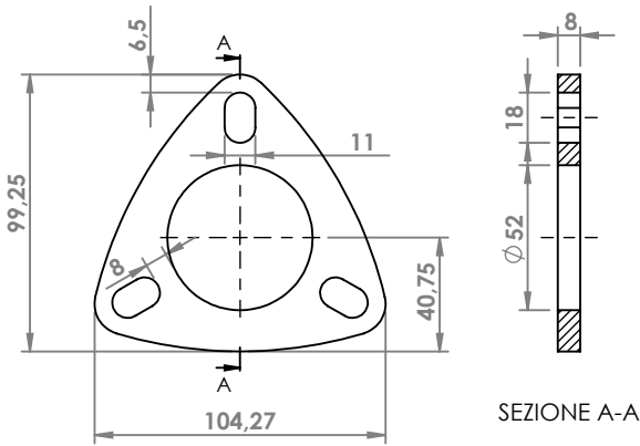
OPEL ASTRA 1.8 '00 FLANGIA COD. FL 520961
