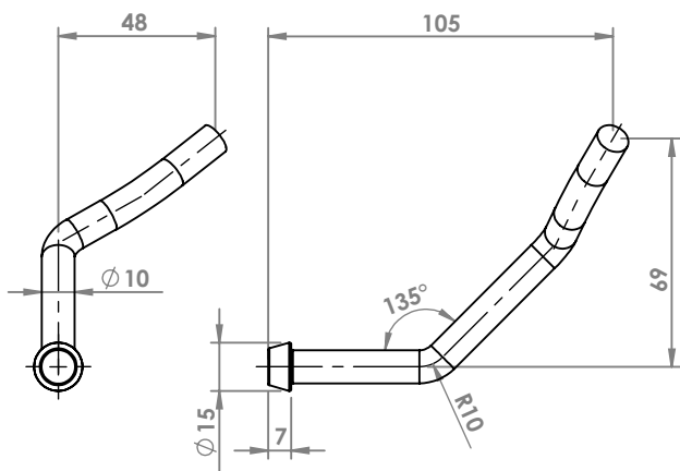
CITROEN C1 1.0 VRS '15 ATTACCO COD. AT 141710
