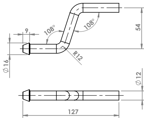
SEAT IBIZA 1.4 16V '06 ATTACCO COD. AT 680123
