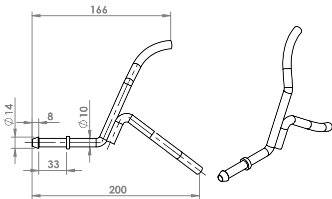
BMW E46 316 I ATTACCO COD. AT 120806
