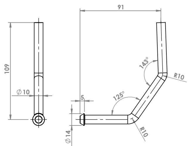
FIAT 500 ATTACCO COD. AT 242117
