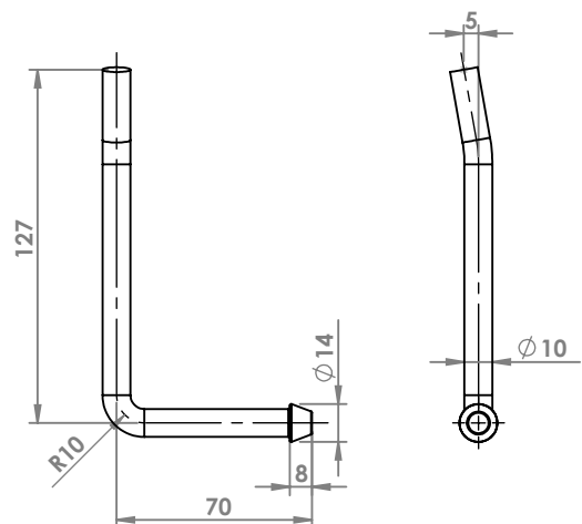
NISSAN ALMERA 1.5 - 1.8 '00 ATTACCO COD. AT 500710
