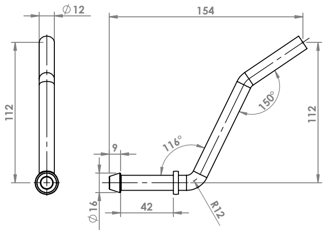
FORD GALAXY 2.0 '98 ATTACCO COD. AT 261112
