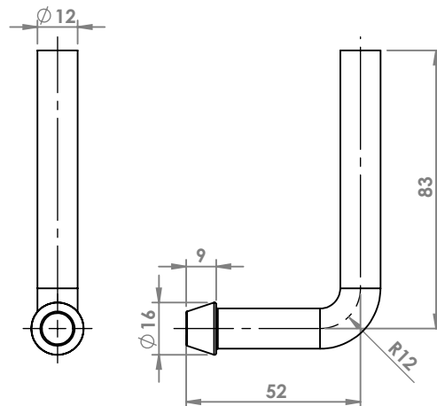
OPEL AGILA 1.0 | 12V '08 ATTACCO COD. AT 521209
