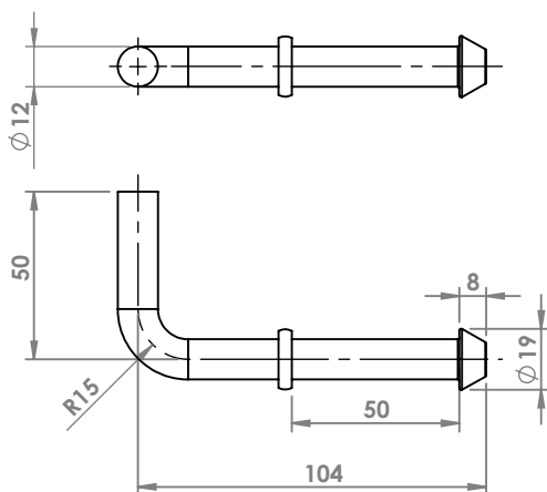
PEUGEOT 307 1.6 16V ATTACCO COD. AT 541317
