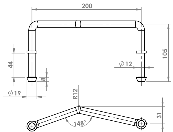
PEUGEOT 207 ATTACCO COD. AT 541501
