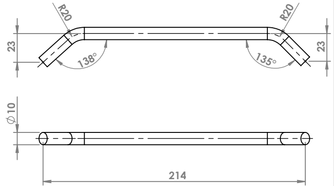
PEUGEOT 206 ATTACCO COD. AT 541238
