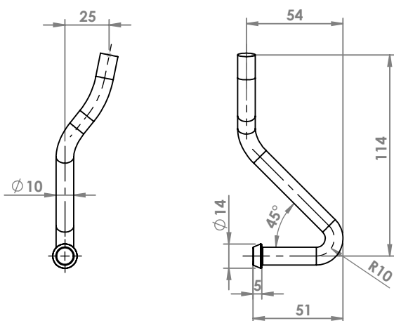
TOYOTA YARIS ATTACCO COD. AT 801220
