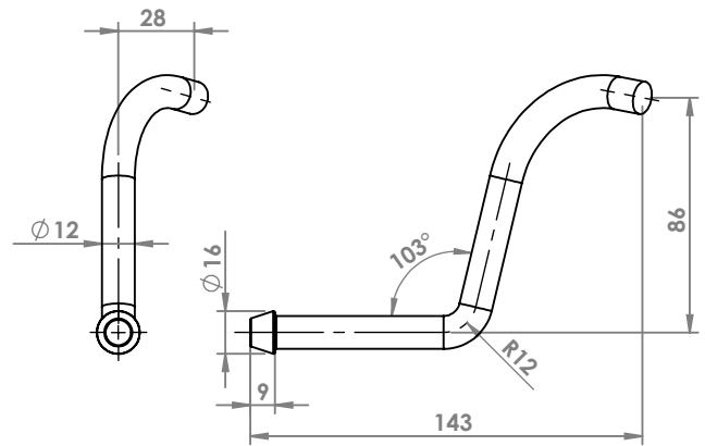
MERCEDES VITO ATTACCO COD. AT 440908
