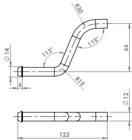
TOYOTA RAV4 2.0 16V '05 ATTACCO COD. AT 801609
