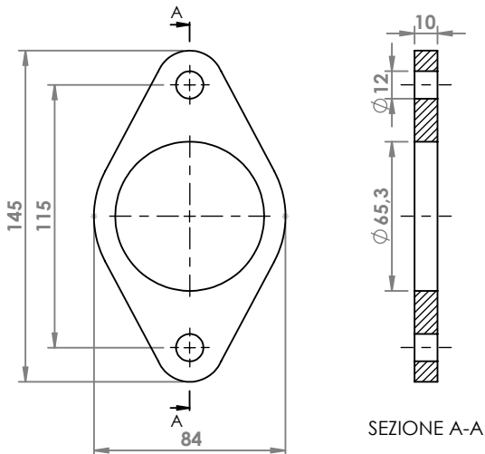
FORD FOCUS FLANGIA COD. FL 261522
