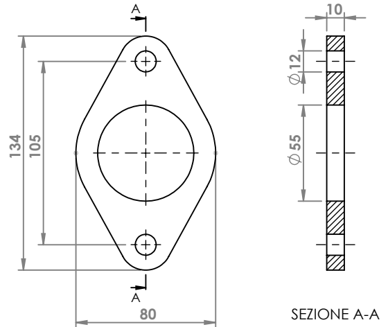
FORD FOCUS FLANGIA COD. FL 261521
