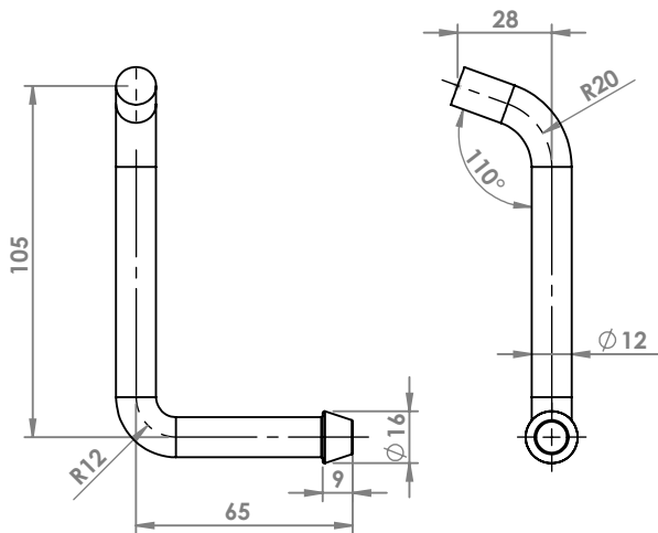
VW POLO ATTACCO COD. AT 860326
