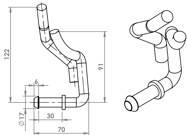
MERCEDES 200-230-300 ATTACCO COD. AT 440221
