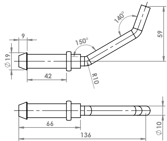
PEUGEOT 307 COUPE' ATTACCO COD. AT 541306
