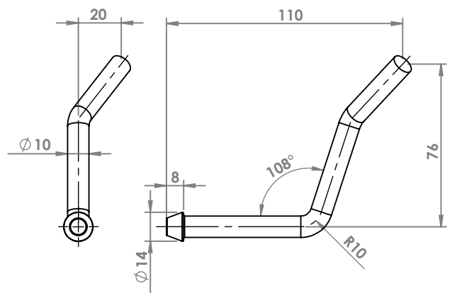
FORD FIESTA ATTACCO COD. AT 260374
