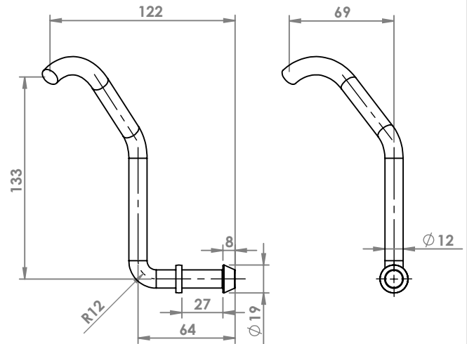
MERCEDES 200-230-300 ATTACCO COD. AT 440215
