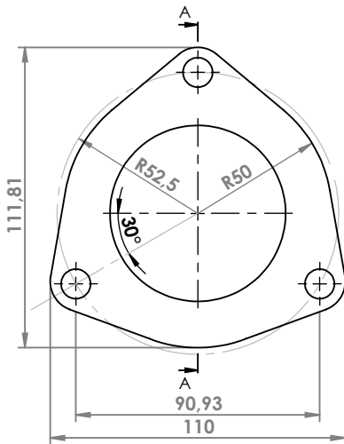
FIAT IVECO DAILY FLANGIA COD. FL 244001
