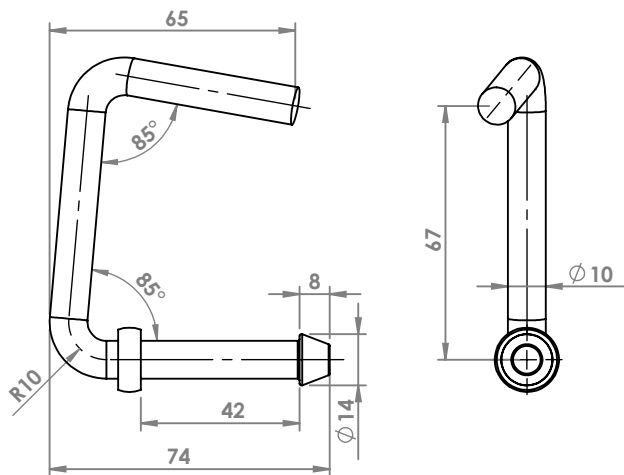
NISSAN QASHQAI 1.6 - 1.9 TD '06 ATTACCO COD. AT 500802
