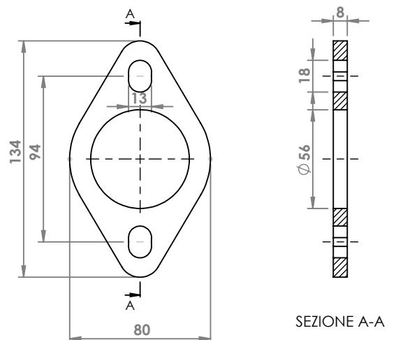
FORD FOCUS 1.4 '03 FLANGIA COD. FL 261525
