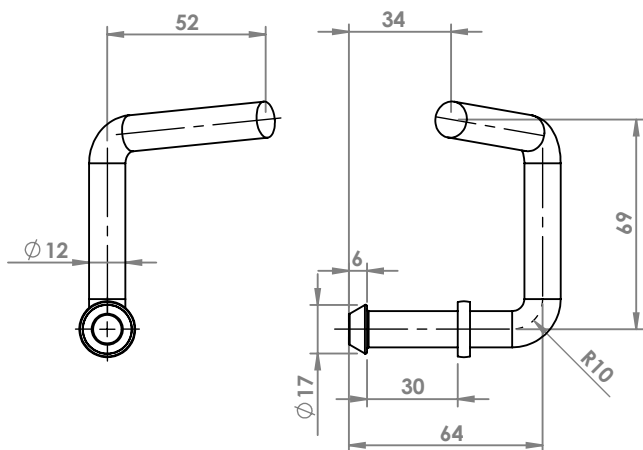
MERCEDES 200-230-300 ATTACCO COD. AT 440222
