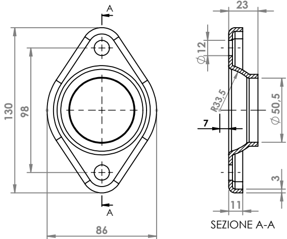
TOYOTA YARIS FLANGIA COD. FL 801216
