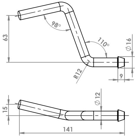
MERCEDES VITO 2.2 TD SWB - LWB '03 ATTACCO COD. AT 440907
