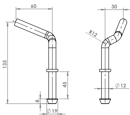
PEUGEOT 208 1.0 - 1.2 12V ATTACCO COD. AT 541602
