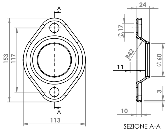
TOYOTA LAND CRUISER FLANGIA COD. FL 801302
