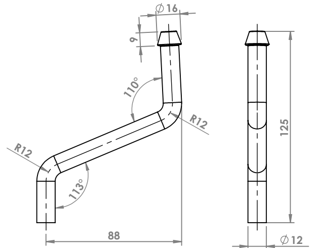
MERCEDES VITO ATTACCO COD. AT 440904
