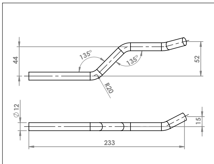
OPEL ASTRA 1.8 I ATTACCO COD. AT 520944
