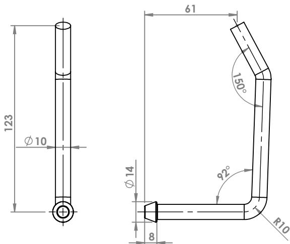
FORD TRANSIT 1.8 TDI ATTACCO COD. AT 261012
