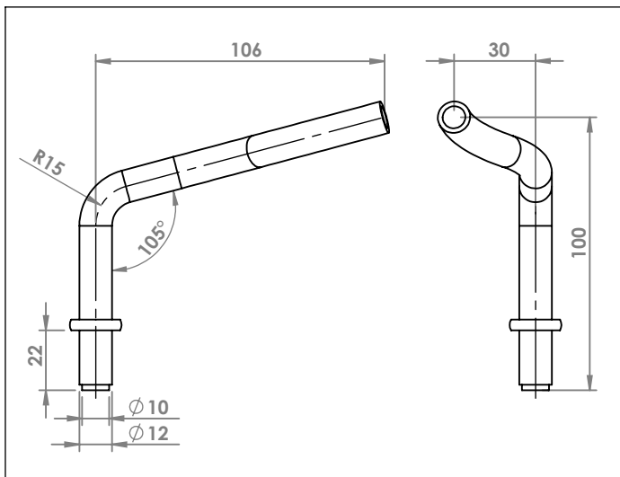
RENAULT ATTACCO COD. AT 601334
