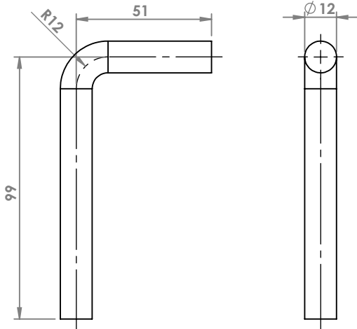
MERCEDES VITO ATTACCO COD. AT 440903
