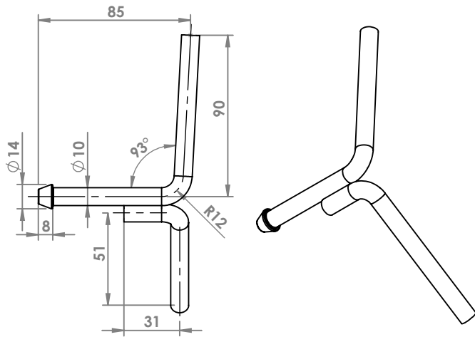
NISSAN NOTE ATTACCO COD. AT 500905
