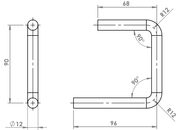
MERCEDES VITO ATTACCO COD. AT 440902
