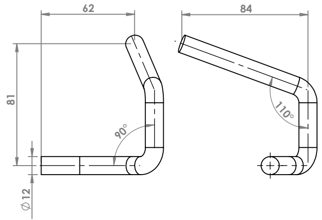
ALFA 159 ATTACCO COD. AT 021601
