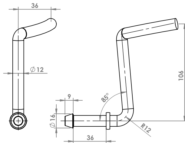
DAEWOO MATIZ 0.8 - 1.0 '05 ATTACCO COD. AT 160119
