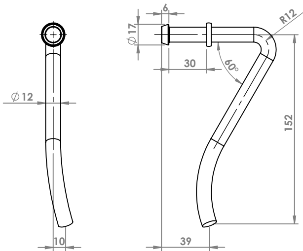
SKODA OCTAVIA ATTACCO COD. AT 690203
