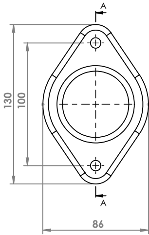
FIAT PALIO FLANGIA COD. FL 243013
