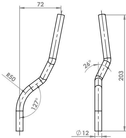
ALFA 159 ATTACCO COD. AT 021602
