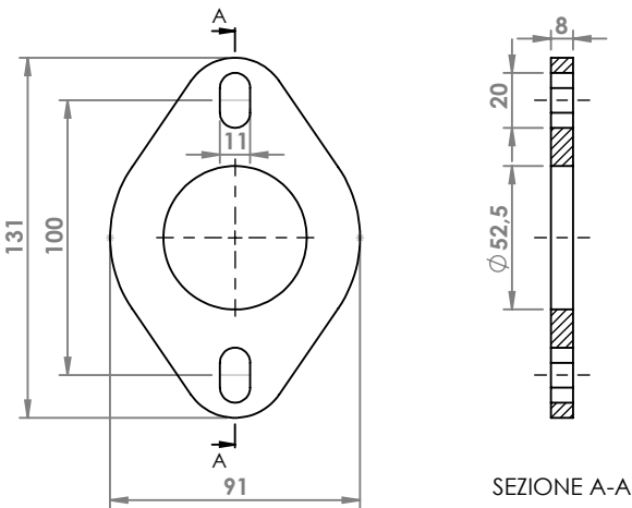
FORD FOCUS 1.6 16V '04 FLANGIA COD. FL 261517
