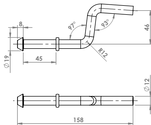
OPEL ASTRA ATTACCO COD. AT 520947
