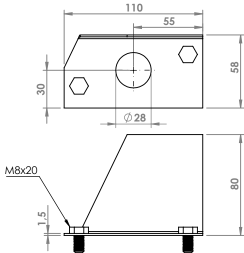
BMW ATTACCO COD. AT 120027 / PD
