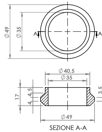
CITROEN DYANE 4 - 6 ANELLO \varnothing esterno mm 49 \varnothing interno mm 35 COD. AN 140802
