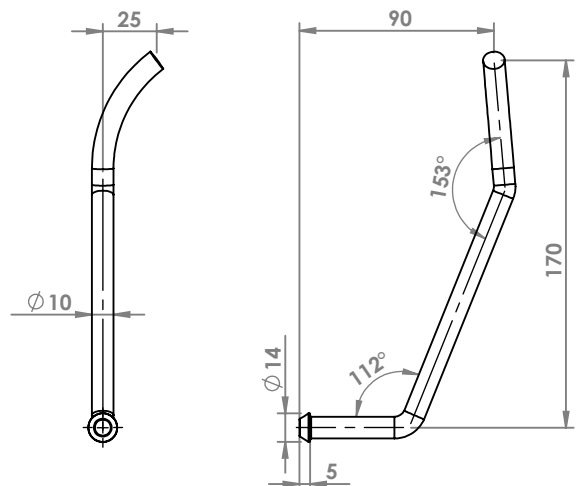
FIAT PANDA ATTACCO COD. AT 243614
