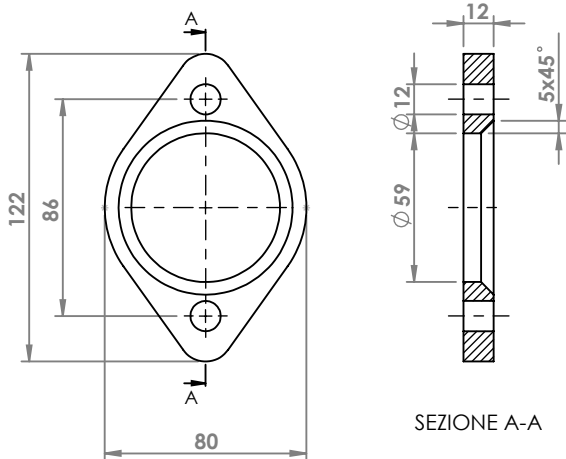
RENAULT R30 TURBO DIESEL FLANGIA COD. FL 600607
