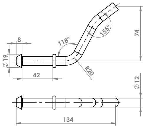
PEUGEOT 307 1.6 SW ATTACCO COD. AT 541313
