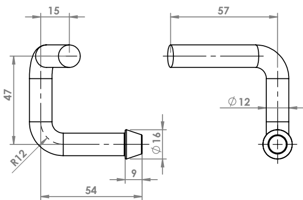
VW POLO ATTACCO COD. AT 860321
