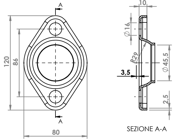
OPEL AGILA FLANGIA COD. FL 521211
