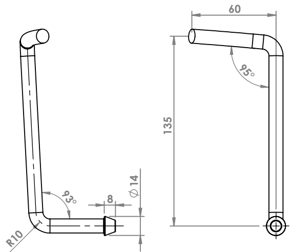
AUTO VARIE ATTACCO COD. AT 010044
