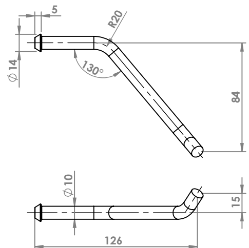
TOYOTA YARIS ATTACCO COD. AT 801222
