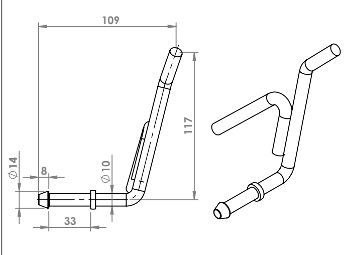
BMW E46 316 I ATTACCO COD. AT 120805
