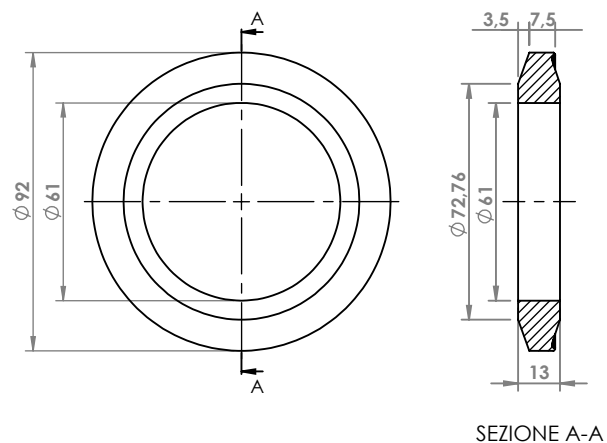
MERCEDES ANELLO COD. AN 440020
