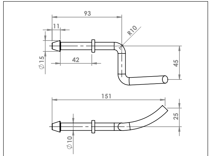
FORD MONDEO ATTACCO COD. AT 261229
