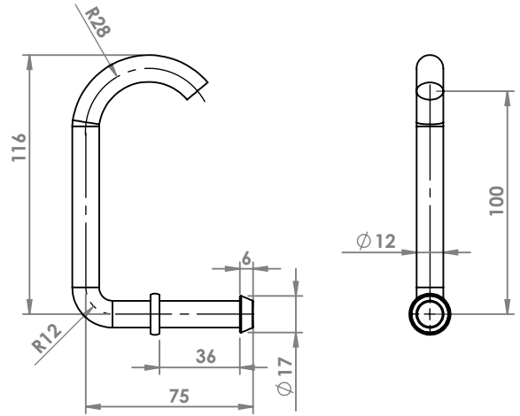
VW PASSAT 1.5 FSI '05 ATTACCO COD. AT 860217
