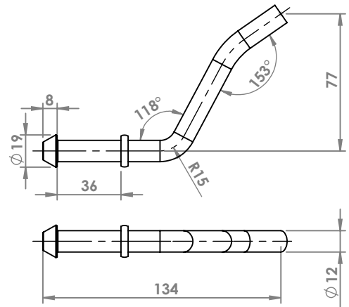
PEUGEOT 307 ATTACCO COD. AT 541316
