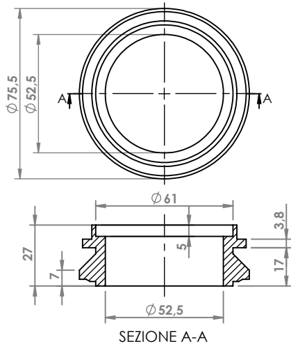
FIAT ANELLO COD. AN 240031
