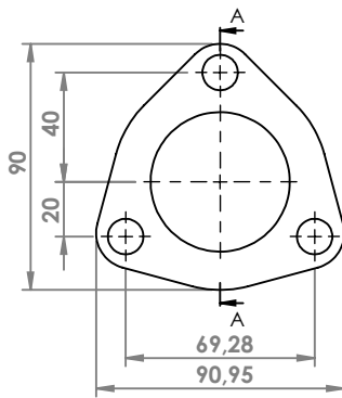
SEAT CORDOBA FLANGIA COD. FL 680615
