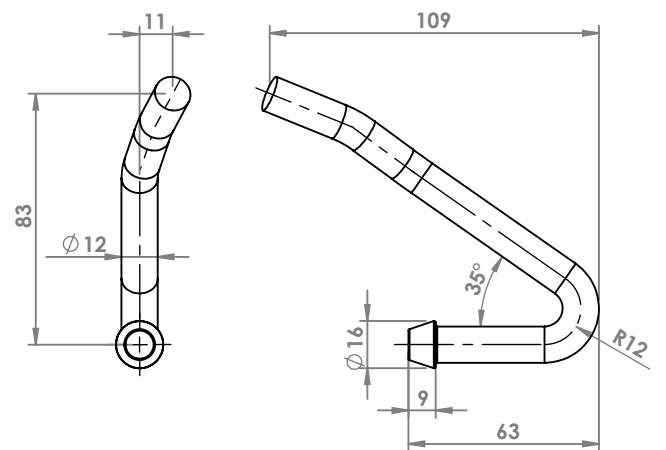
MERCEDES VITO 2.2 TD SWB - LWB '03 ATTACCO COD. AT 440906
