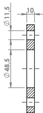
HYUNDAI GETZ 1.1 / 1.3 12V FLANGIA COD. FL 300604
