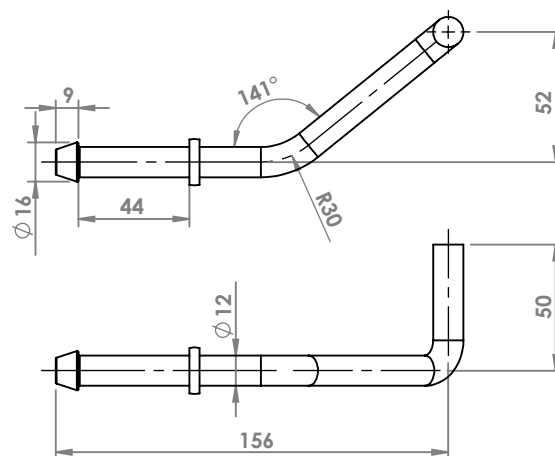
NISSAN QASHQAI 2.0 '06 ATTACCO COD. AT 500804
