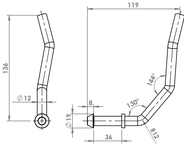
ALFA 156 2.5 I KAT V6 ATTACCO COD. AT 021202 / PD
