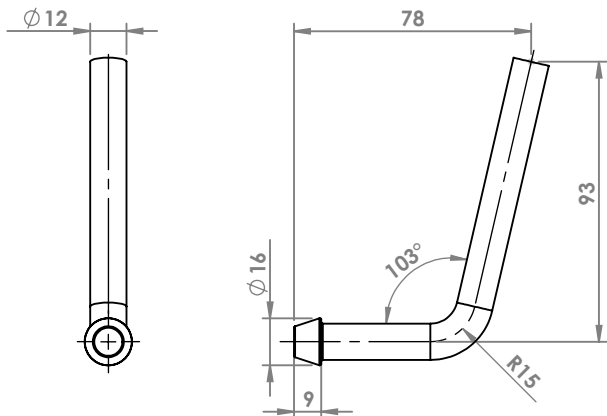
OPEL AGILA 1.0 | 12V '08 ATTACCO COD. AT 521208
