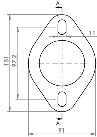
NISSAN QASHQAI 2.0 '06 FLANGIA COD. FL 500806
