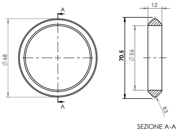
BMW ANELLO COD. AN 120031
