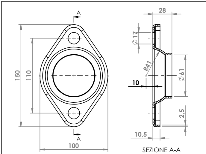
TOYOTA RAV4 FLANGIA COD. FL 801605
