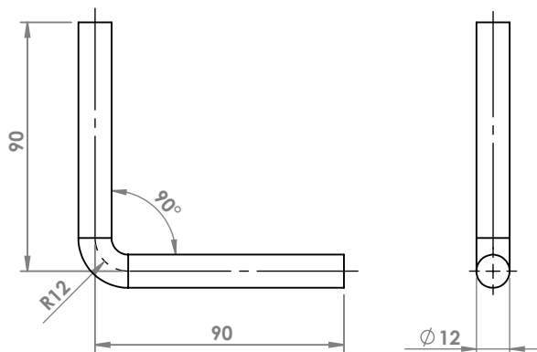
OPEL MERIVA ATTACCO COD. AT 521506
