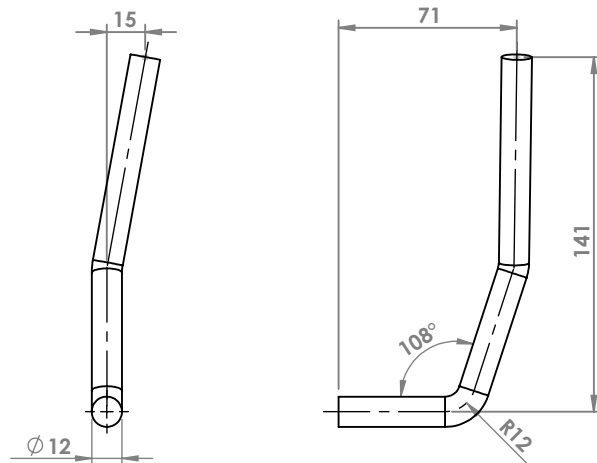
OPEL CORSA 1.3 COMBO TD '03 ATTACCO COD. AT 520330
