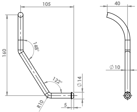
FIAT PANDA ATTACCO COD. AT 243615
