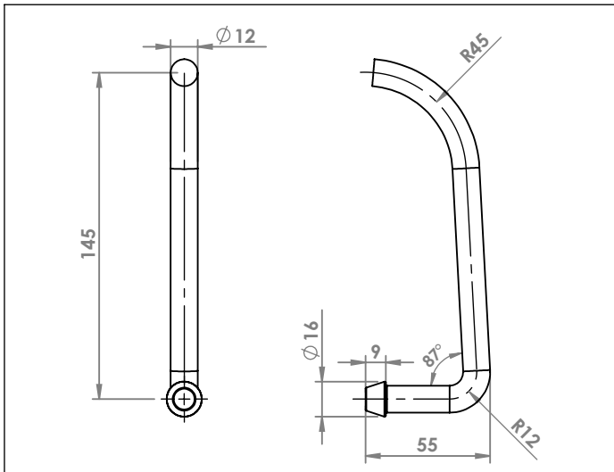
AUDI A2 ATTACCO COD. AT 040617
