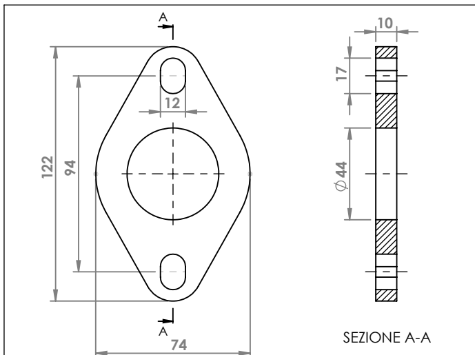
DAIHATSU FEROZA FLANGIA COD. FL 180308
