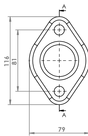
NISSAN ALMERA FLANGIA COD. FL 500705
