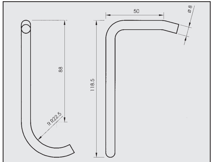
RENAULT CLIO 1.8 16V ATTACCO COD. AT 601305
