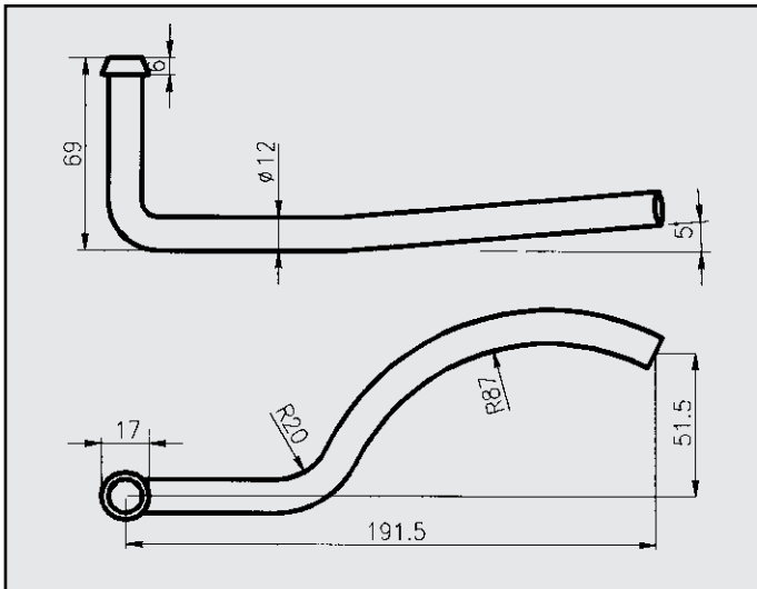
FIAT ULISSE 2.0 IE TD 1.9 2.1 ATTACCO COD. AT 242706
