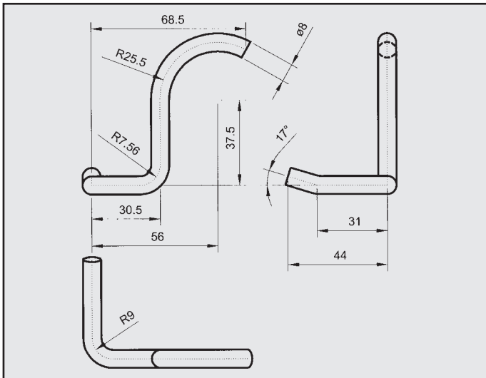
RENAULT TRAFFIC 2,0 DIESEL ATTACCO posteriore COD. AT 601204
