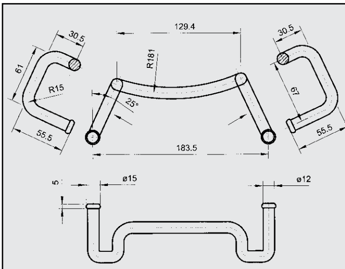
FIAT IVECO S 2000 STAFFA ANTERIORE COD. AT 242502
