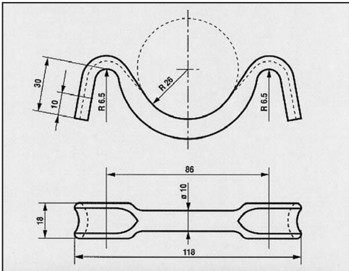
OPEL VECTRA ATTACCO COD. AT 520805
