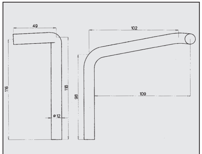
VOLKSWAGEN GOLF ATTACCO COD. AT 861003
