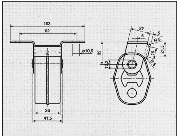
SEAT ATTACCO COD. AT 680004
