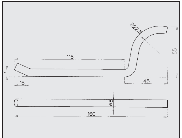
TICO ATTACCO COD. AT 790005
