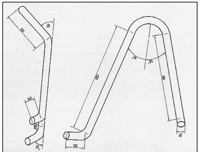
ACURA LEGEND 2 DOOR 87/88 ATTACCO COD. AT 280901
