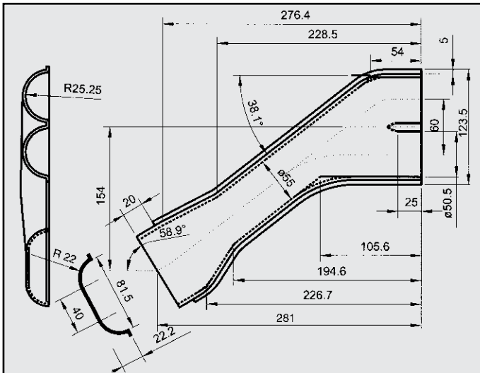
BMW 525i KAT MANICOTTO 2 VIE COD. M 120210
