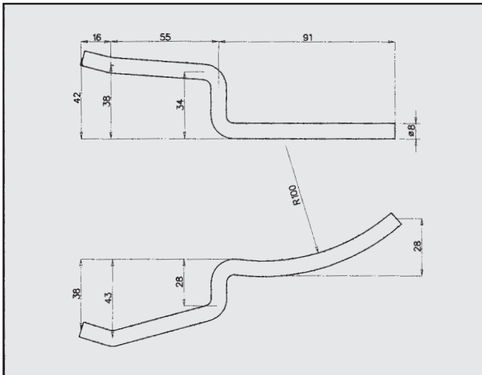
RENAULT KANGOO 1.4 ATTACCO COD. AT 601701
