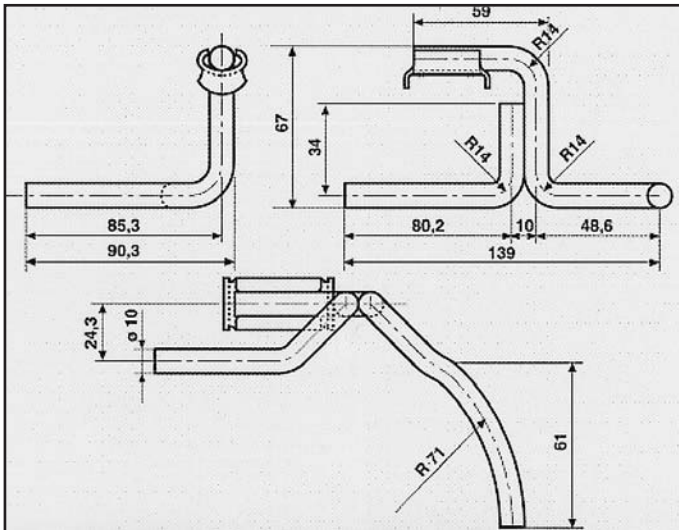
FORD ESCORT ATTACCO posteriore COD. AT 260240
