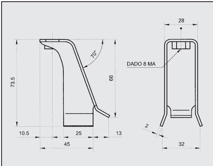
SUZUKI VITARA 1.6 JLX JLX SE ATTACCO COD. AT 720108
