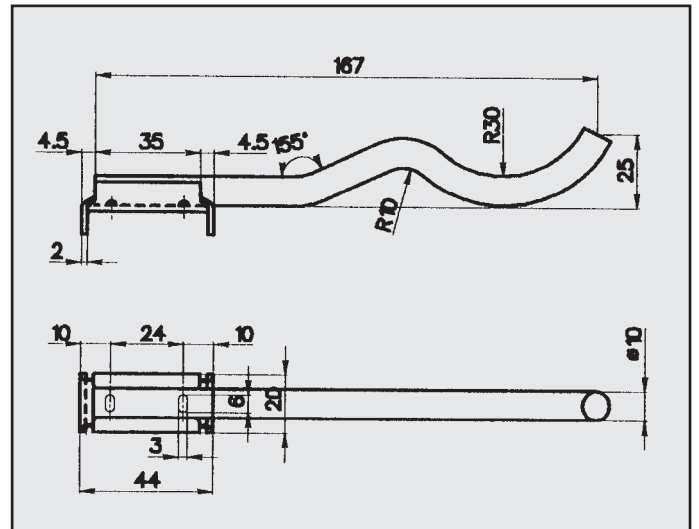
FORD ATTACCO COD. AT 260012
