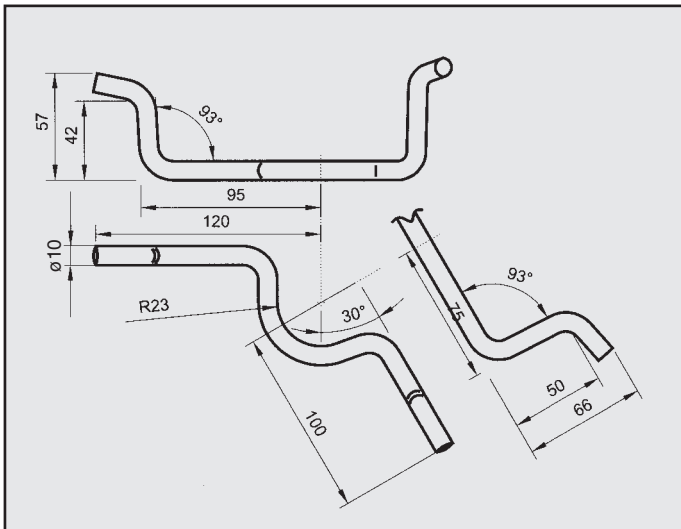
ROVER 416 1.6 16V ATTACCO COD. AT 620701
