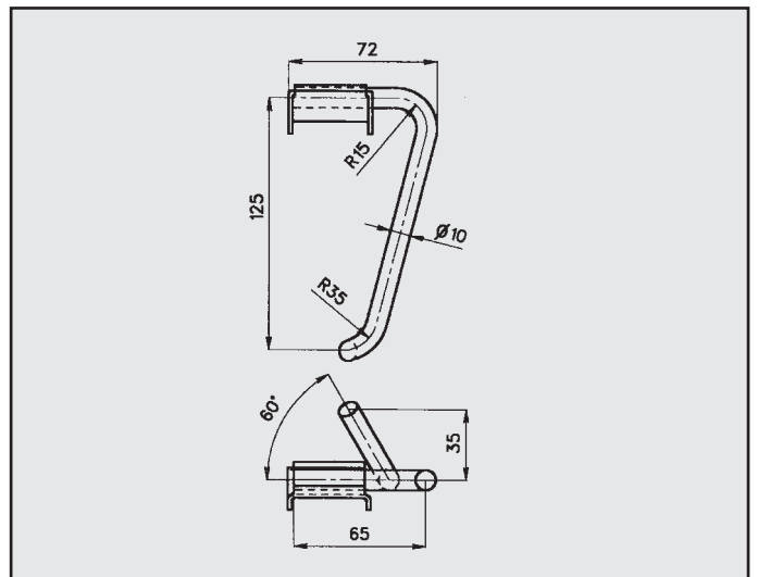
FORD ESCORT ATTACCO COD. AT 260253
