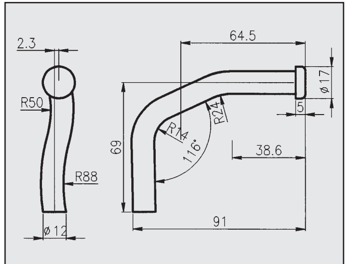
OPEL OMEGA ATTACCO COD. AT 520614
