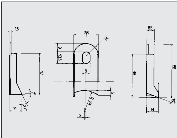
GIULIETTA ATTACCO per posteriore COD. AT 020212 116503000309 116973000303 116503000304 116503000300
