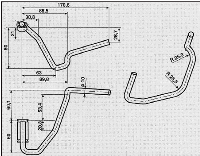
FORD ATTACCO COD. AT 260007
