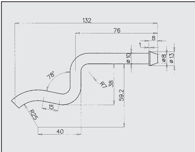
FORD FOCUS 1.6 ATTACCO COD. AT 261510
