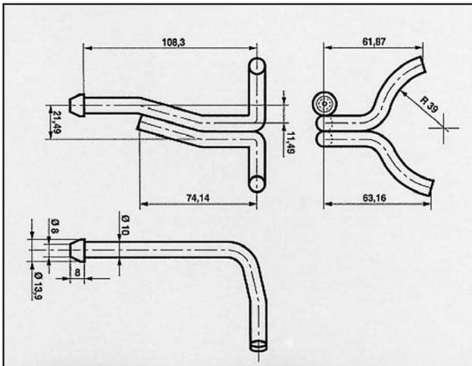
FORD SCORPIO ATTACCO COD. AT 260805
