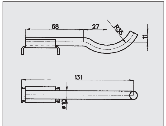
FORD ATTACCO COD. AT 260013
