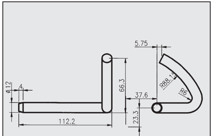
VOLKSWAGEN ATTACCO COD. AT 860010
