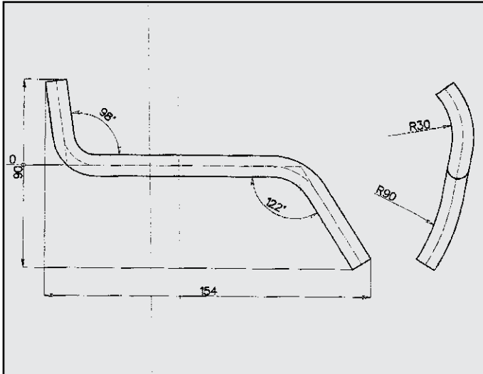
BMW 320 ATTACCO COD. AT 120409
