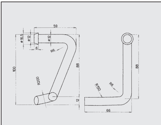
TOYOTA YARIS ATTACCO COD. AT 801202
