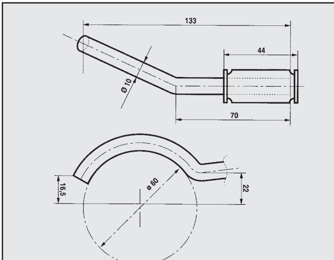
FORD ESCORT RS TURBO ATTACCO posteriore COD. AT 260248
