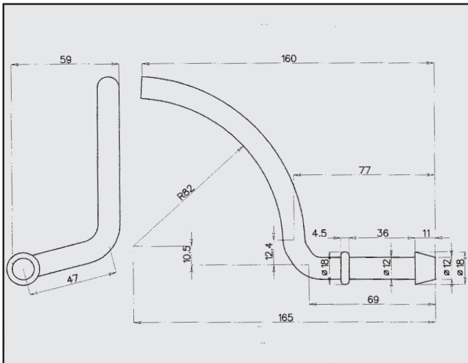
FORD GALAXY ATTACCO COD. AT 261107
