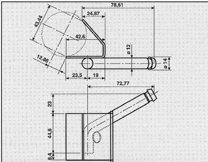
SEAT ATTACCO COD. AT 680002
