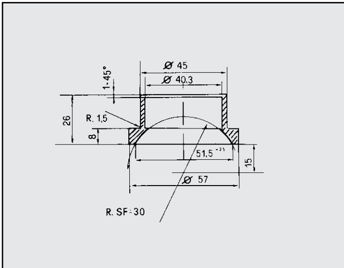
CITROEN PEUGEOT ANELLO \varnothing esterno mm 57 COD. AN 140001
