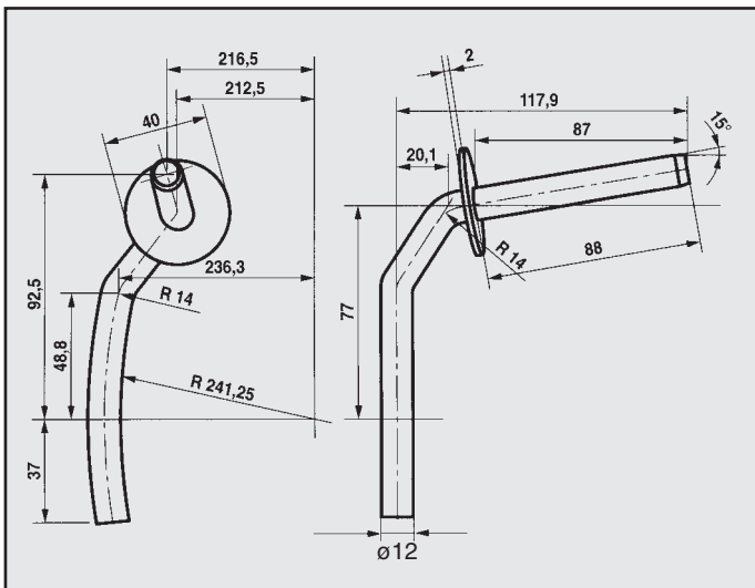
VOLKSWAGEN TRANSPORTER 2.4 D ATTACCO COD. AT 861102
