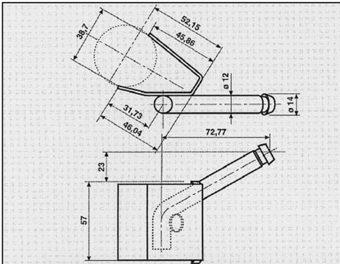
SEAT ATTACCO COD. AT 680001
