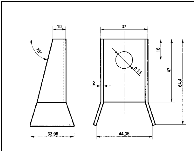
BMW ATTACCO COD. AT 120007
