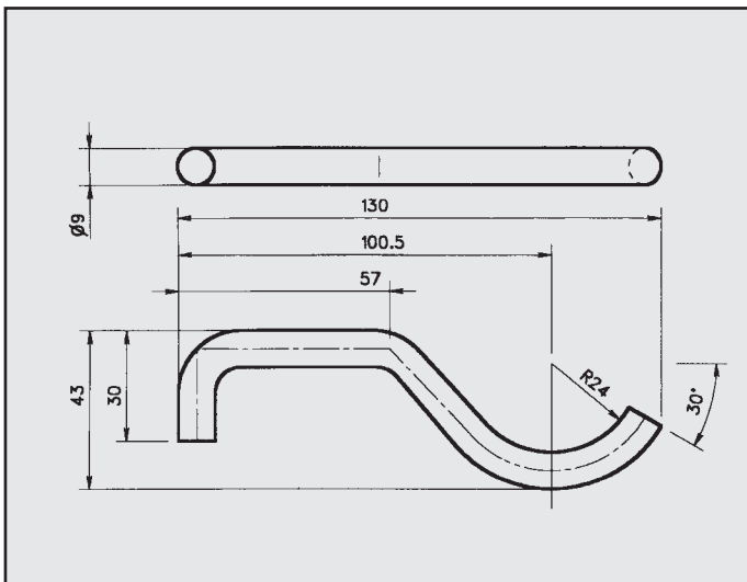
HONDA BALLADE SPORT ATTACCO per posteriore COD. AT 2280302
