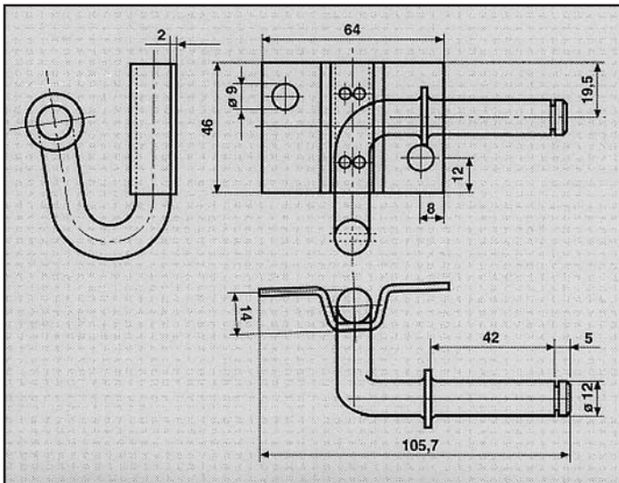
OPEL ATTACCO COD. AT 520002
