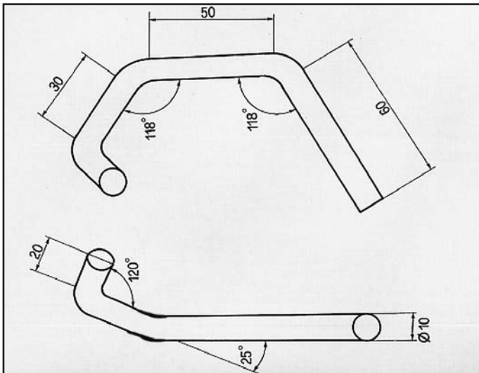
ACURA LEGEND 86-88 USA ATTACCO COD. AT 280903
