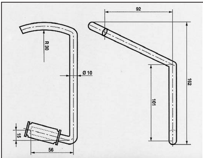
FORD ESCORT RS TURBO ATTACCO posteriore COD. AT 260249
