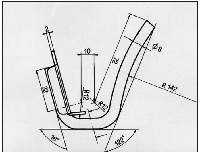
KADETT GSI ATTACCO COD. AT 520105
