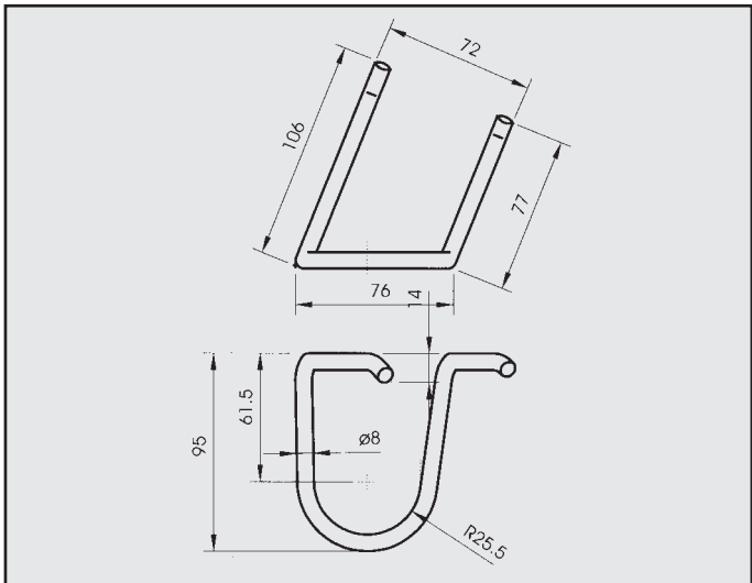
RENAULT ATTACCO COD. AT 600001
