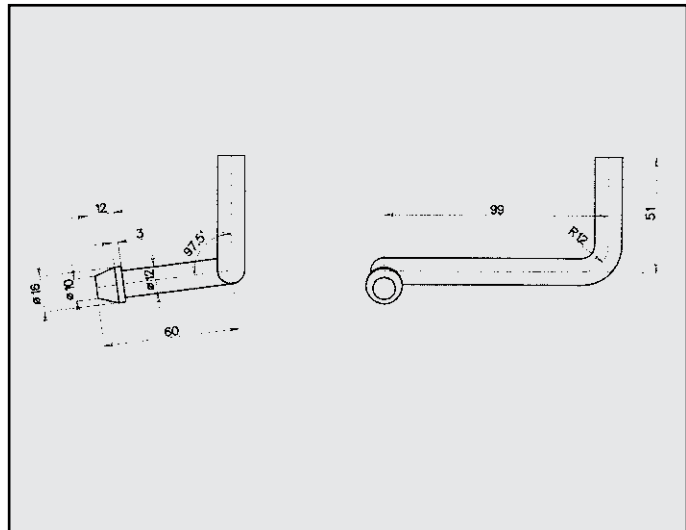
DAEWOO NUBIRA 1.6 ATTACCO POSTERIORE COD. AT 160304
