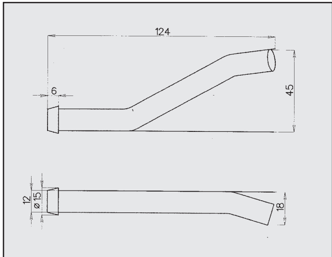
VOLVO S40-V40 ATTACCO COD. AT 880902
