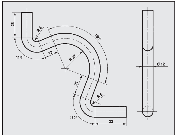
OPEL VECTRA 2.0 CAT ATTACCO COD. AT 520814
