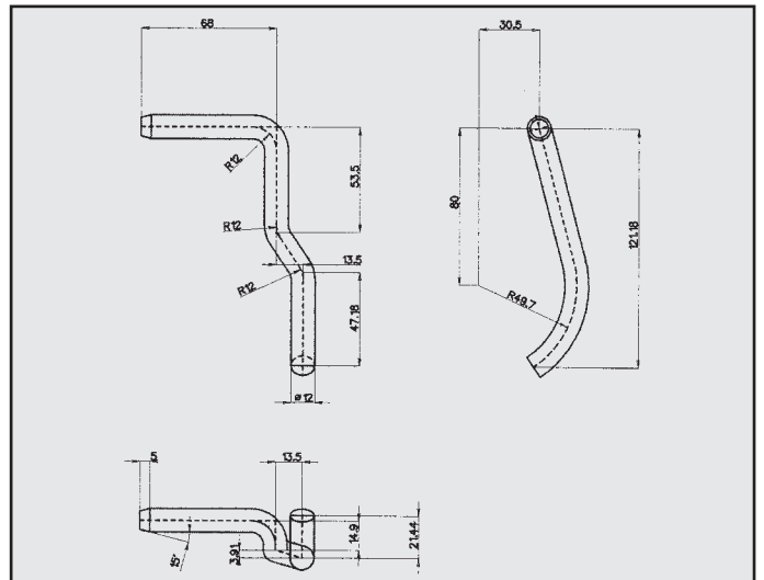
VOLKSWAGEN CADDY ATTACCO COD. AT 861301
