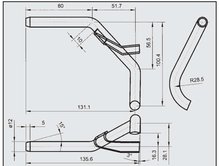
VOLKSWAGEN ATTACCO COD. AT 860004
