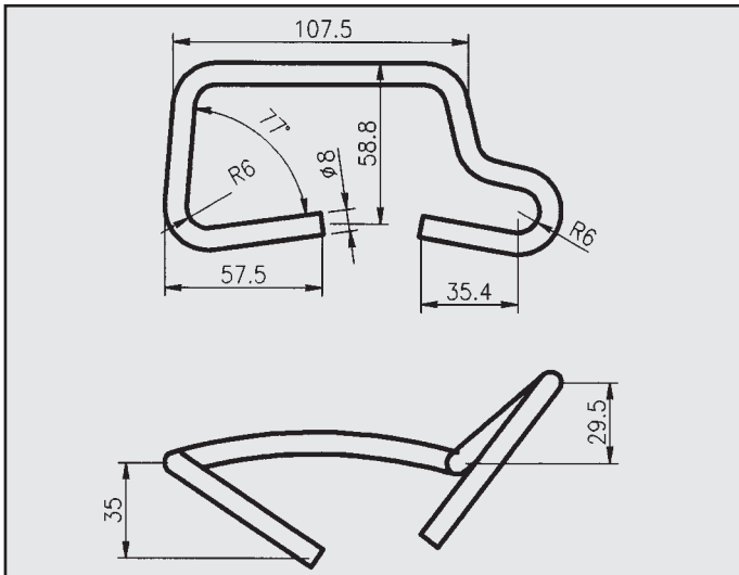
RENAULT 19 ATTACCO COD. AT 600913
