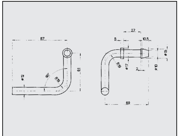
FIAT ATTACCO COD. AT 240018
