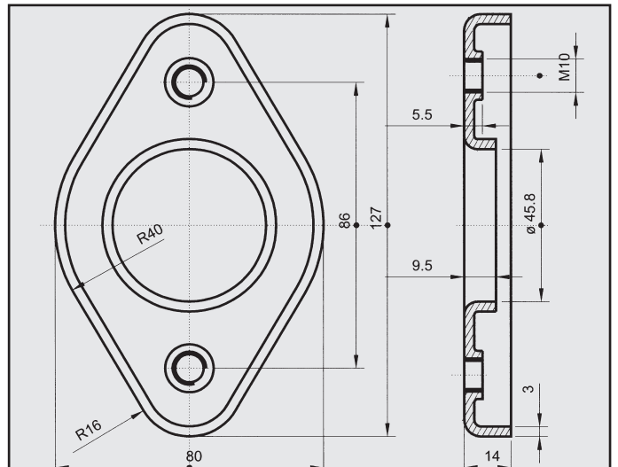
OPEL KADETT FLANGIA COD. FL 520111
