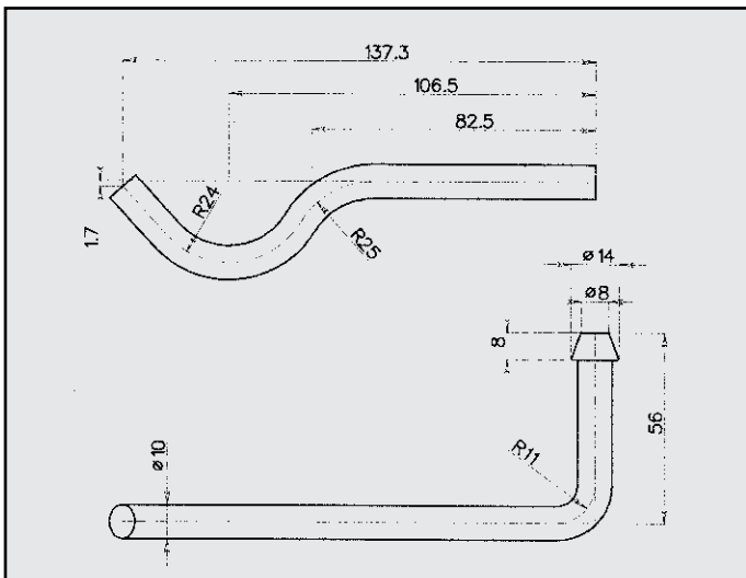
FIAT ATTACCO COD. AT 240017
