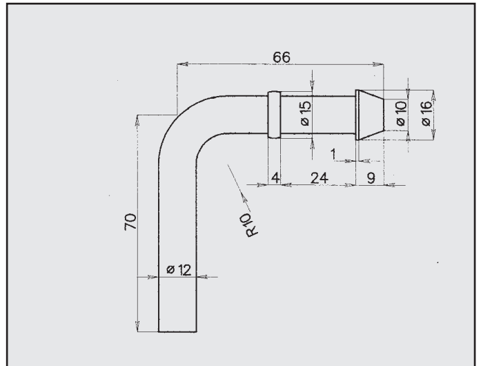
OPEL AGILA ATTACCO COD. AT 521202
