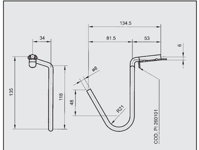
FORD ESCORT - ORION 1.300 ATTACCO COD. AT 260231
