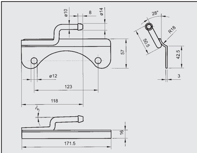
MASERATI ATTACCO COD. AT 400001
