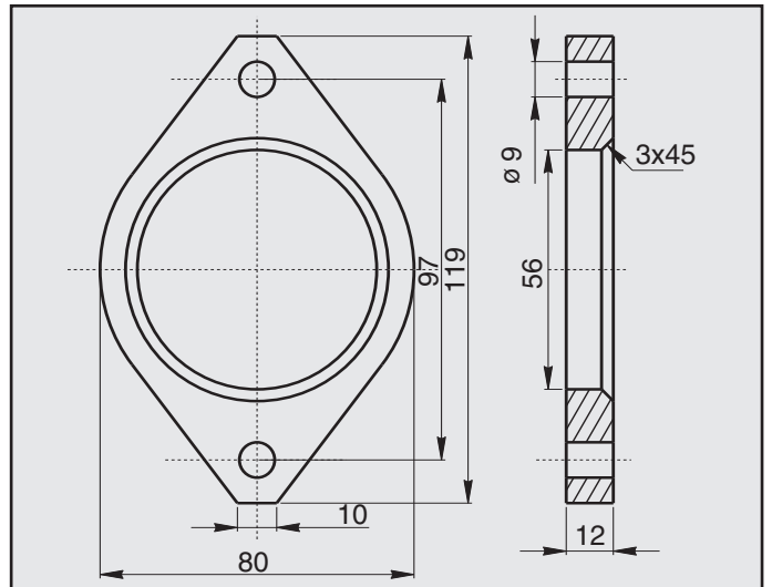
OPEL VECTRA 1.7 TURBO DIESEL FLANGIA COD. FL 520824
