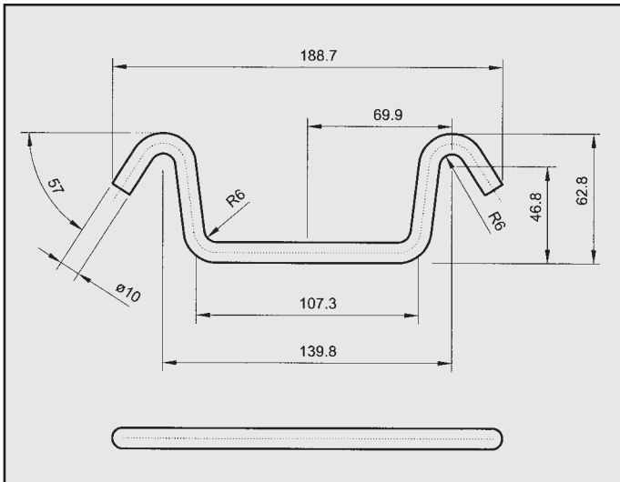
OPEL CALIBRA ATTACCO COD. AT 521002
