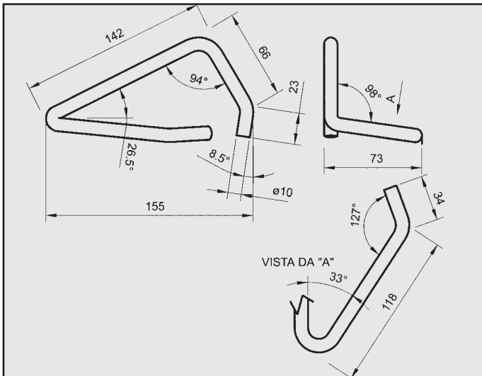
ROVER ATTACCO COD. AT 620002
