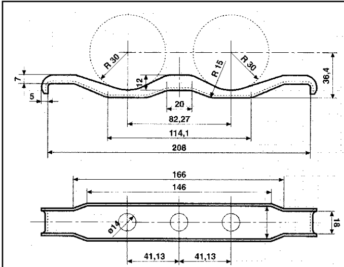
BMW ATTACCO COD. AT 120002
