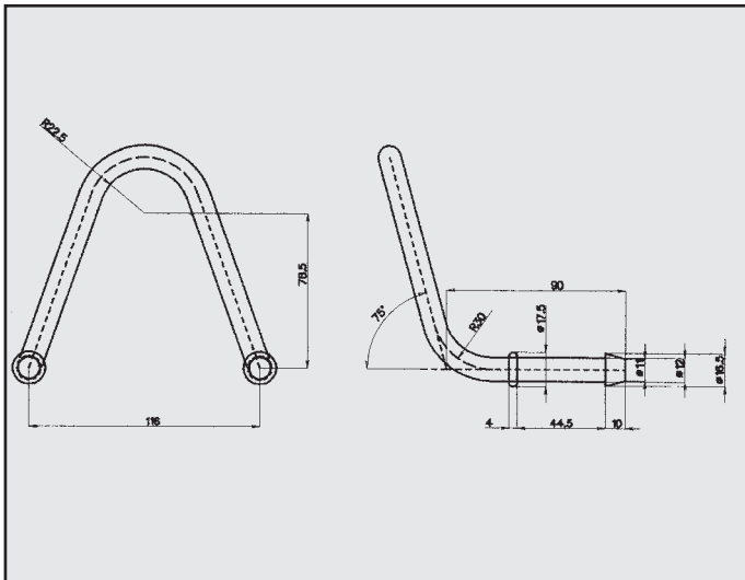
PEUGEOT ATTACCO COD. AT 540001
