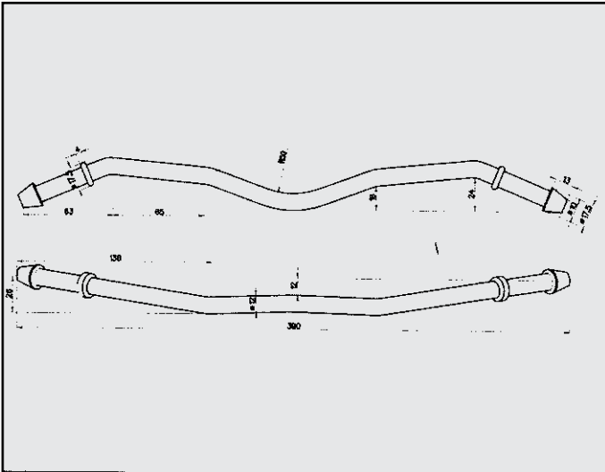
ALFA 167 ATTACCO COD. AT 021402
