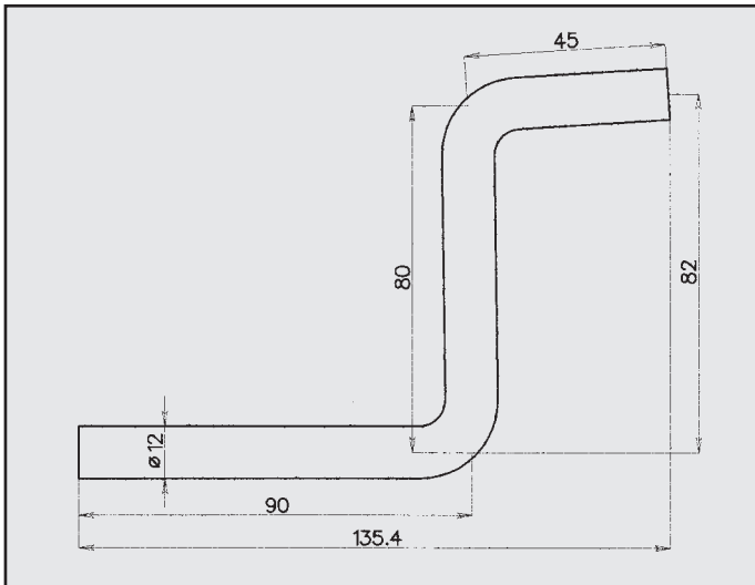
SAAB 900 ATTACCO COD. AT 640210
