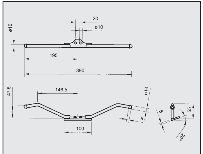
MASERATI ATTACCO COD. AT 400004
