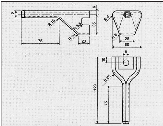
VOLKSWAGEN ATTACCO COD. AT 860002
