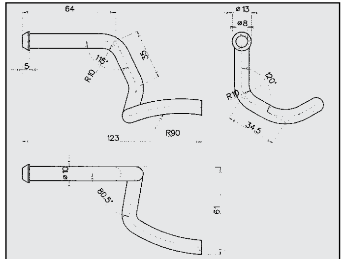
FIAT STILO ATTACCO COD. AT 243503
