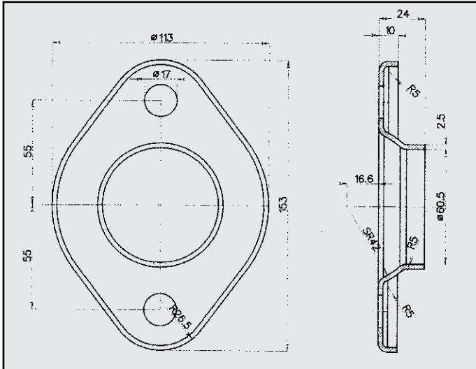
TOYOTA LEXUS FLANGIA COD. FL 801401
