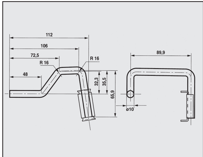
CITROEN ZX 1900 ATTACCO COD. AT 140904 96070794
