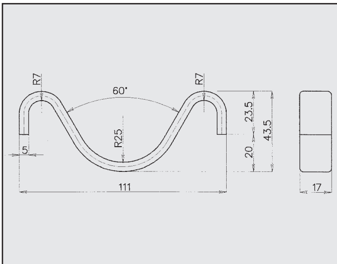
TICO ATTACCO COD. AT 790010
