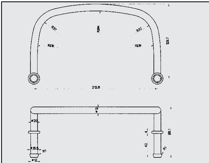
FERRARI ATTACCO COD. AT 220002
