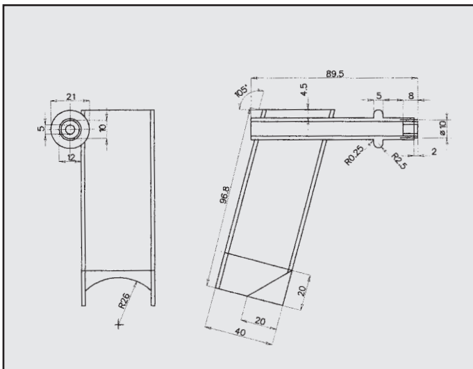
RENAULT CLIO ATTACCO COD. AT 601311
