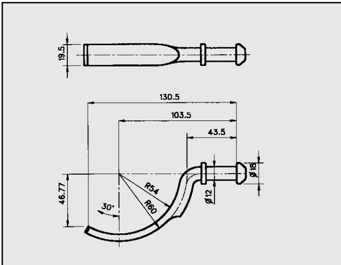
CHRYSLER VOYAGER ATTACCO COD. AT 130102
