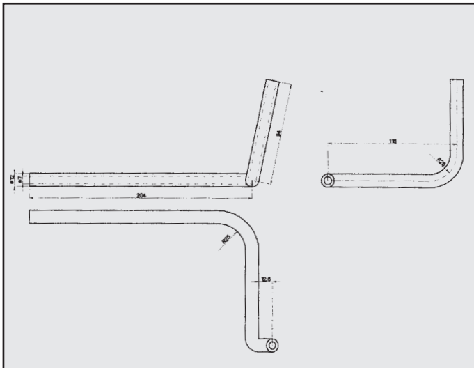
MERCEDES VITO ATTACCO COD. AT 440901
