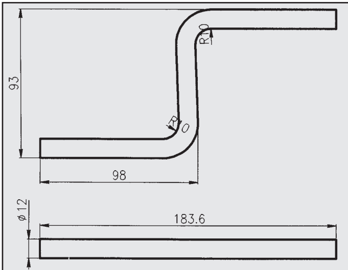
OPEL VECTRA ATTACCO COD. AT 520820
