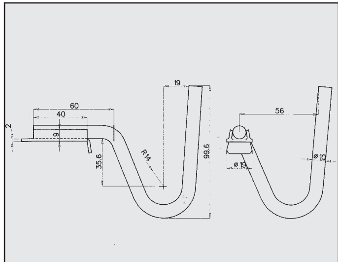
FORD ESCORD ATTACCO COD. AT 260203
