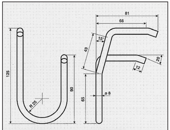
RENAULT 21 NEVADA 1.7 TS ATTACCO centrale COD. AT 601005
