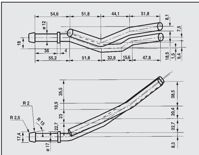
FORD MPV GALAXY 95 ATTACCO COD. AT 261101
