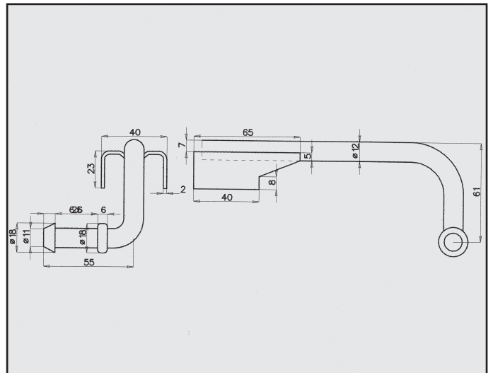
ALFA ROMEO 156 ATTACCO COD. AT 021204
