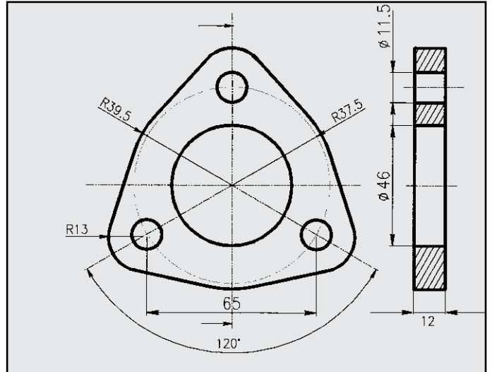
SEAT IBIZA 1.0 FLANGIA COD. FL 680119
