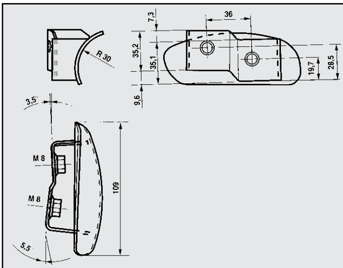
AUDI 100/1994 ATTACCO COD. AT 040105 SX
