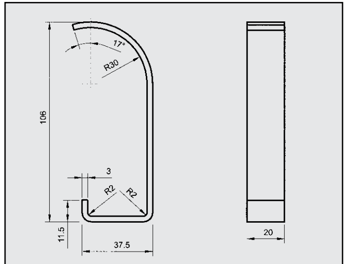
FIAT DAILY ATTACCO COD. AT 241506
