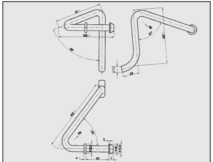
OPEL ATTACCO COD. AT 520023
