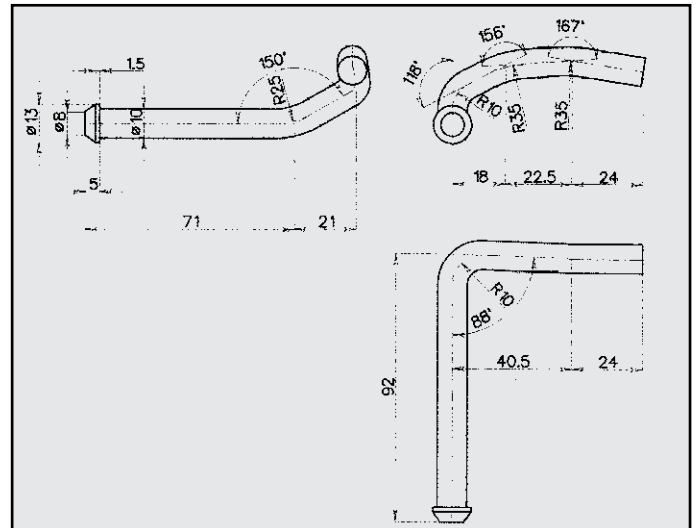
FIAT STILO ATTACCO COD. AT 243502/DX
