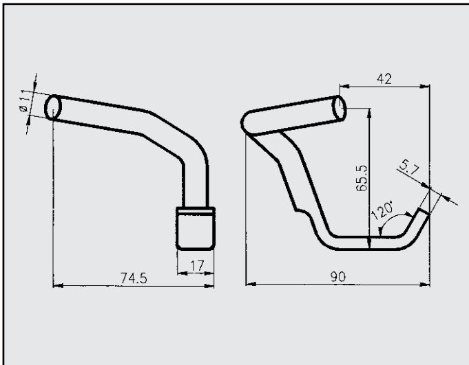
FIAT 600 ATTACCO COD. AT 243102
