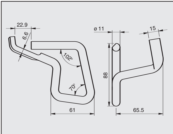
CITROEN XM ATTACCO COD. AT 141101
