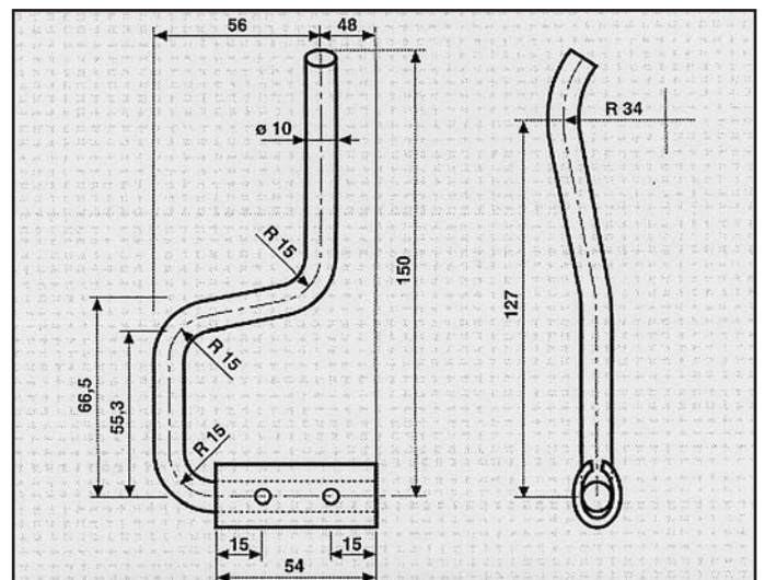
FORD SCORPIO ATTACCO COD. AT 260803
