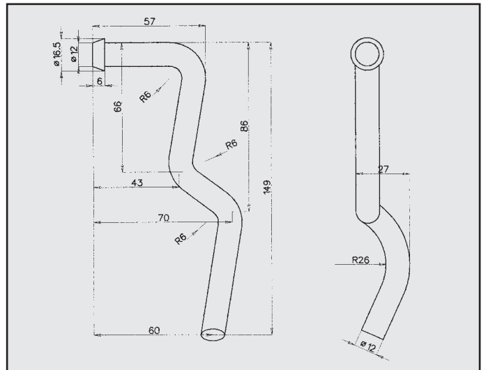
HYUNDAY ATHOS ATTACCO COD. AT 300301
