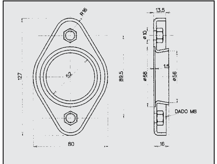
TOYOTA CAMRY 2.0 FLANGIA COD. FL 800110
