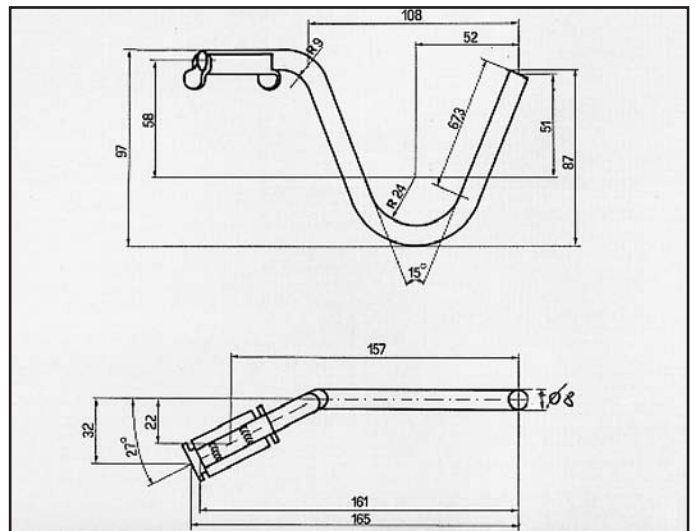
ESCORT 1300/83 ATTACCO posteriore COD. AT 260227
