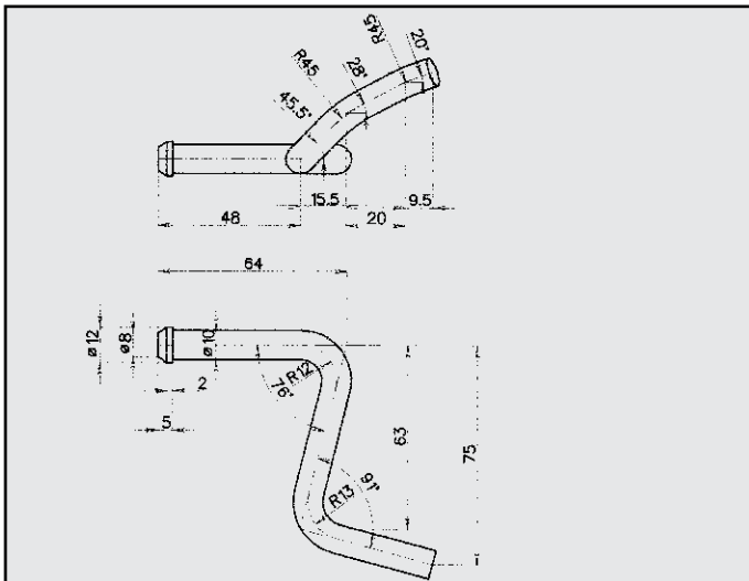
FIAT STILO ATTACCO COD. AT 243501
