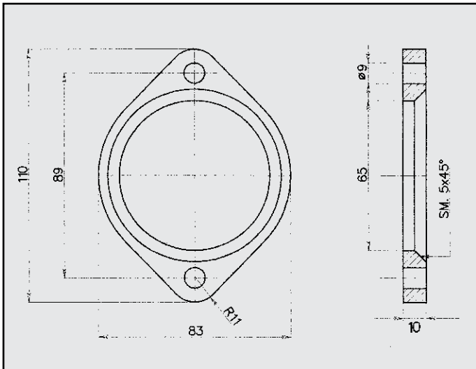
LAND ROVER DISCOVERY FLANGIA COD. FL 350101
