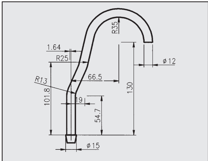
FORD ATTACCO COD. AT 260020
