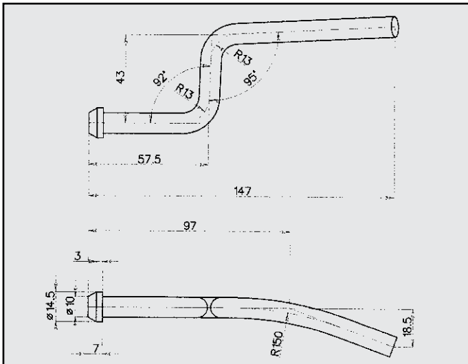
BMW 520 ATTACCO COD. AT 120705
