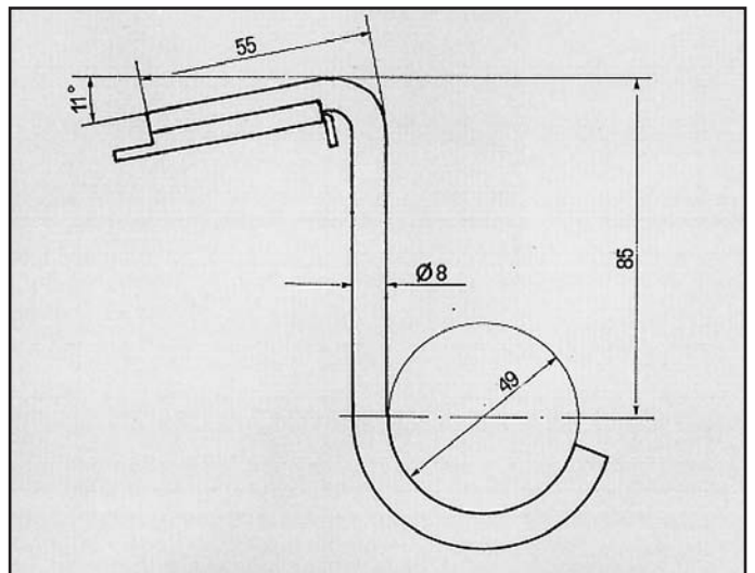
ASCONA ATTACCO posteriore COD. AT 520201/C
