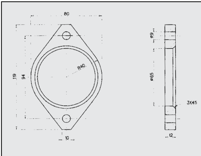
BMW 318 IS 16V FLANGIA COD. FL 120603
