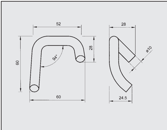
HONDA CIVIC ATTACCO COD. AT 280421
