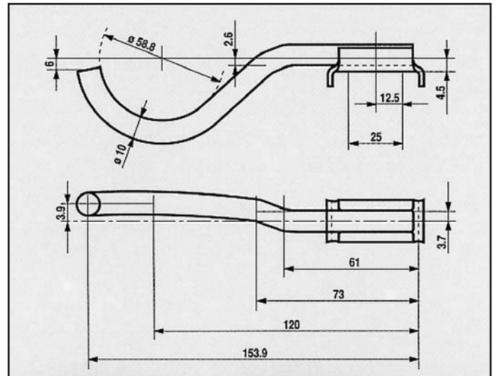
FORD ESCORT 1300 CFI ATTACCO COD. AT 260233
