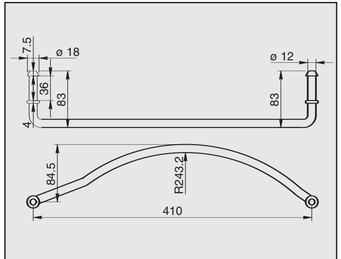
ALFA 156 ATTACCO COD. AT 021203
