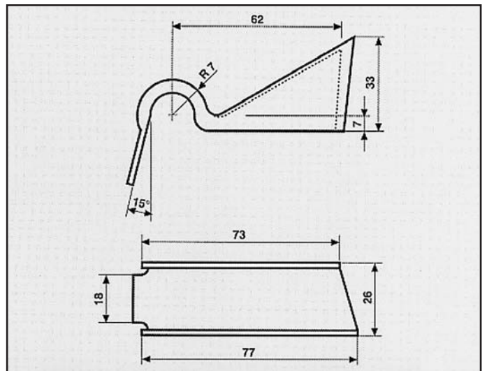
MERCEDES 200 TD S.W. ATTACCO posteriore COD. AT 440207/B
