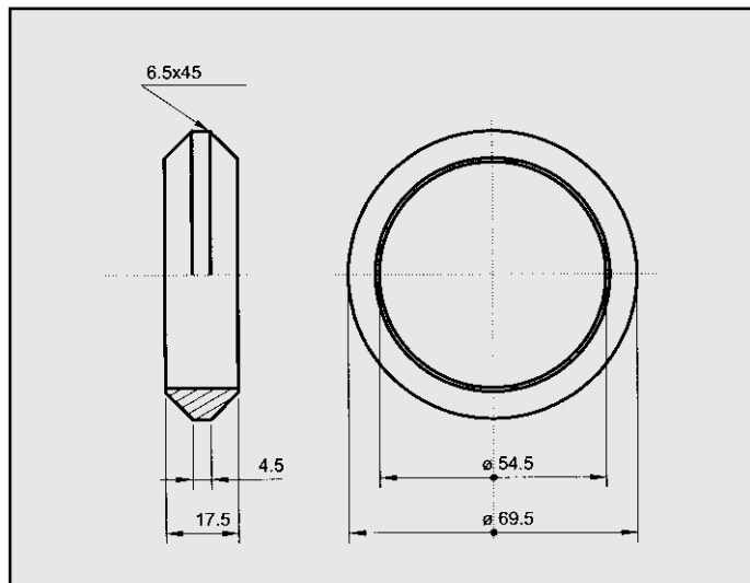
FIAT ULISSE 2.0 ANELLO COD. AN 240007
