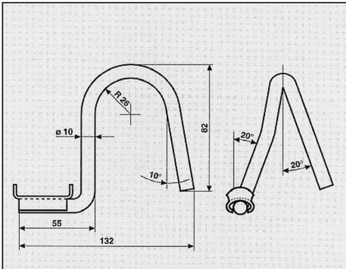
FORD SIERRA 1600 ATTACCO posteriore COD. AT 260618
