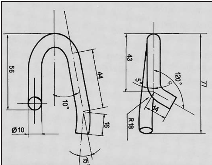
ENGINE TURBO DIESEL ATTACCO COD. AT 540401
