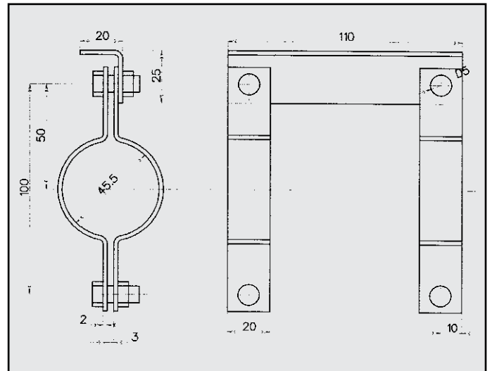
BMW ATTACCO COD. AT 120011
