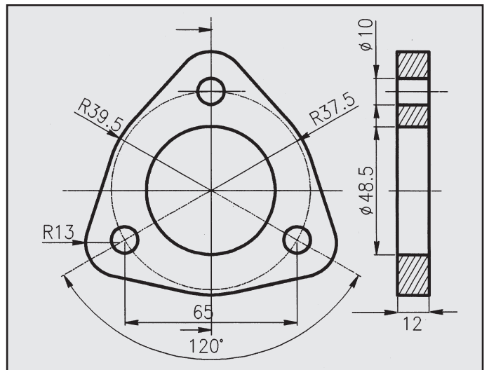
FIAT 500 SPORTING FLANGIA COD. FL 242109
