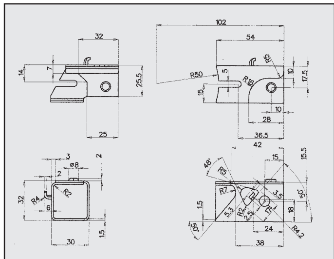
RENAULT ATTACCO COD. AT 600005
