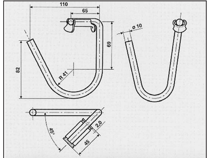
FORD FIESTA/89 ATTACCO posteriore COD. AT 260321
