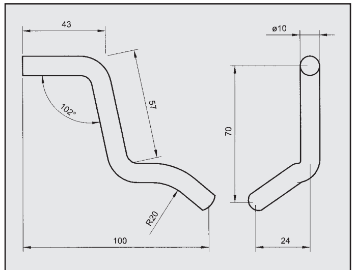
ROVER 214 ATTACCO COD. AT 620602
