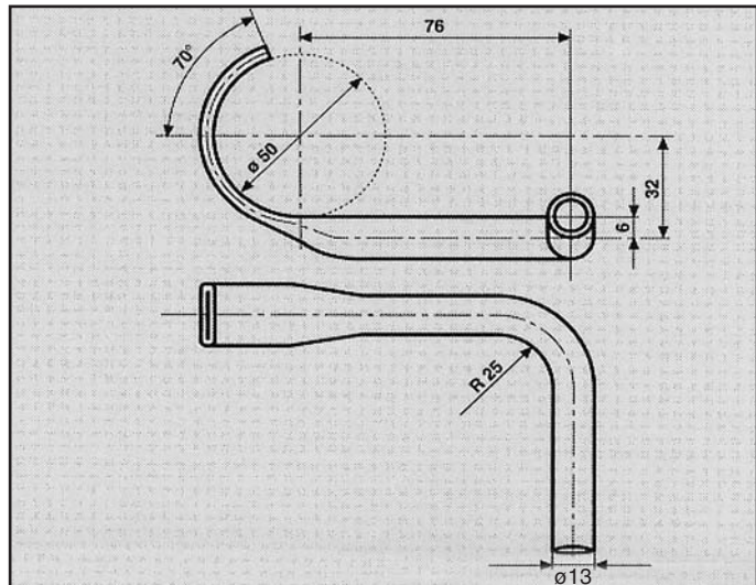
OPEL ATTACCO COD. AT 520005
