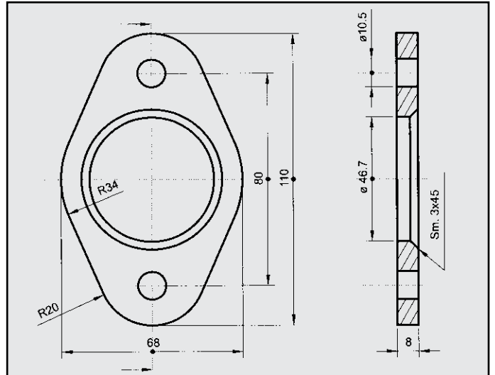
SEAT IBIZA FLANGIA COD. FL 680117
