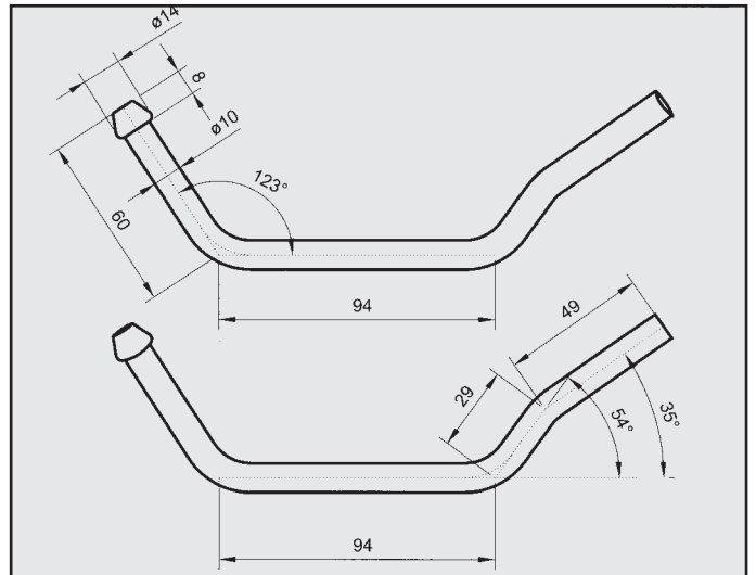
NISSAN PRIMERA 2.0 SLX ATTACCO COD. AT 500404
