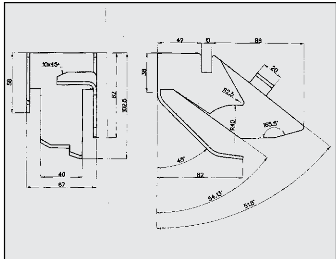
BMW ATTACCO COD. AT 120026
