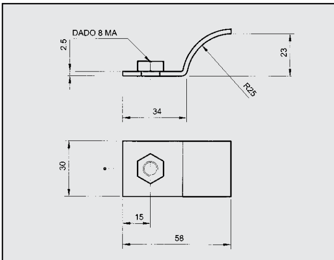
FIAT 128 COUPE' ATTACCO COD. AT 240402
