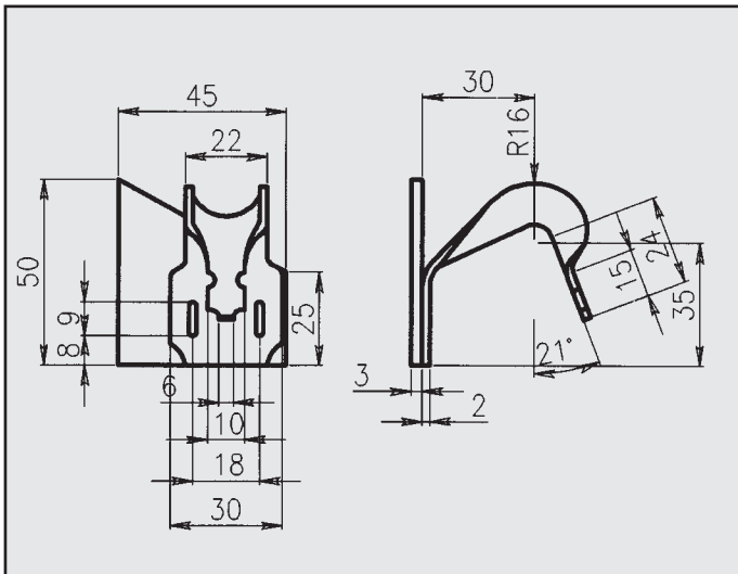
VOLKSWAGEN POLO 1.05 / 1.3 ATTACCO COD. AT 860311
