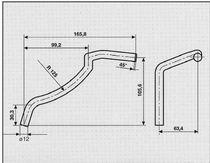
OPEL VECTRA ATTACCO COD. AT 520809
