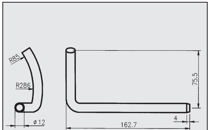
VOLKSWAGEN ATTACCO COD. AT 860011
