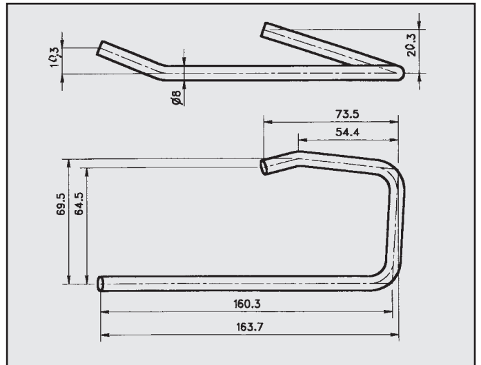
PEUGEOT 106 CAT ATTACCO COD. AT 540803
