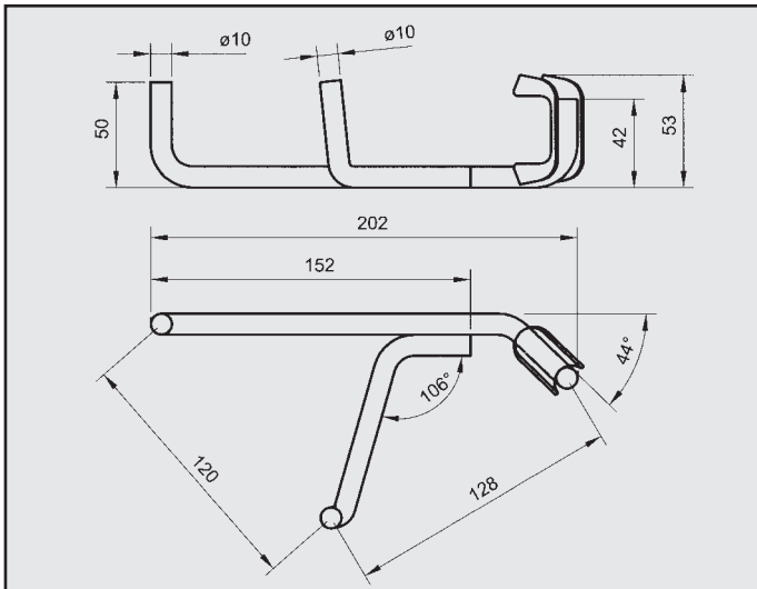
MITSUBISHI SPACE WAGON ATTACCO COD. AT 460302
