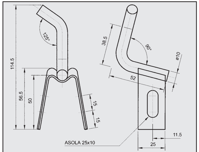
HONDA ATTACCO COD. AT 280419
