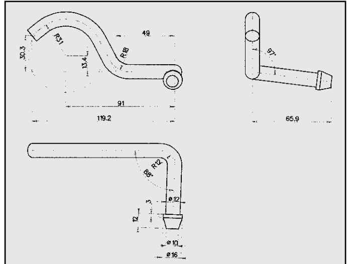
ALFA 147 ATTACCO COD. AT 021507
