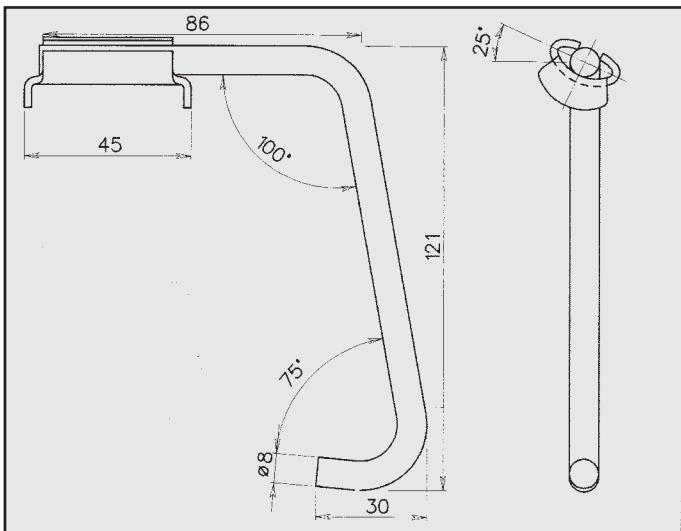
FORD FIESTA ATTACCO COD. AT 260346
