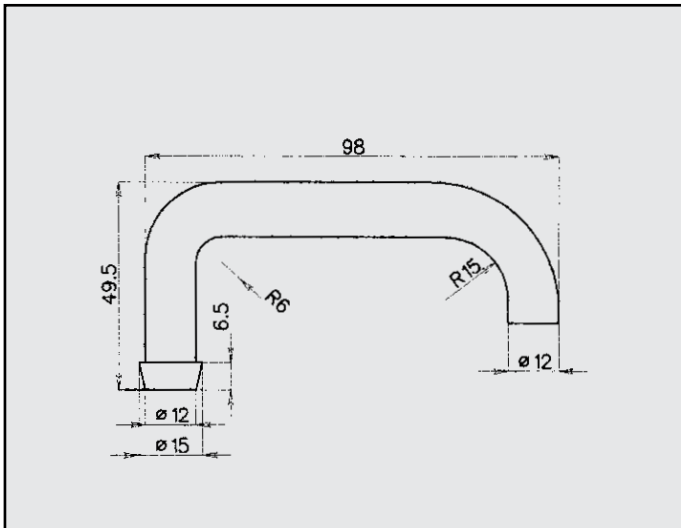
DAEWOO MATIZ ATTACCO COD. AT 160101
