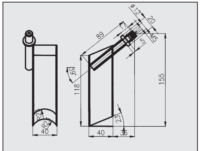
RENAULT CLIO 1.2 KAT 97 ATTACCO COD. AT 601308
