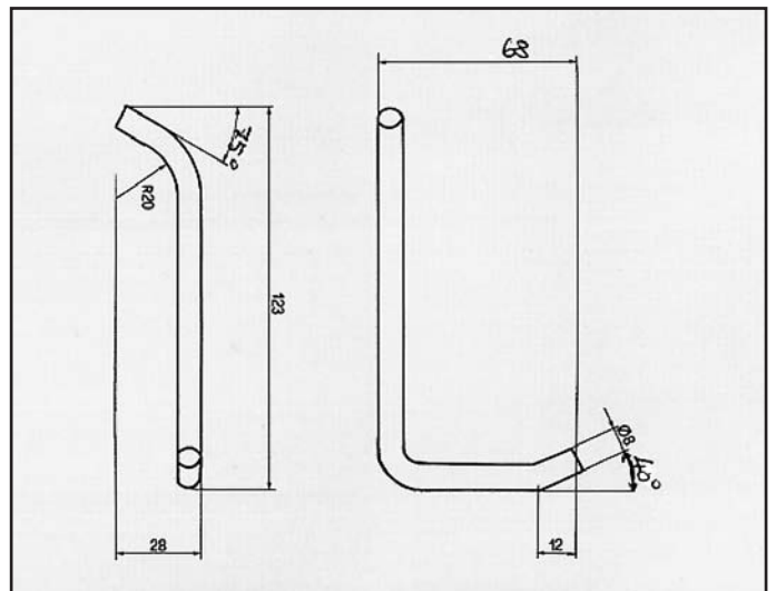
SAMBA 1100 ATTACCO tubo COD. AT 780403
