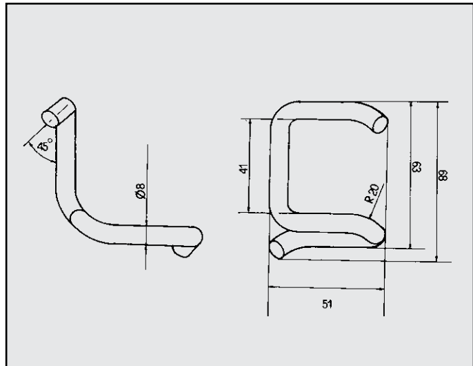
VISA 650 ATTACCO marmitta centrale COD. AT 140103
