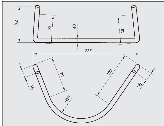
PEUGEOT 205 ATTACCO COD. AT 540318
