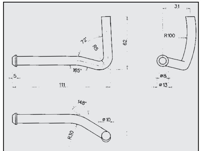
FIAT STILO ATTACCO COD. AT 243504/SX
