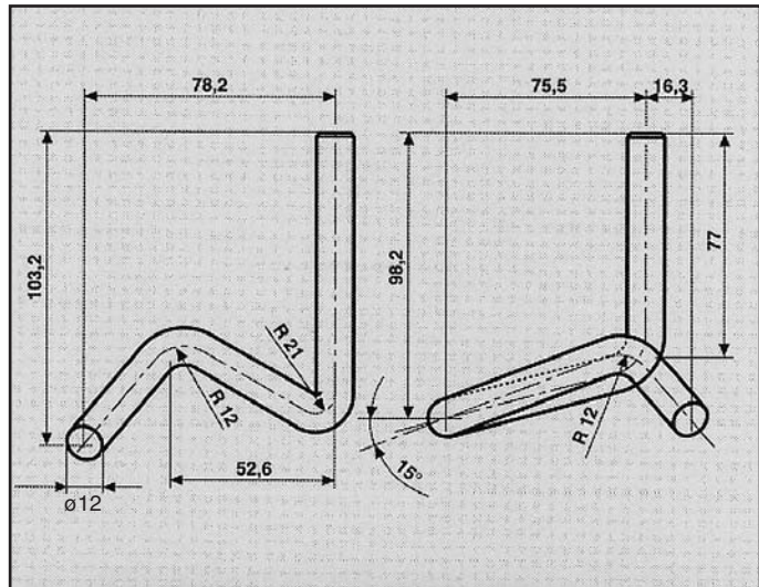
OPEL ATTACCO COD. AT 520006
