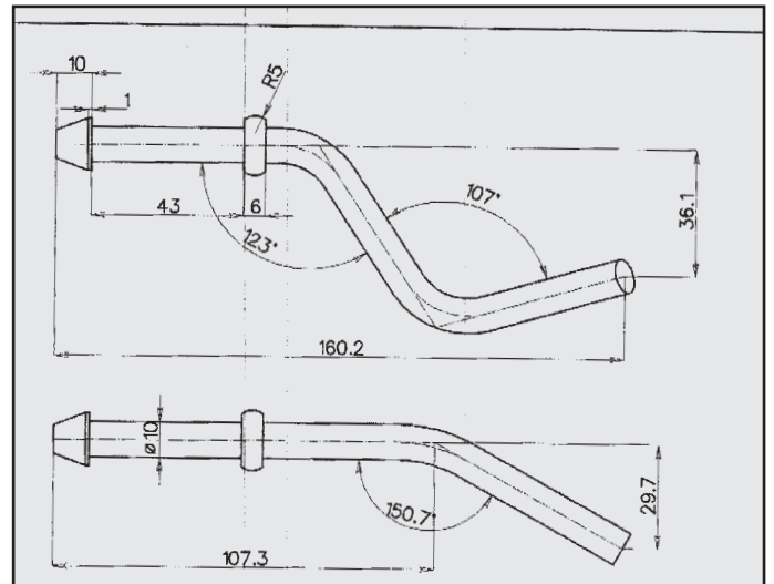
FORD ATTACCO COD. AT 260031
