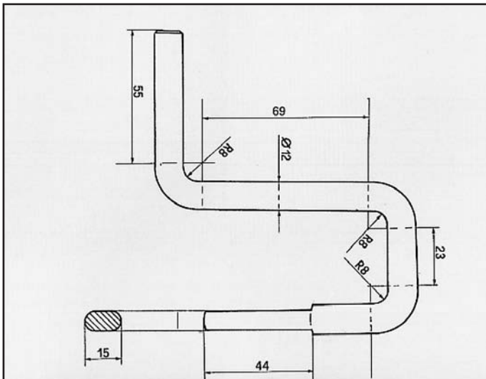
MR II 1600 GT ATTACCO COD. AT 800501
