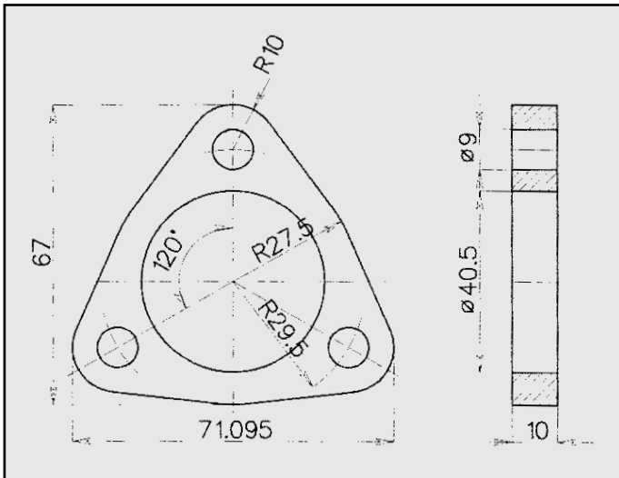
SEAT FLANGIA COD. FL 680007
