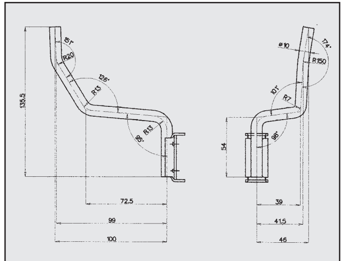
FORD ESCORT ATTACCO COD. AT 260280
