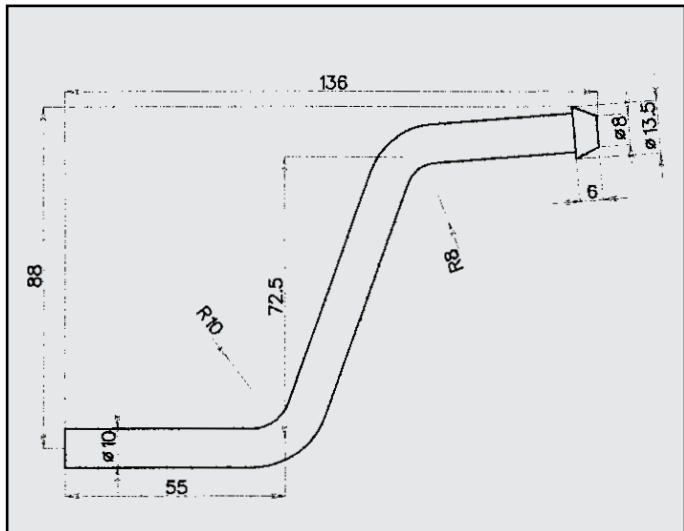
DAEWOO LANOS 2/3V ATTACCO COD. AT 160206
