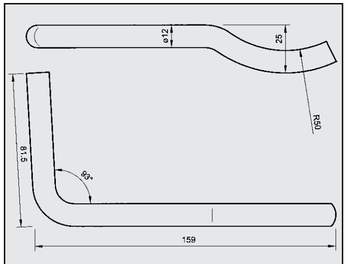
AUDI 80 ATTACCO COD. AT 040314
