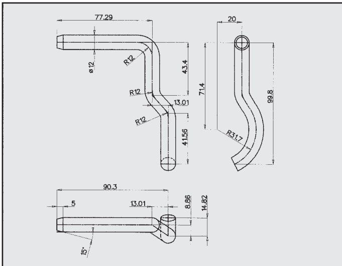
VOLKSWAGEN ATTACCO COD. AT 860032
