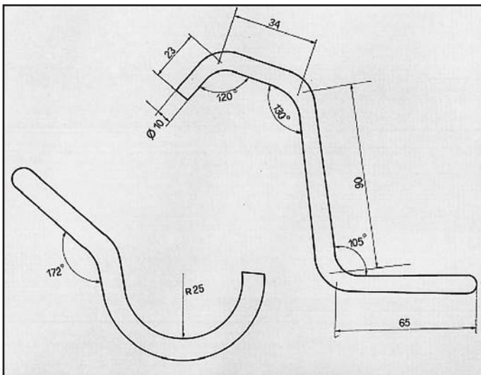
HONDA ACURA LEGEND 86-88 USA ATTACCO COD. AT 280904
