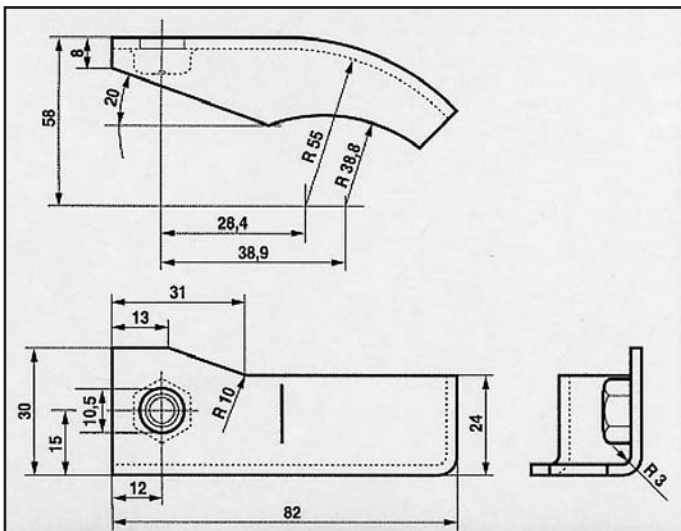
VOLKSWAGEN GOLF/JETTA ATTACCO COD. AT 860901
