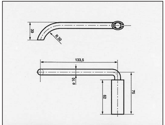
FORD SIERRA 2.0 E ATTACCO COD. AT 260621
