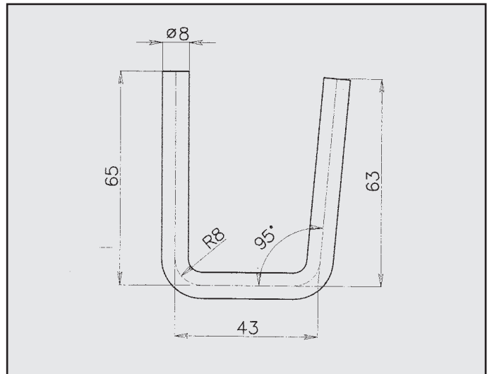
RENAULT LAGUNA 1800 ATTACCO COD. AT 601406/2
