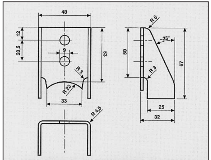
MERCEDES 100D 2.4 ATTACCO COD. AT 440005
