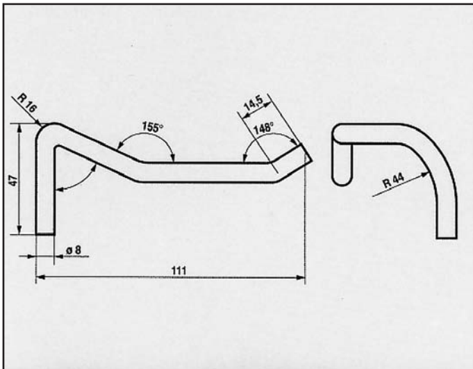
RENAULT R21 2.1 D ATTACCO posteriore COD. AT 601007
