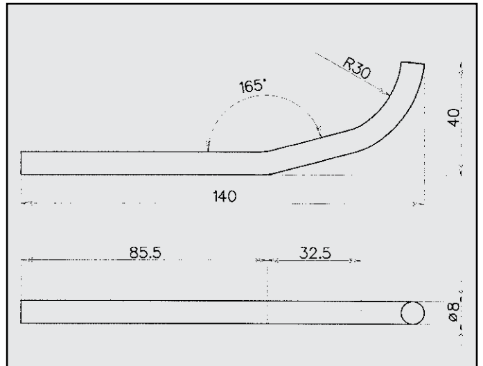
ALFA GTV ATTACCO COD. AT 020611
