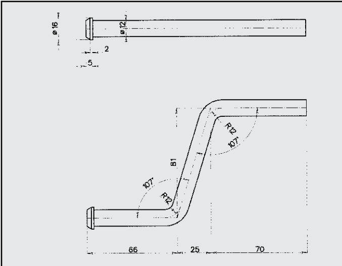
ALFA 147 ATTACCO POSTERIORE DX COD. AT 021504
