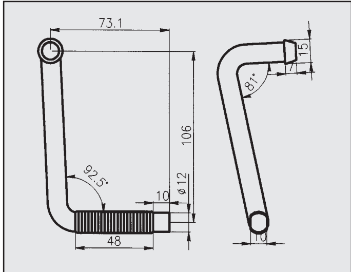
MASERATI ATTACCO COD. AT 400011
