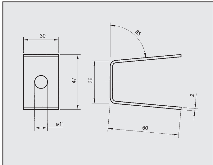
SAAB 900 ATTACCO COD. AT 640208
