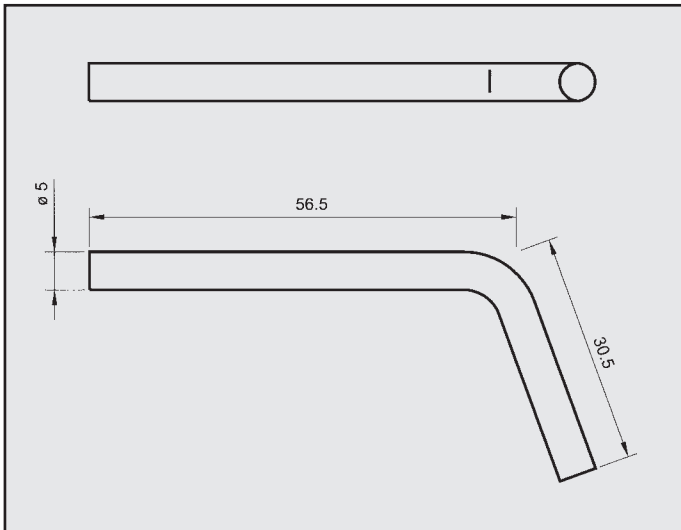
VOLVO 440 "88" ATTACCO COD. AT 880404
