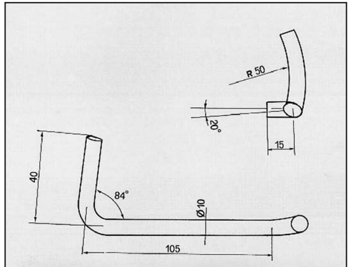
CRX ATTACCO COD. AT 280505
