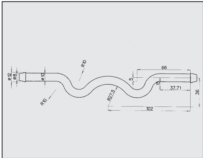
FORD FOCUS TD 1.8 ATTACCO COD. AT 261507
