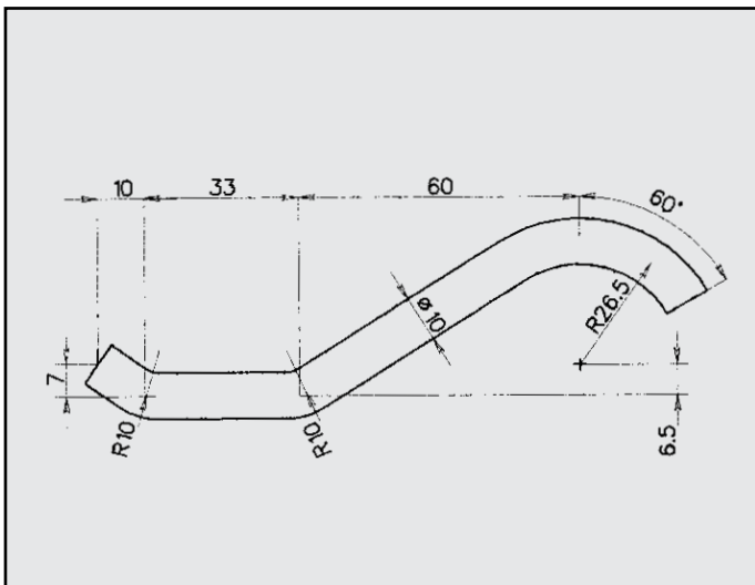
DAIHATSU ATTACCO CENTRALE COD. AT 180009
