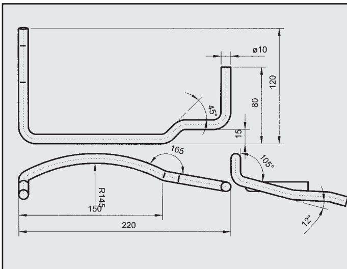
ROVER 416 ATTACCO COD. AT 620702
