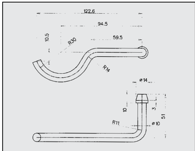
FIAT ATTACCO COD. AT 240014
