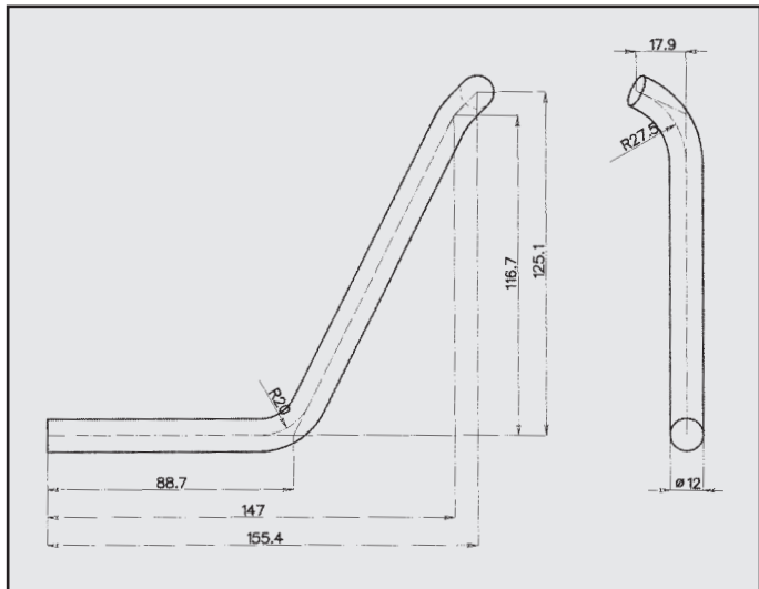
VOLKSWAGEN ATTACCO COD. AT 860036
