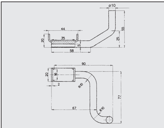
SKODA FELICITA ATTACCO COD. AT 690304
