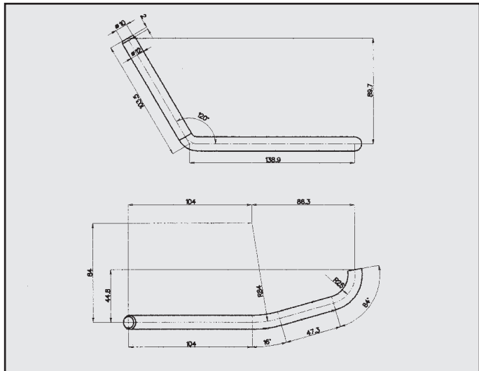
VOLKSWAGEN ATTACCO COD. AT 860035
