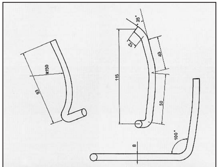
SUPER 5 CAMPUS ATTACCO posteriore COD. AT 600114
