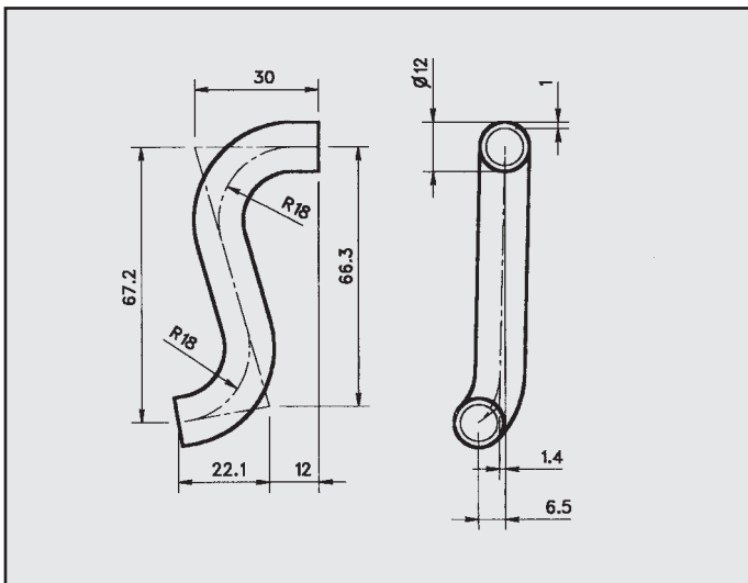
MERCEDES ATTACCO COD. AT 440009
