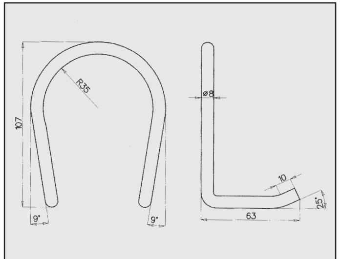
SUPER 5 GT TURBO ATTACCO COD. AT 600107
