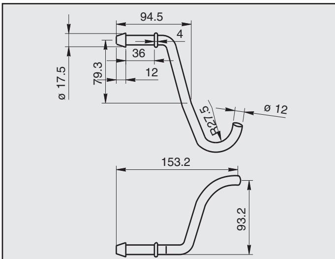
ALFA 156 2.5 i KAT V6 ATTACCO COD. AT 021202
