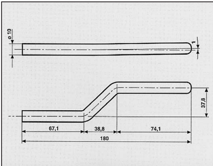
MERCEDES ATTACCO COD. AT 440002
