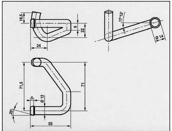
VOLKSWAGEN CORRADO G60 391 ATTACCO COD. AT 860701
