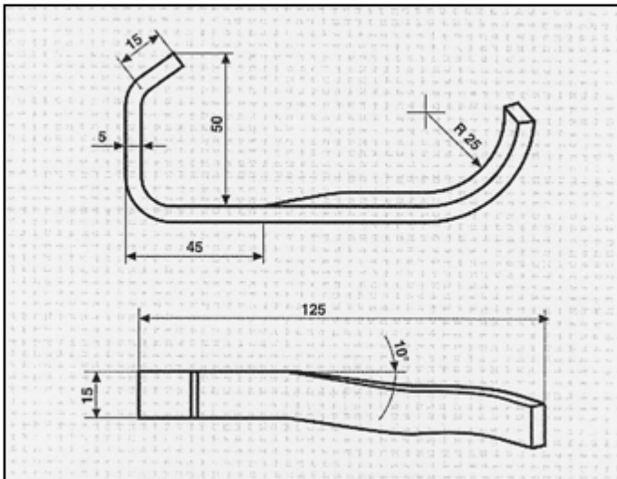
FIAT TEMPRA 1.9 TURBO DIESEL S.W. (1990) ATTACCO posteriore COD. AT 241903
