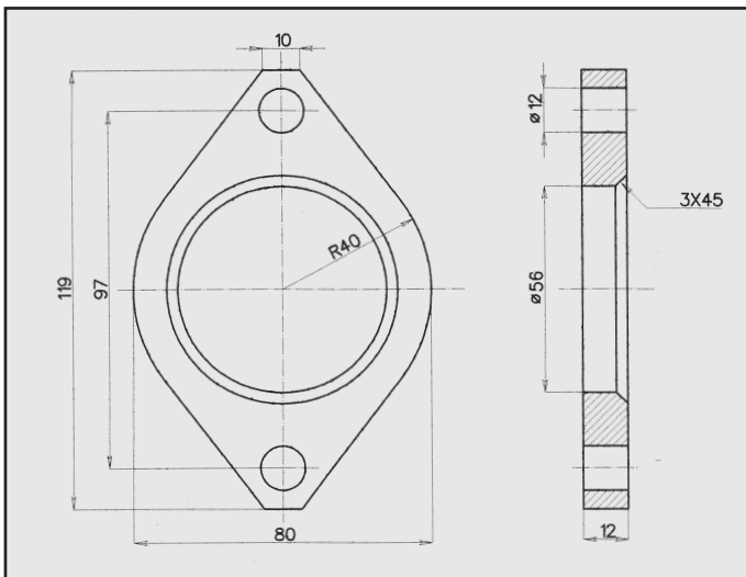
OPEL VECTRA 1.8-2.0 16V FLANGIA COD. FL 520832
