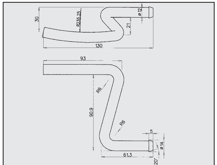
SEAT ATTACCO COD. AT 680006
