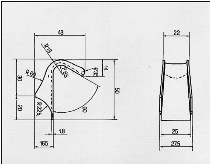
GOLF/DERBY SCIROCCO DIESEL ATTACCO marmitta posteriore COD. AT 860107
