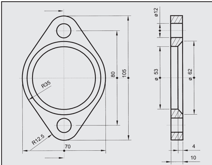
OPEL ASTRA FLANGIA COD. FL 520905
