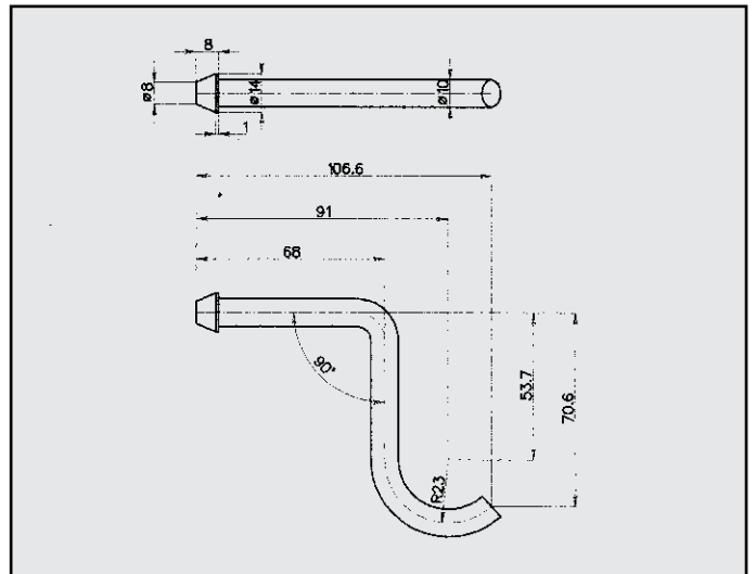
FIAT ATTACCO COD. AT 240019
