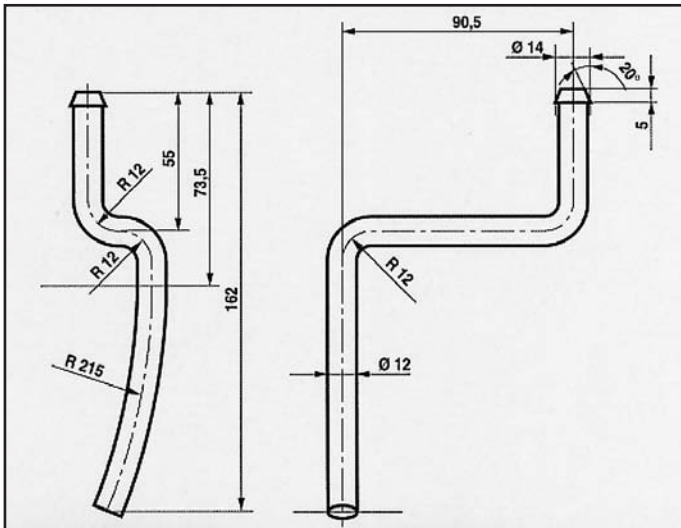
SEAT CORDOBA ATTACCO COD. AT 680605
