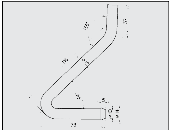
FIAT ULISSE ATTACCO COD. AT 242709
