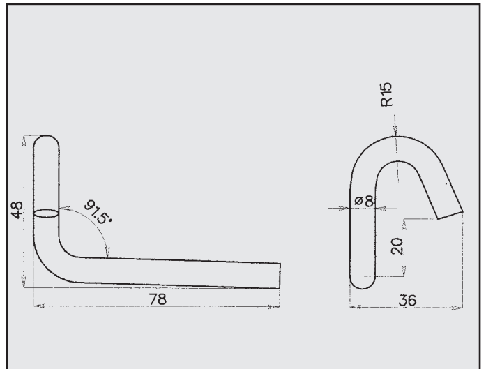
RENAULT MEGANE 1.9-2.0 D ATTACCO COD. AT 601610
