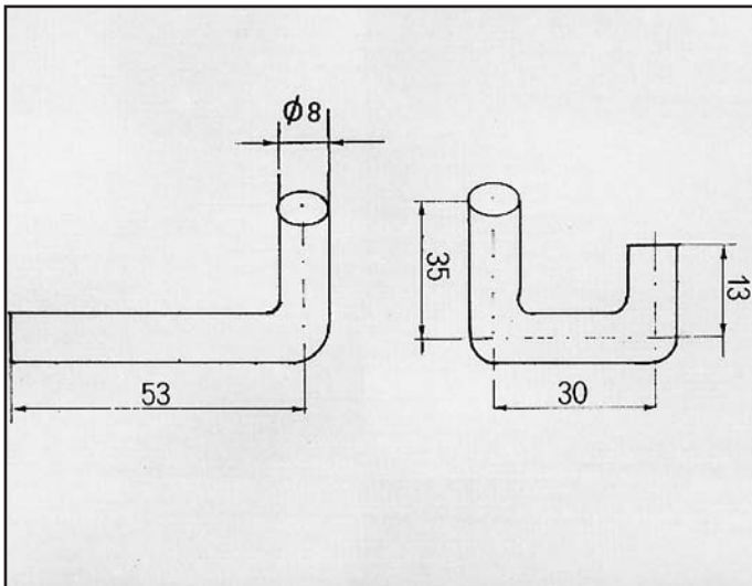
99 COUPÉ ATTACCO COD. AT 640101
