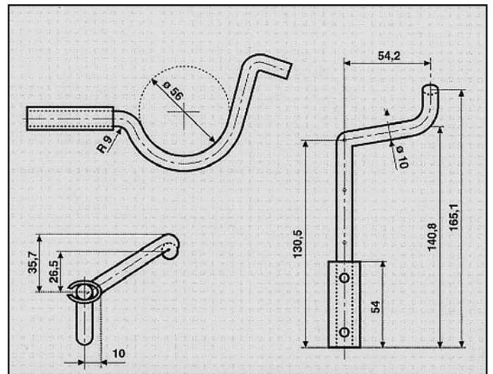
OPEL ATTACCO COD. AT 520012
