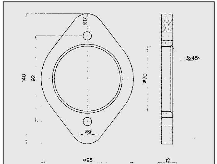
OPEL OMEGA FLANGIA COD. FL 520620
