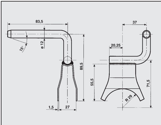
VOLKSWAGEN ATTACCO COD. AT 860001
