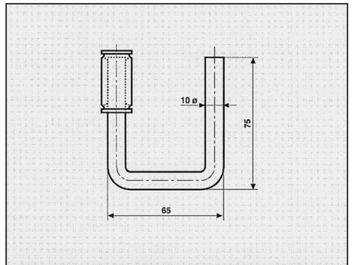
FORD SIERRA 18 CVH ATTACCO centrale COD. AT 260617
