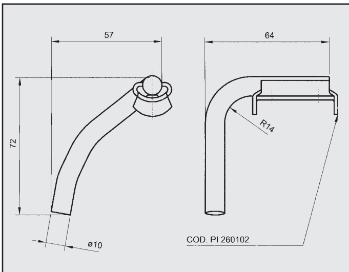
VOLVO 340 ATTACCO COD. AT 880107
