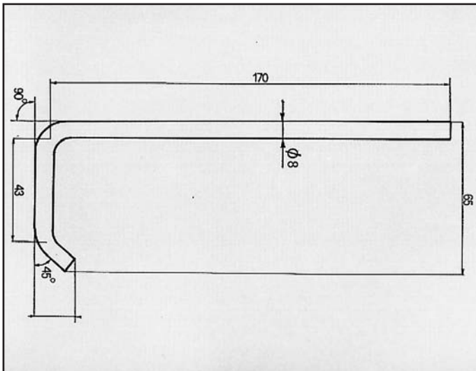
ACTY ATTACCO COD. AT 280201
