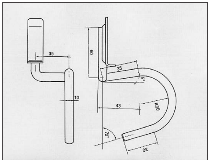
KADETT GSI ATTACCO COD. AT 520107
