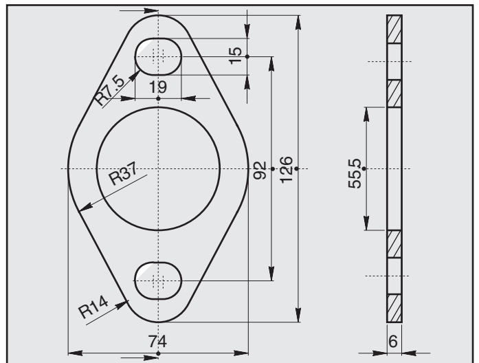
OPEL VECTRA 2.0 FLANGIA COD. FL 520826
