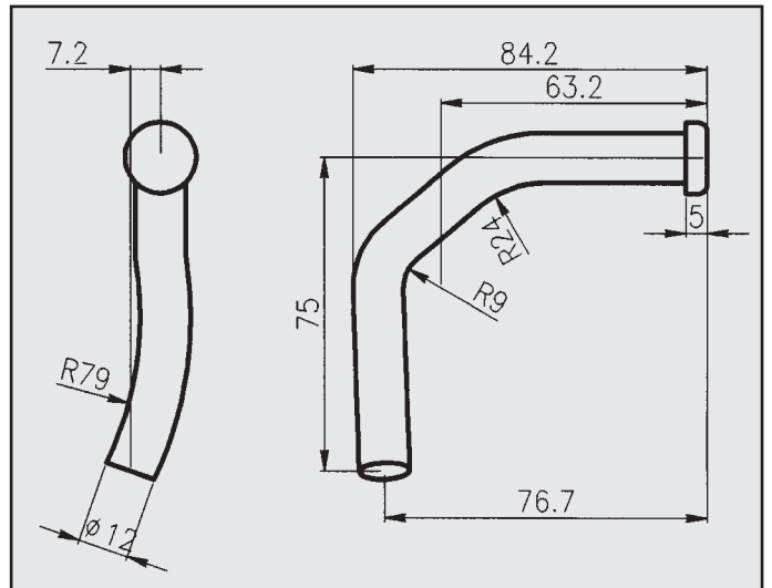
OPEL OMEGA ATTACCO COD. AT 520615
