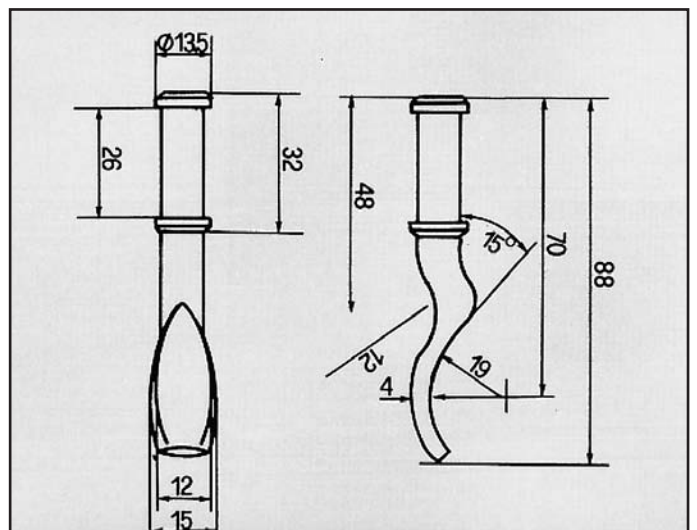
GLC 1500 ATTACCO COD. AT 420303
