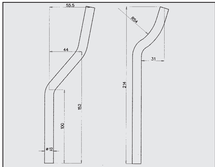
OPEL ASTRA ATTACCO COD. AT 520927
