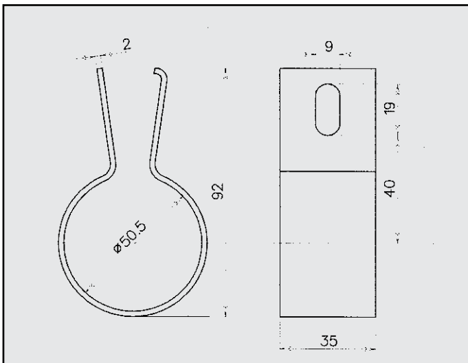
FORD FASCETTA COD. F 260016
