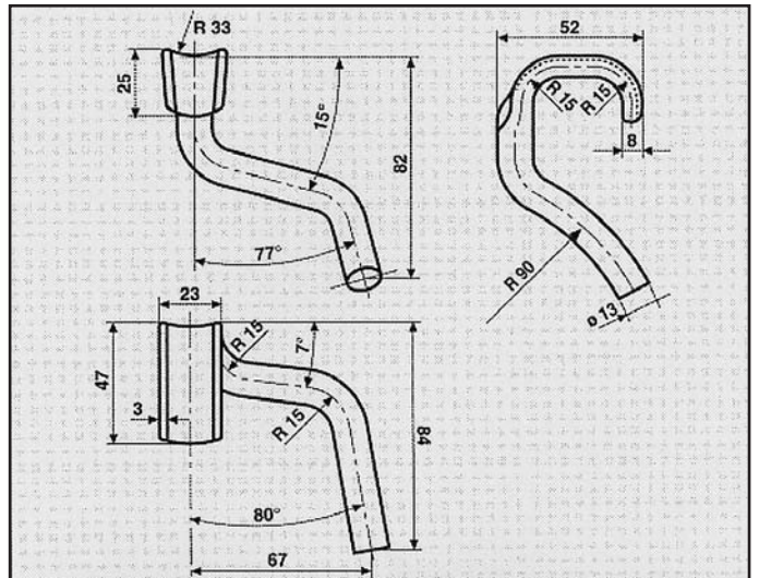
OPEL SENATOR ATTACCO COD. AT 520502
