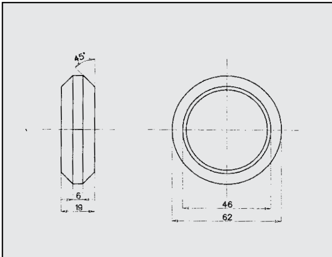
FIAT SCUDO 1.6/1.9D ANELLO COD. AN 243203
