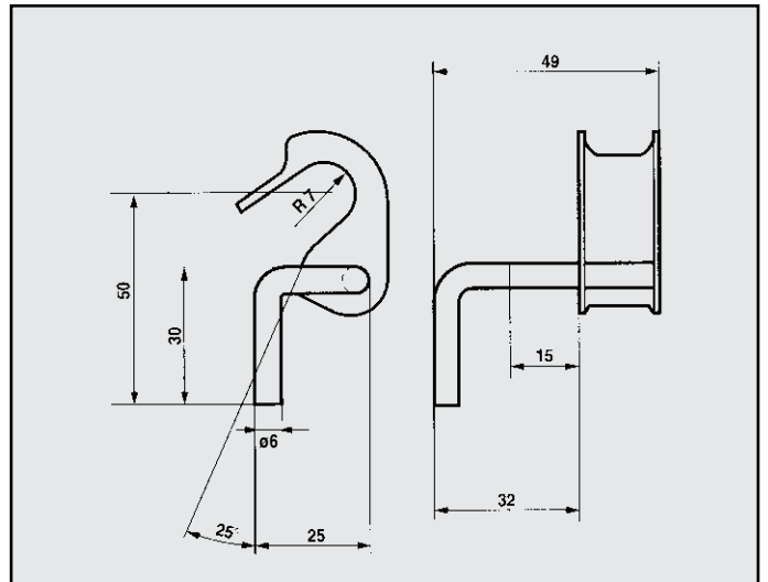
ALFA 75/2.0 TWIN SPARK ATTACCO per posteriore SX COD. AT 020308/SX
