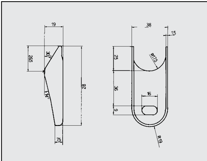
AUDI 80 ATTACCO marmitta anteriore COD. AT 040301 055253209F
