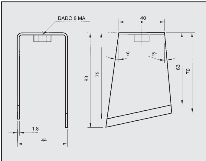
MITSUBISHI PAJERO 2.3 - 2.5 TD ATTACCO COD. AT 460202
