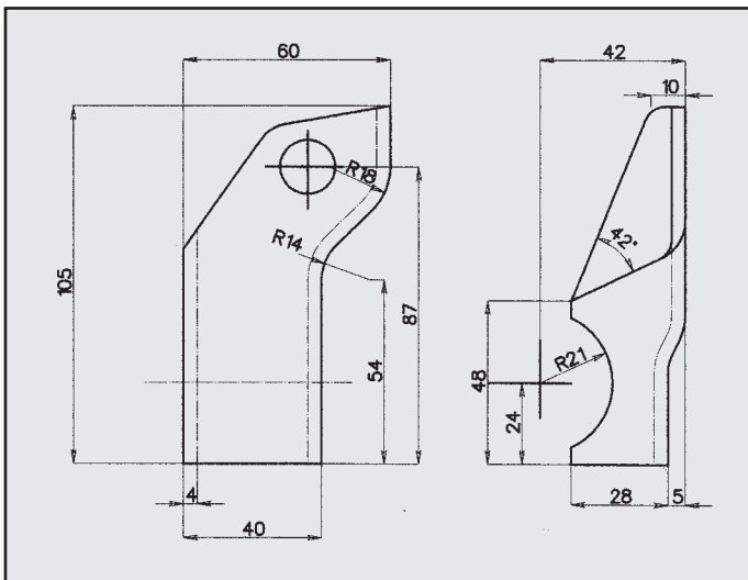
PEUGEOT 206 ATTACCO COD. AT 541210
