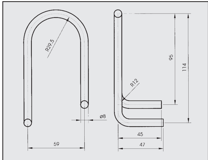
RENAULT ATTACCO COD. AT 600004
