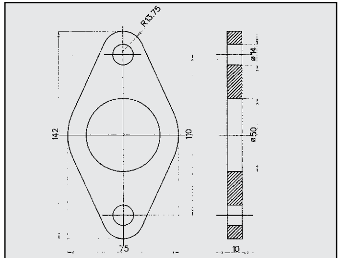
MAZDA 1.8 16V FLANGIA COD. FL 420002
