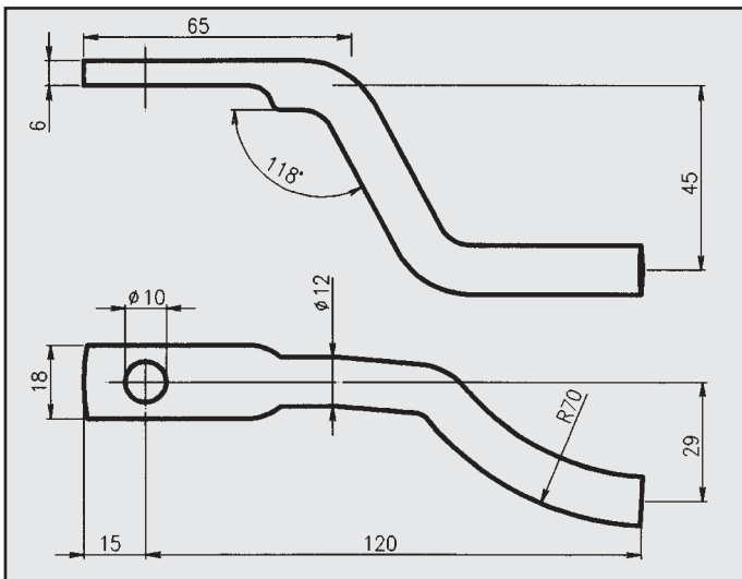
MITSUBISHI PAJERO '86 ATTACCO COD. AT 460209
