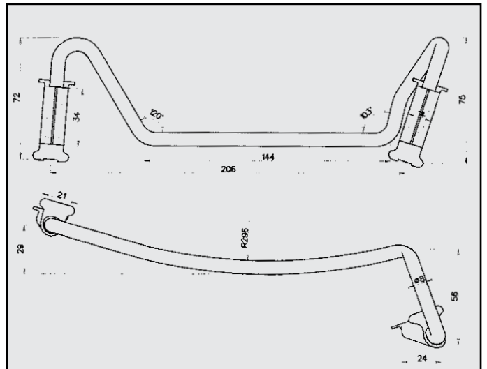
FIAT ULISSE 1.8 ATTACCO COD. AT 242710
