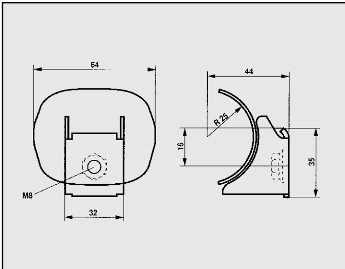
AUDI 100 C4 / DIESEL ATTACCO COD. AT 040103
