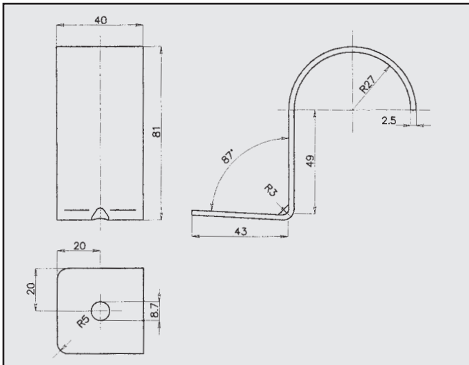
RENAULT 25 ATTACCO COD. AT 601503
