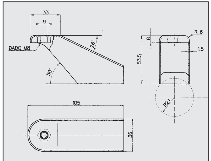
MITSUBISHI LANCER ATTACCO COD. AT 460401
