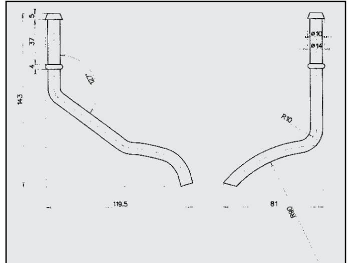
BMW ATTACCO COD. AT 120606
