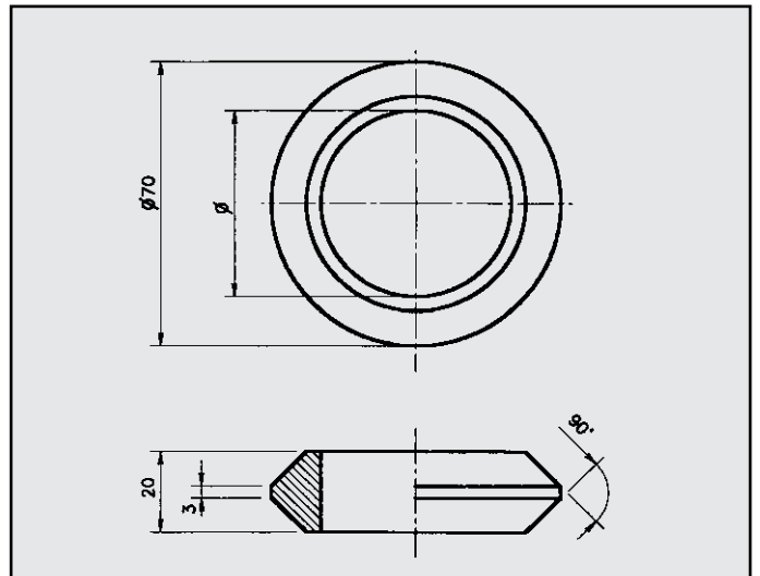
PEUGEOT 205 - 309 ANELLO \varnothing esterno mm 70 \varnothing interno mm 41 - 46 - 51 COD. AN 540302
