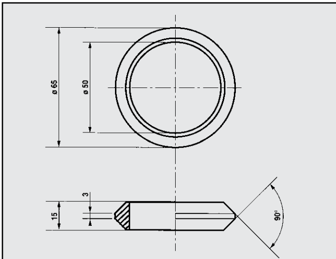
RENAULT 21 NEVADA ANELLO \varnothing esterno mm 65 \varnothing interno mm 50 COD. AN 601008
