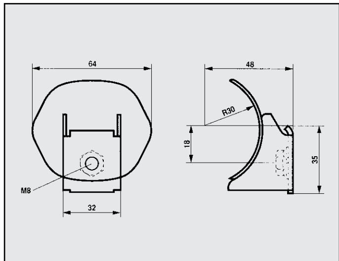
AUDI 100 C4 / TURBO DIESEL ATTACCO COD. AT 040102
