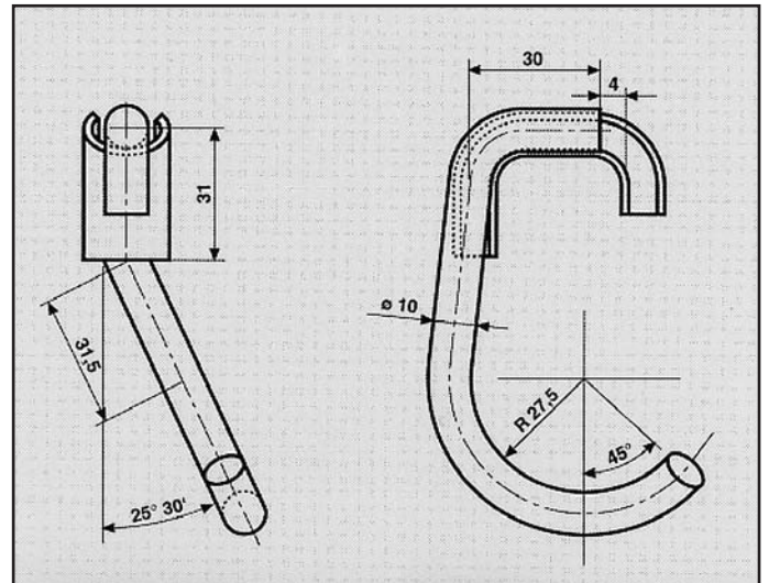
OPEL ATTACCO posteriore COD. AT 520010
