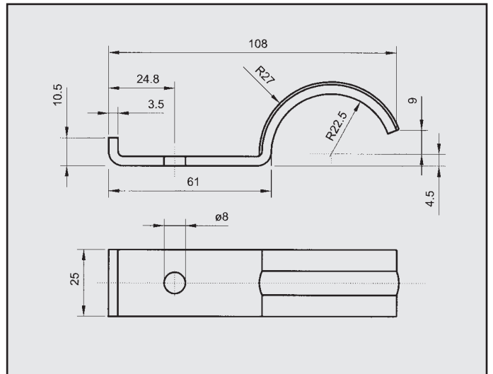
RENAULT 25 TD ATTACCO COD. AT 600605
