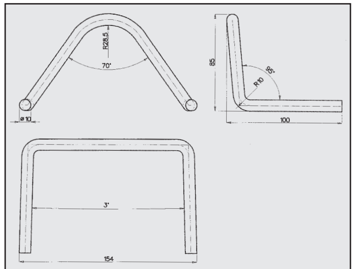
VOLKSWAGEN POLO ATTACCO COD. AT 860315
