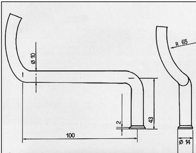
626 2000 16V ATTACCO anteriore dx COD. AT 420512
