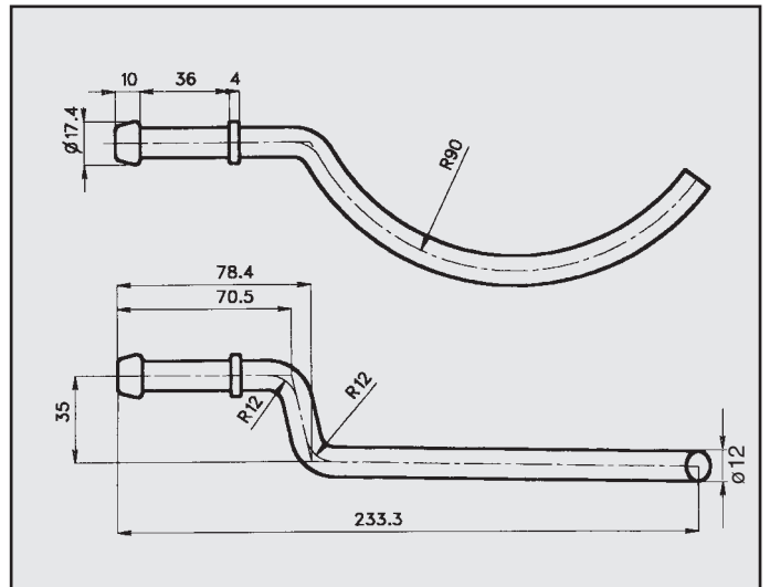
VOLKSWAGEN SHARAN 96 ATTACCO COD. AT 861201
