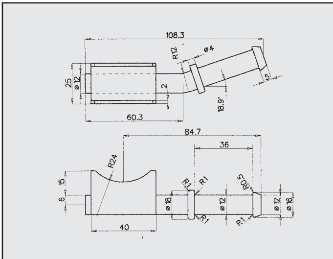
SEAT AROSA ATTACCO COD. AT 680805
