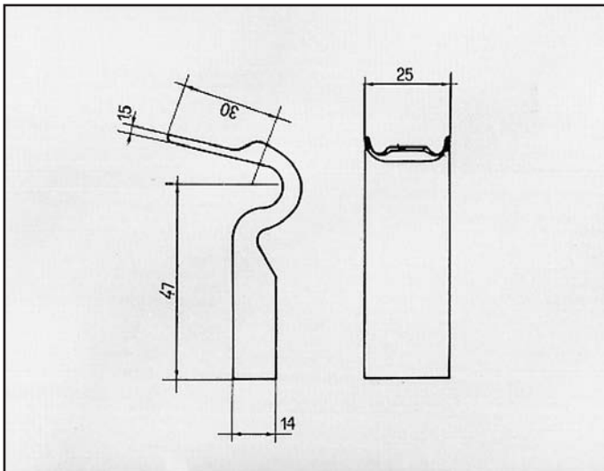
SAMARA 1300-1400-1600 ATTACCO COD. AT 360102
