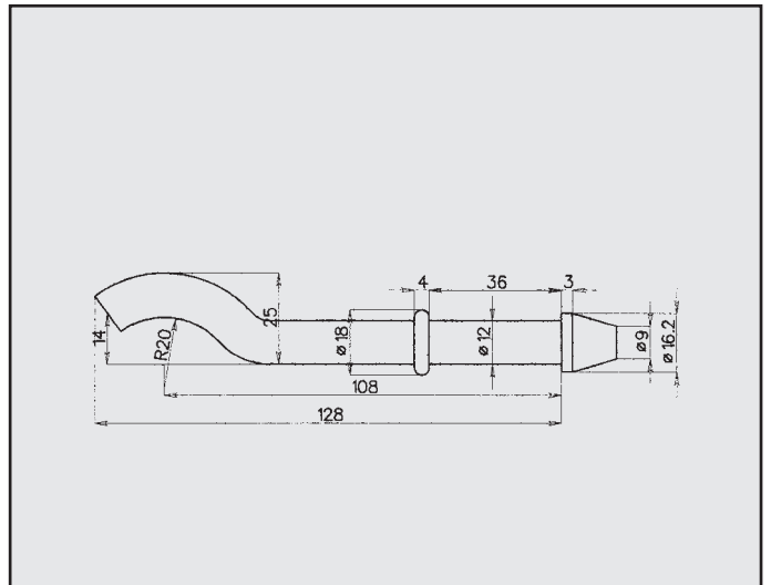
SEAT AROSA ATTACCO COD. AT 680801
