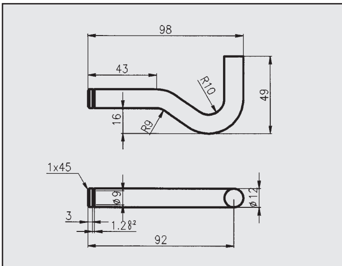
OPEL CORSA B 1.0 1.2 ATTACCO COD. AT 520316
