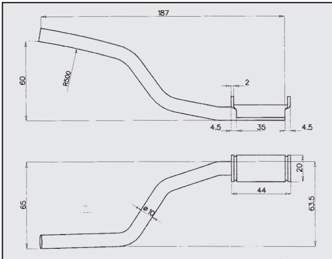
FORD SIERRA ATTACCO COD. AT 260625
