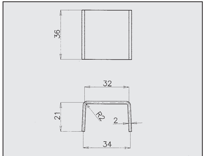
MERCEDES ATTACCO COD. AT 440015
