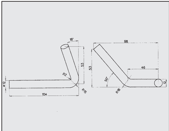
SEAT AROSA / VOLKSWAGEN LUPO ATTACCO COD. AT 680809
