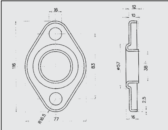
TOYOTA YARIS FLANGIA COD. FL 801204
