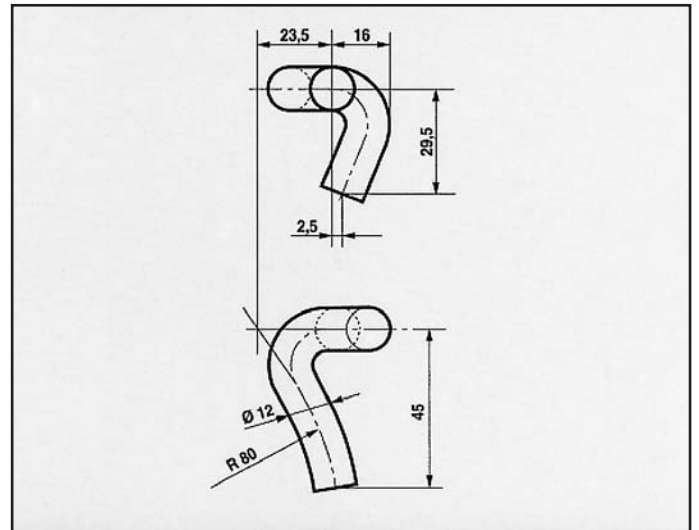
VOLKSWAGEN SYNCRO VR6 ATTACCO COD. AT 860803
