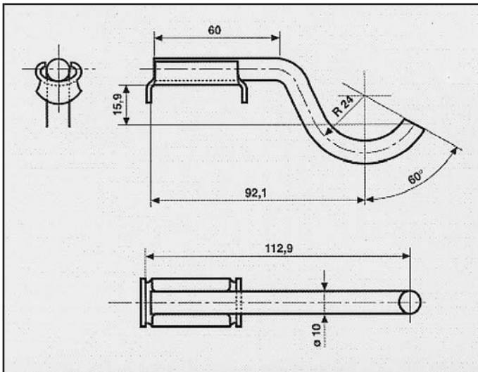
FORD ESCORT ATTACCO COD. AT 260241
