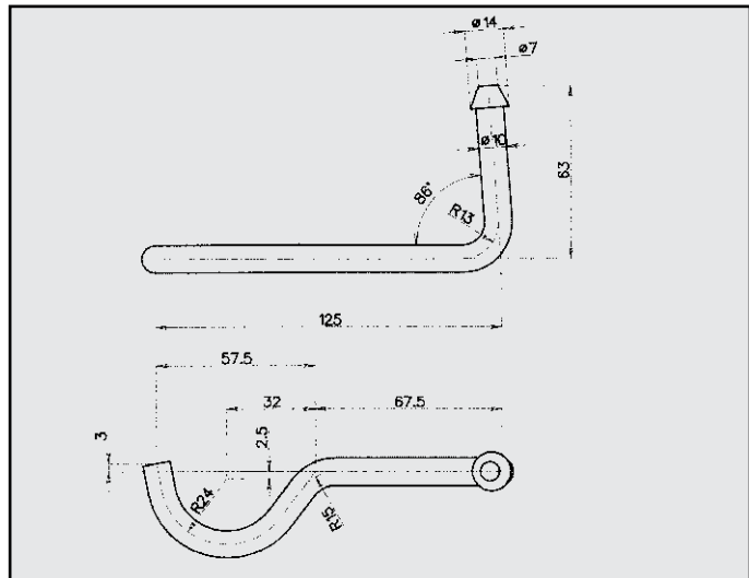
FIAT DOBLO' 1.2 ATTACCO COD. AT 243404
