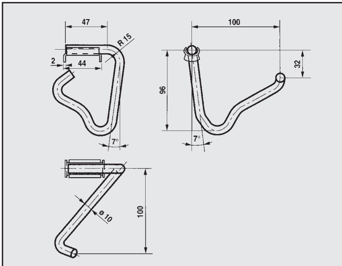
FORD FIESTA 1.3 CAT '89 ATTACCO COD. AT 260329
