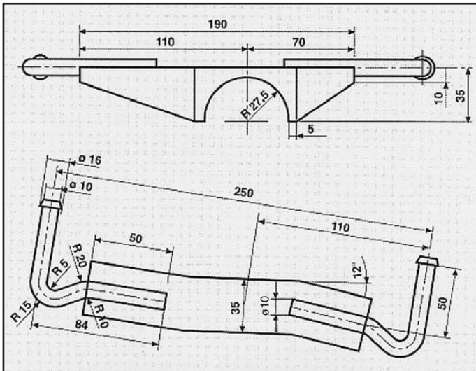
MAZDA ATTACCO COD. AT 420001
