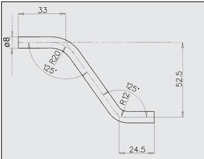
MOTO GUZZI GRISO 571 ATTACCO COD. AT 270201
