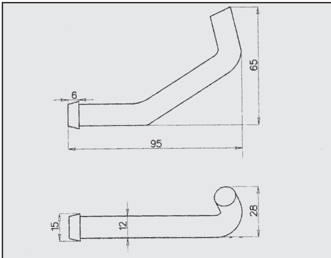
VOLVO S40-V40 ATTACCO COD. AT 880901
