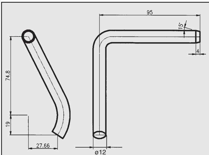
VOLKSWAGEN ATTACCO COD. AT 860009
