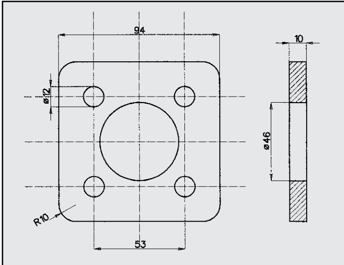
HYUNDAI PONY FLANGIA COD. FL 300106
