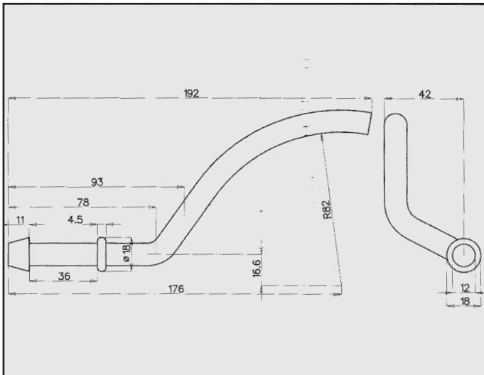
FORD GALAXY ATTACCO COD. AT 261106
