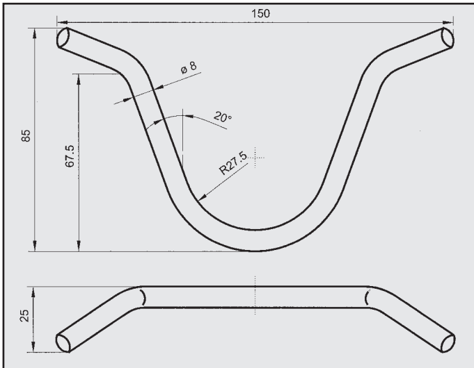
MERCEDES 200 200E ATTACCO COD. AT 440208
