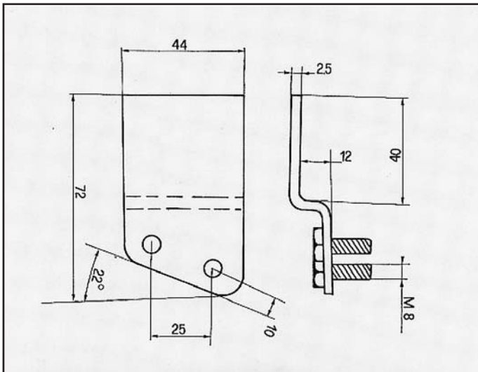
504 GLT BERLINA ATTACCO marmitta anteriore COD. AT 540501
