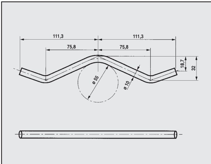
FORD SCORPIO 1995 ATTACCO COD. AT 260812
