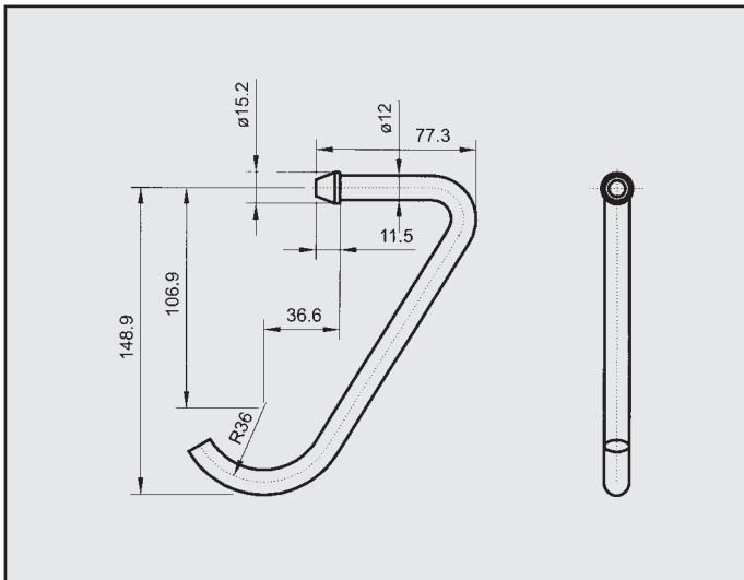
FORD TRANSIT DIESEL '84 ATTACCO COD. AT 261007
