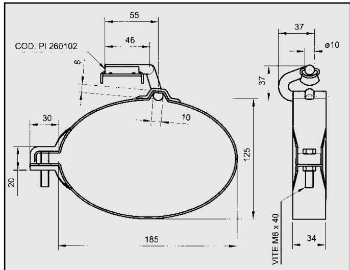
OPEL KADET FASCETTA COD. F 520112
