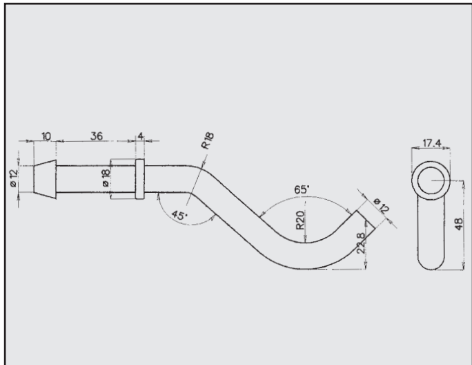
SEAT AROSA / VOLKSWAGEN LUPO ATTACCO COD. AT 680807
