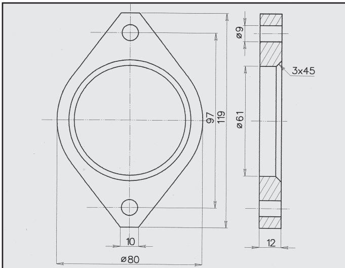
OPEL VECTRA 1.6i KAT FLANGIA COD. FL 520819
