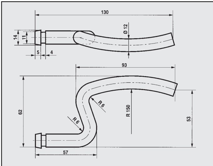
SEAT IBIZA 1.3 R 93 ATTACCO COD. AT 680109
