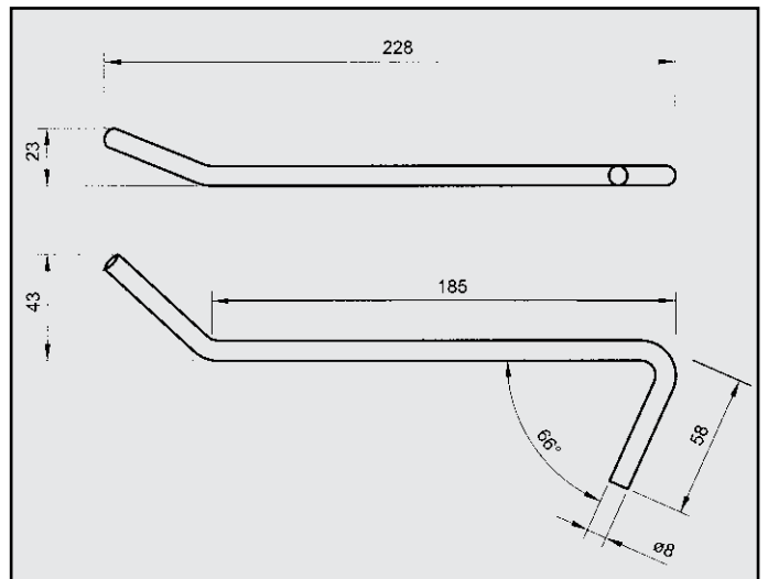
ALFA ROMEO ATTACCO COD. AT 020310
