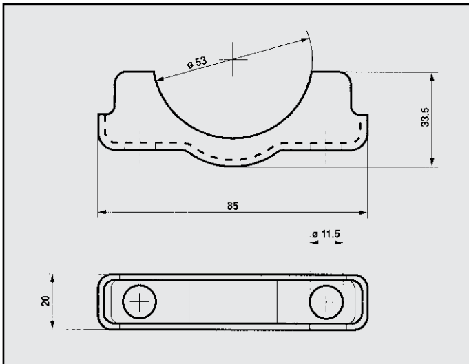
FORD FASCETTA A CAVALLOTO \varnothing 53 COD. F 260002
