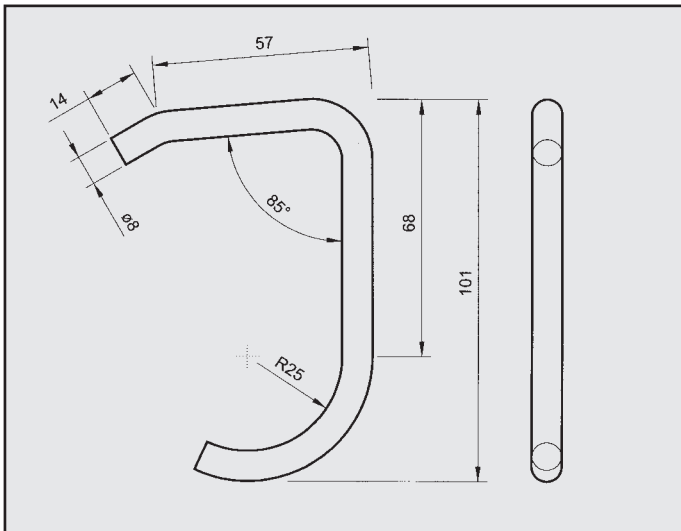
RENAULT R9 ATTACCO COD. AT 600204
