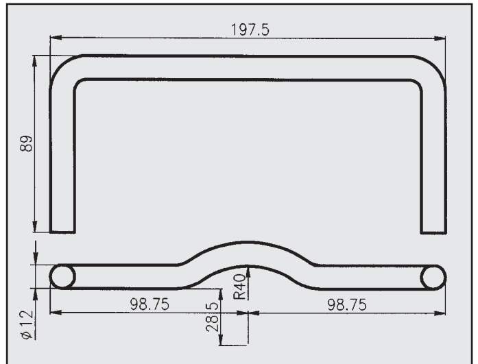
OPEL VECTRA 95 2.0 16V ATTACCO centrale COD. AT 520817
