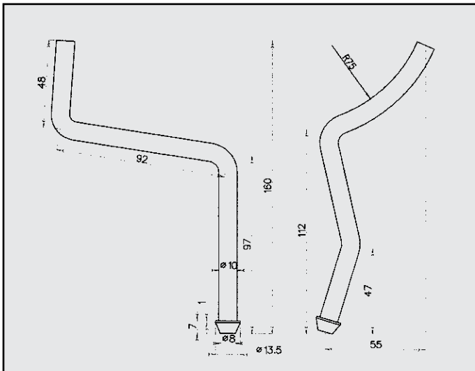
FIAT PALIO 1.2 - 1.6 ATTACCO POSTERIORE COD. AT 243001
