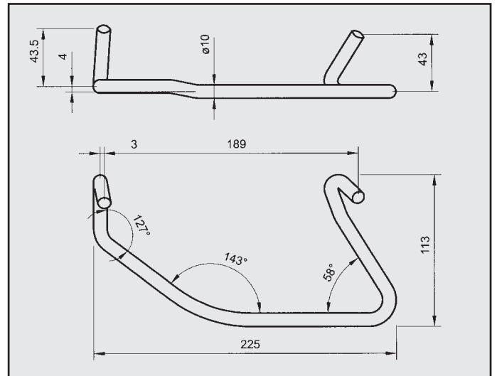
FORD ESCORT ATTACCO COD. AT 260261
