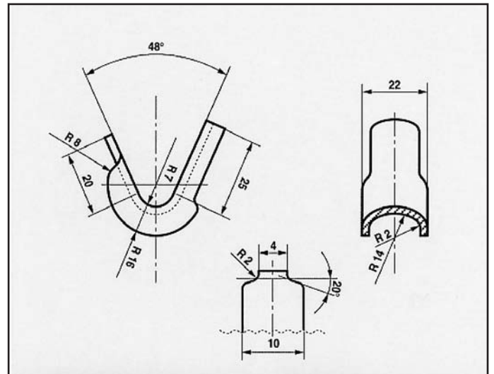
VOLKSWAGEN SYNCRO VR6 ATTACCO COD. AT 860804
