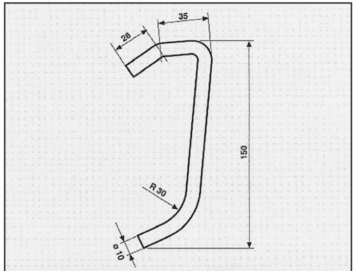
ROVER STERLING ATTACCO COD. AT 620201
