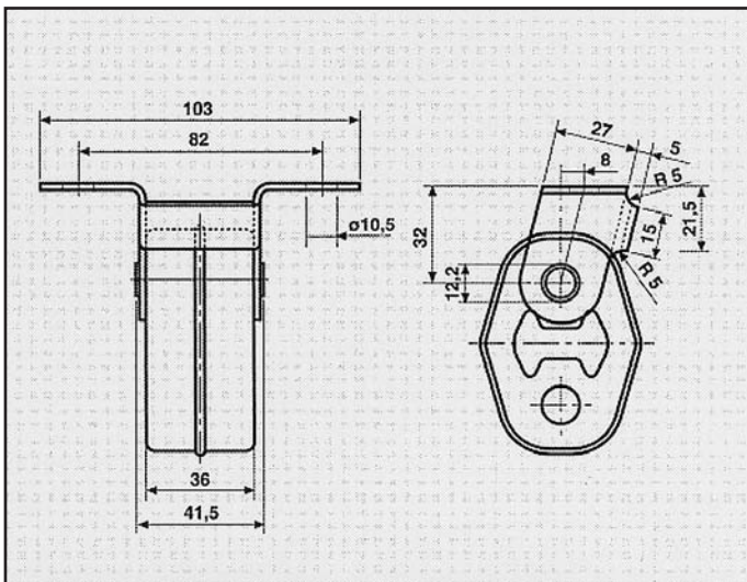
SEAT ATTACCO COD. AT 680003
