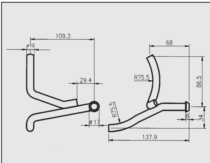
VOLKSWAGEN PASSAT ATTACCO COD. AT 860209
