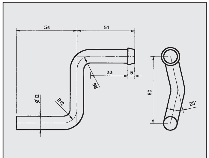
SUZUKI SWIFT ATTACCO COD. AT 720202
