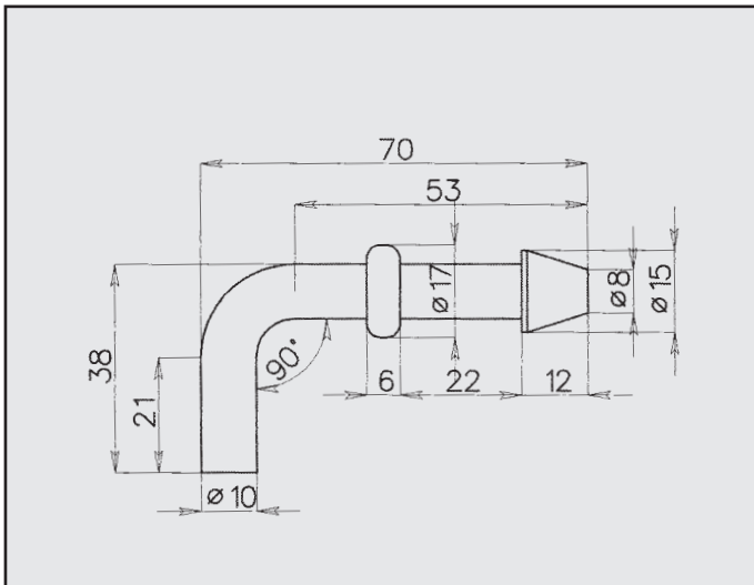
FORD ATTACCO COD. AT 260023
