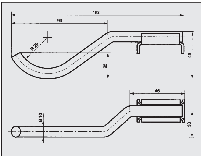
FORD ESCORT/ORION ATTACCO COD. AT 260242
