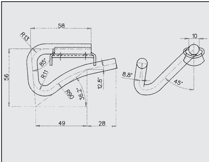
FORD FIESTA ATTACCO COD. AT 260360
