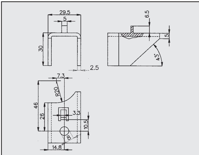
RENAULT CLIO ATTACCO COD. AT 601310
