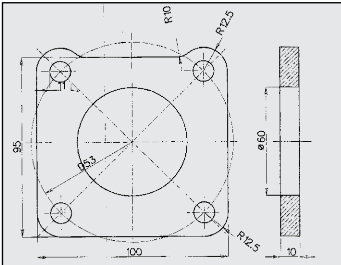
VOLKSWAGEN GOLF FLANGIA COD. FL 860126
