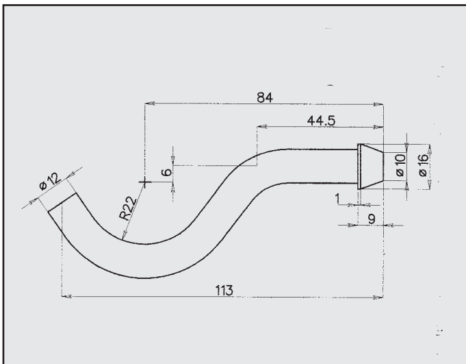
OPEL ATTACCO COD. AT 521201
