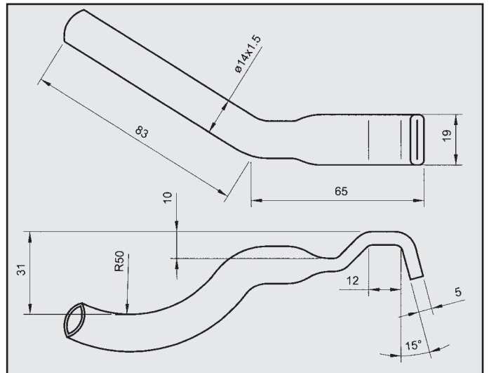
SAAB 900 ATTACCO COD. AT 640202 / AN
