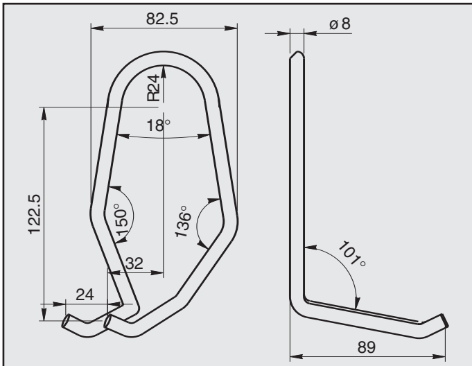
ALFA 145 / 146 ATTACCO COD. AT 021106
