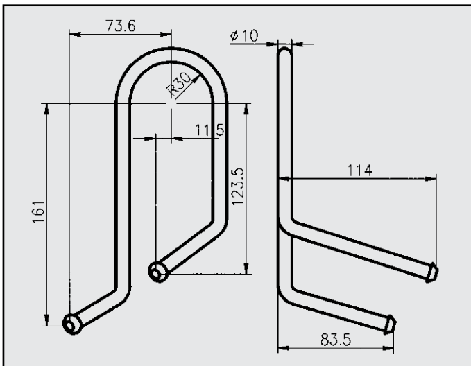
FIAT MAREA TD ATTACCO COD. AT 242810
