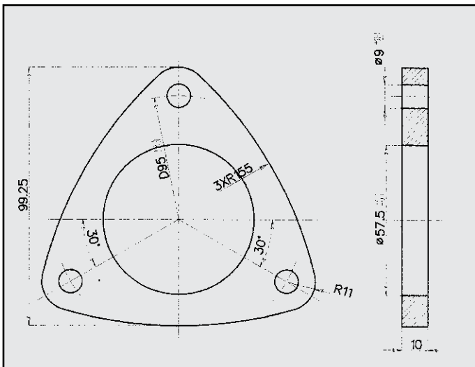
ALFA ROMEO 145/146/155 FLANGIA COD. FL 021107
