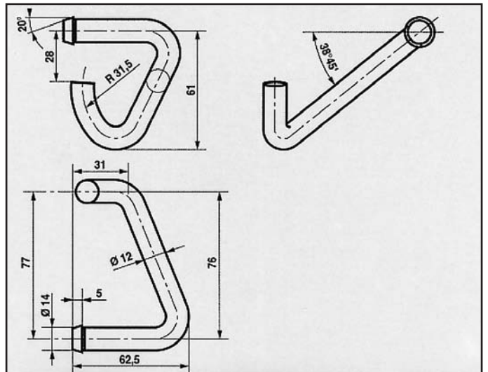
VOLKSWAGEN CORRADO G60 91 ATTACCO COD. AT 860702
