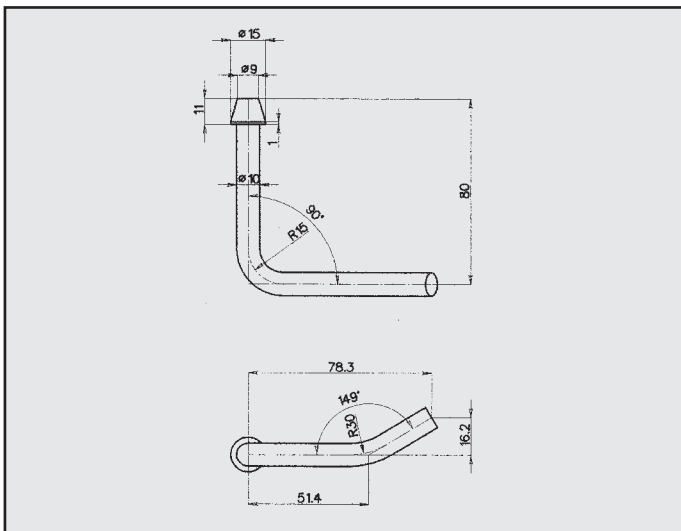
TOYOTA ATTACCO COD. AT 800009
