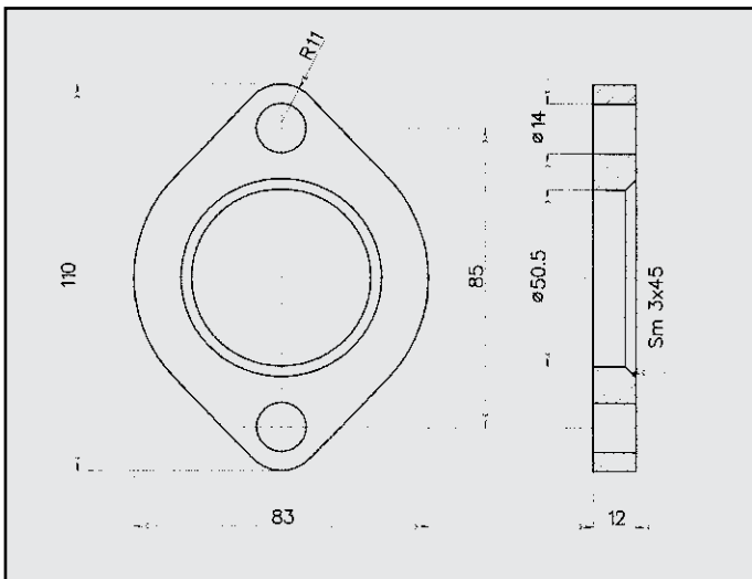
HYUNDAI PONY FLANGIA COD. FL 300107
