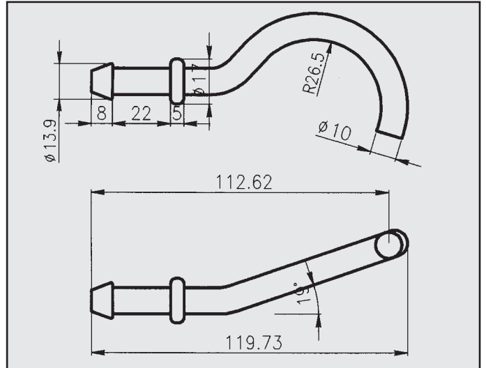
FORD ESCORT ATTACCO COD. AT 260271
