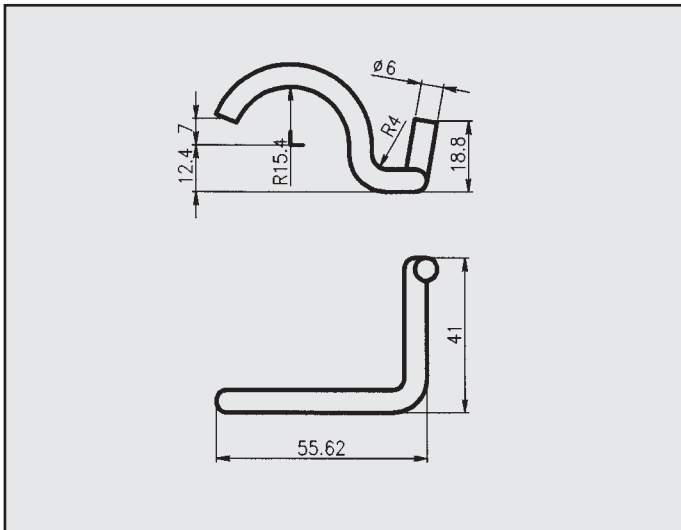
LIGIER ATTACCO COD. AT 390001
