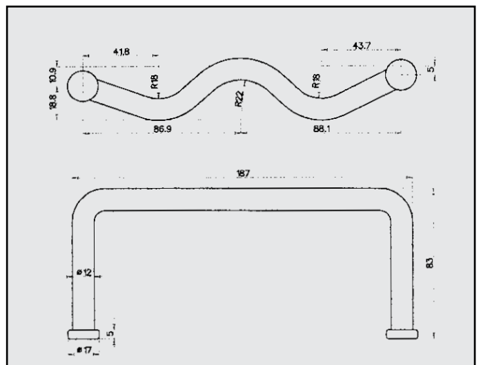
FIAT MAREA 1.6I 16V ATTACCO COD. AT 242815
