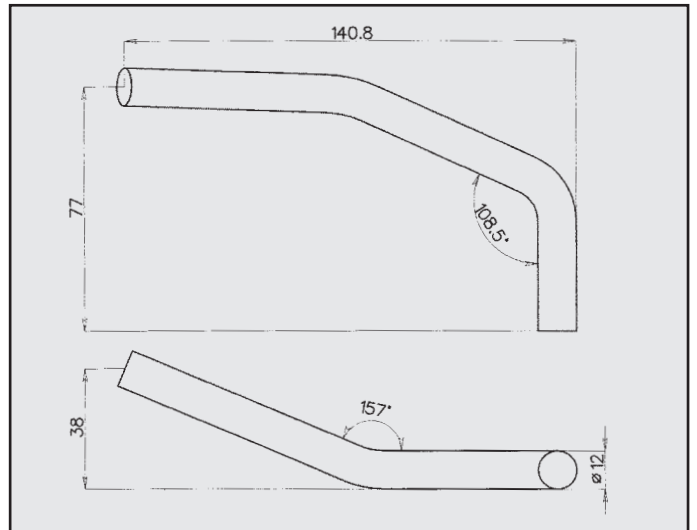
OPEL VECTRA ATTACCO COD. AT 520829
