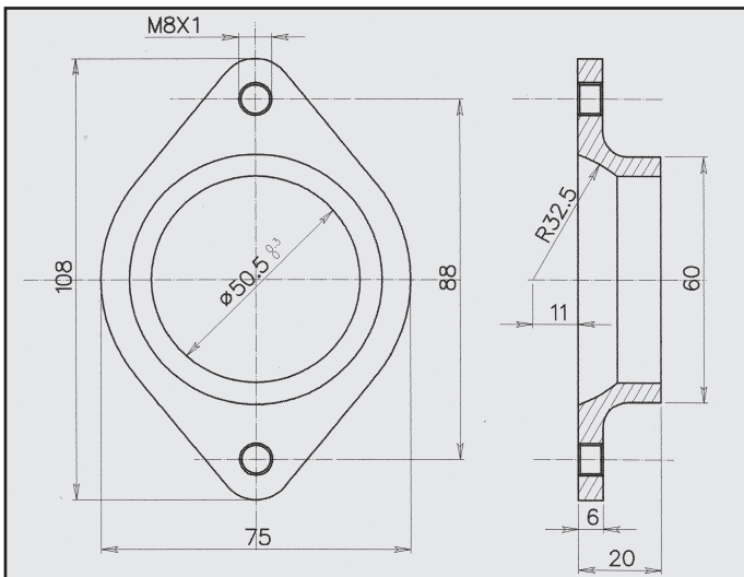
OPEL VECTRA FLANGIA COD. FL 520823
