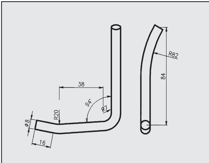
PEUGEOT GT ATTACCO COD. AT 540301
