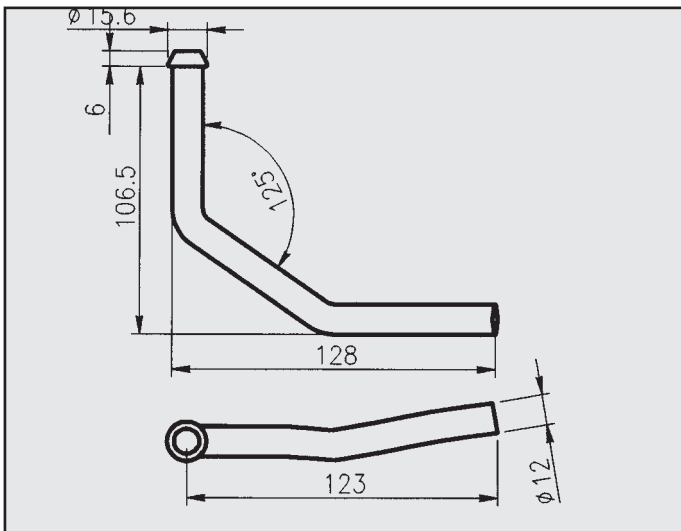
NISSAN PRIMERA 1.6 ATTACCO COD. AT 500414
