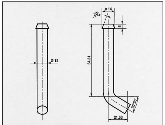
SEAT CORDOBA ATTACCO COD. AT 680604
