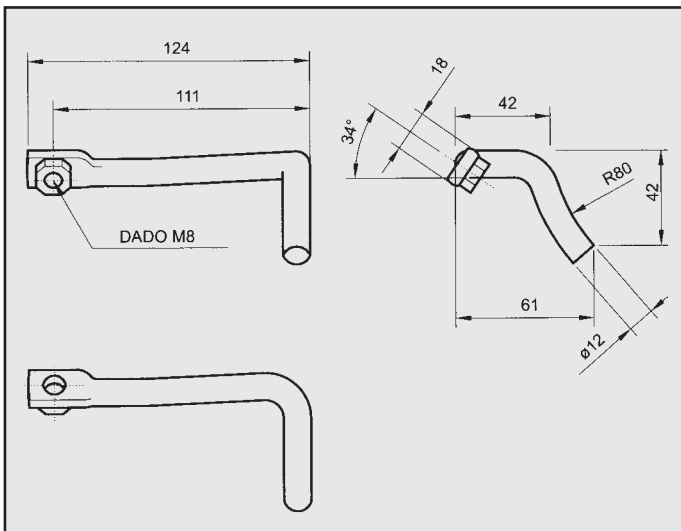
MITSUBISHI SPACE WAGON 2.0 ATTACCO per posteriore COD. AT 460304
