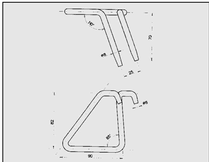
FIAT COUPE' 2.0 TURBO 16 V ECO ATTACCO COD. AT 242401
