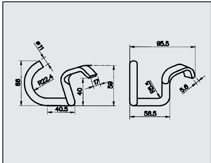
FIAT 600 ATTACCO COD. AT 243105
