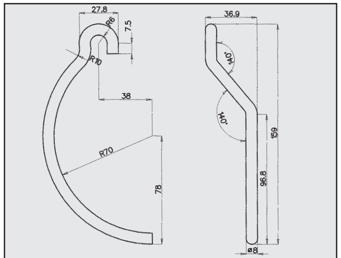
OPEL ATTACCO SX COD. AT 520025/SX
