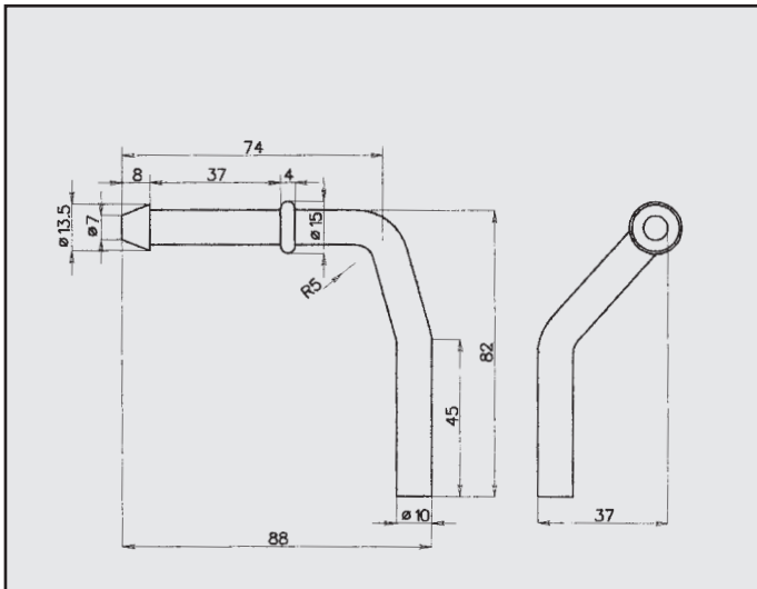
FORD FOCUS TURBO DIESEL ATTACCO COD. AT 261508
