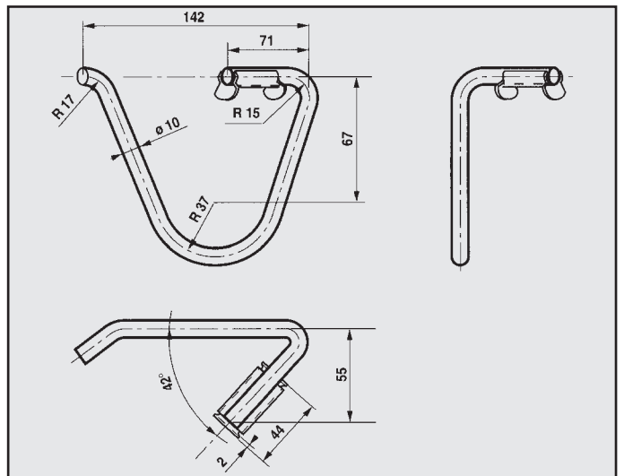
FORD FIESTA 89 1.3 CAT ATTACCO COD. AT 260328
