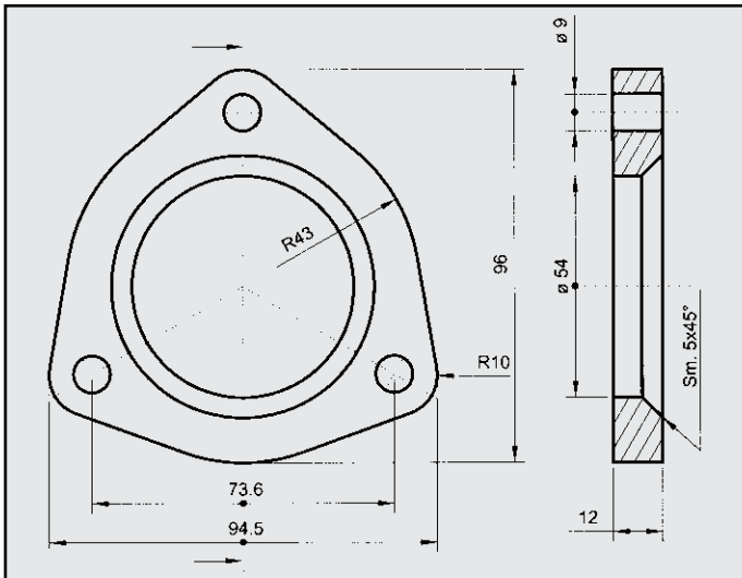
FIAT CROMA 2.5 FLANGIA COD. FL 240005
