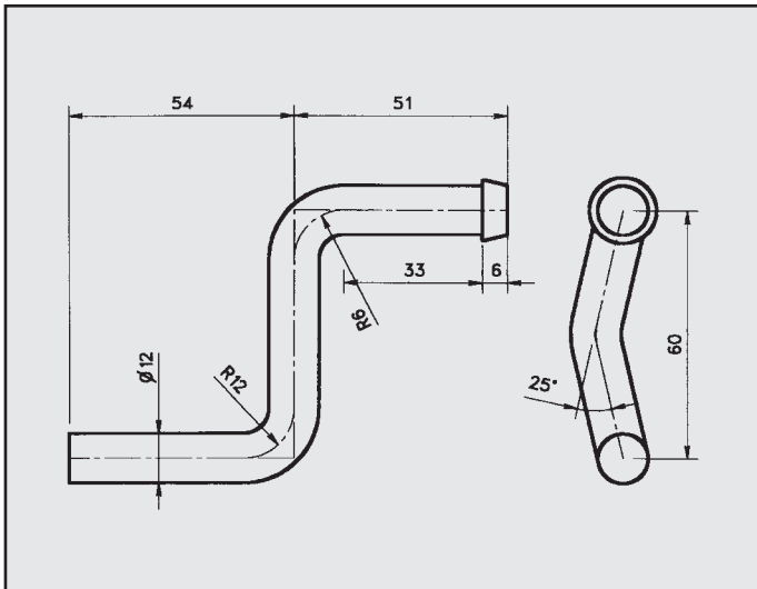
SUZUKI SWIFT ATTACCO COD. AT 720203
