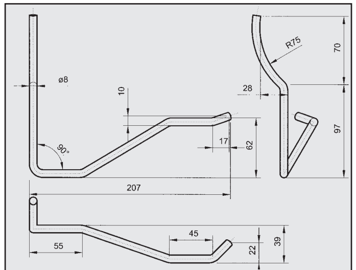
PEUGEOT ATTACCO COD. AT 540806
