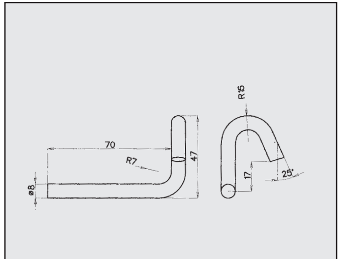
RENAULT MEGANE 1.9-2.0 ATTACCO COD. AT 601609
