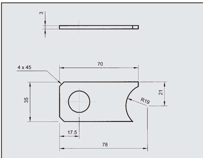
OPEL ATTACCO COD. AT 520016
