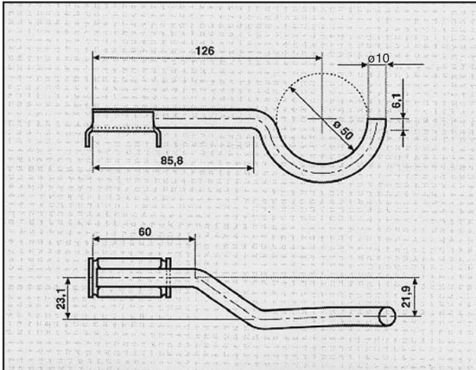
FORD ATTACCO COD. AT 260006
