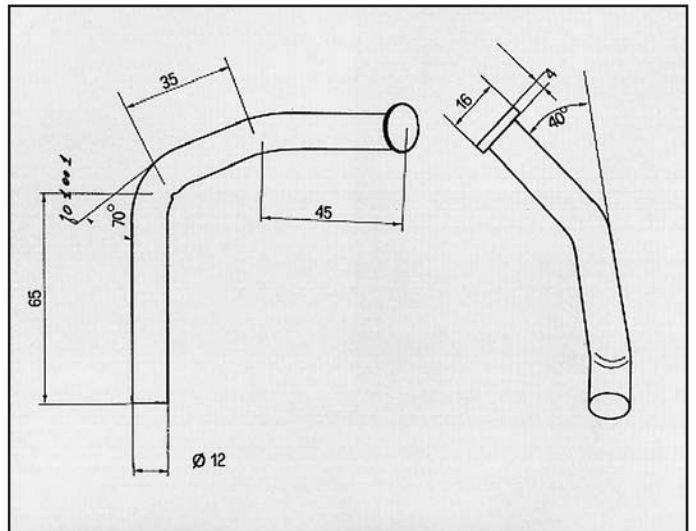
SUPRA 3.0 i TURBO ATTACCO COD. AT 801001
