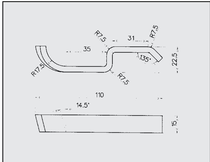
FIAT 600 ATTACCO COD. AT 243104
