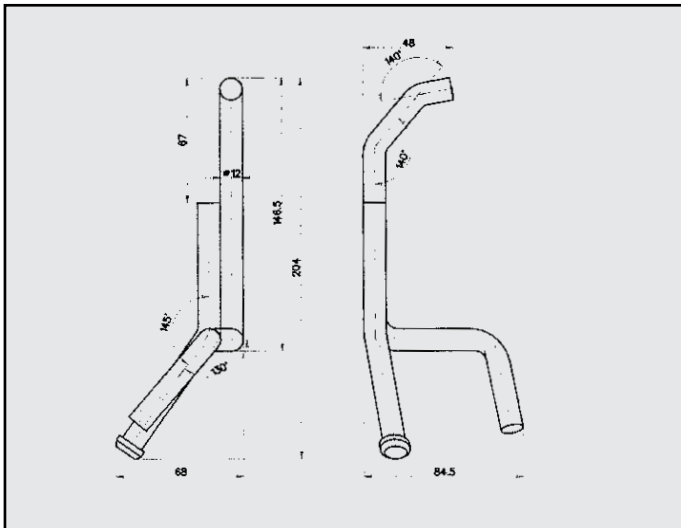
ALFA GTV ATTACCO COD. AT 020614
