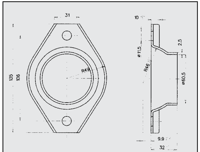
CITROEN JUMPER/PEUGEOT BOXER/SUZUKI FLANGIA COD. FL 140002
