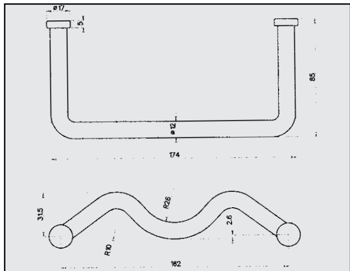
FIAT BRAVO-BRAVA 1.2 16V ATTACCO COD. AT 242326
