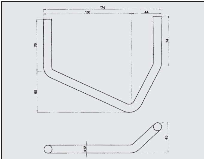
SAAB ATTACCO CENTRALE COD. AT 640001
