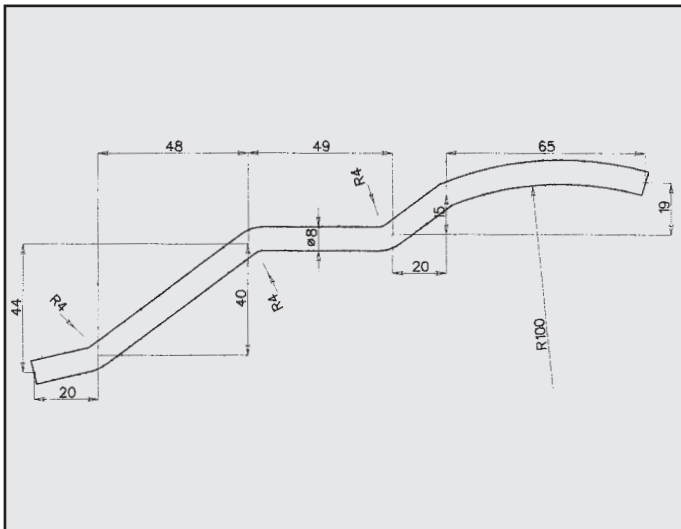
RENAULT KANGOOON 1.4 ATTACCO COD. AT 601702
