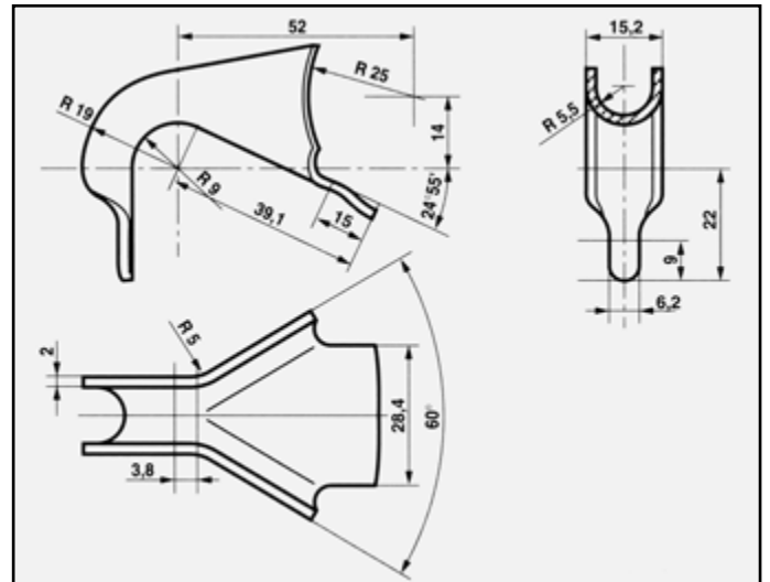
BMW 316 iE/91 ATTACCO centrale COD. AT 120010
