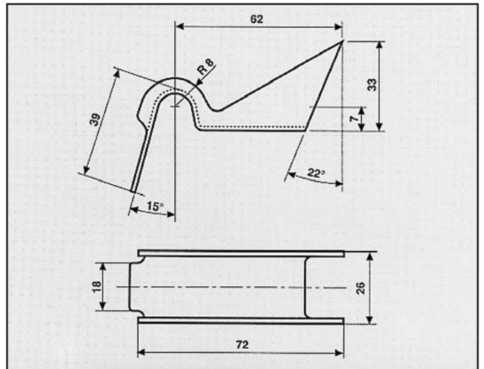
MERCEDES 200 TD S.W. ATTACCO posteriore COD. AT 440207/A
