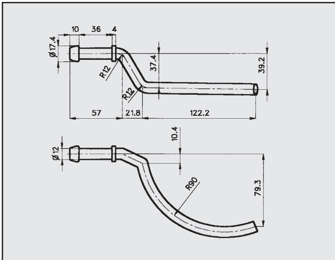
VOLKSWAGEN SHARAN 95 ATTACCO COD. AT 861203
