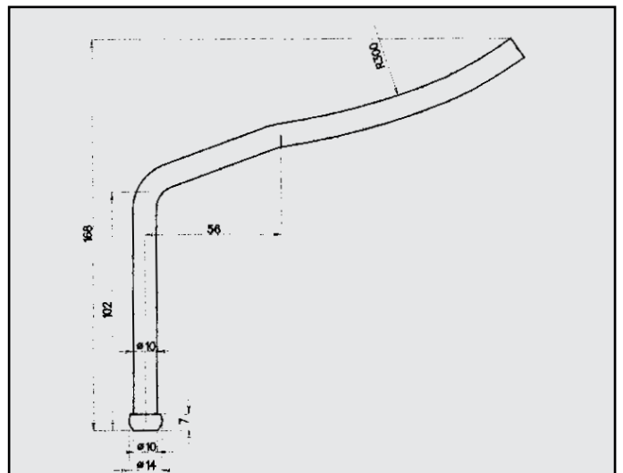
FIAT MAREA 2.4 TD ATTACCO COD. AT 242814
