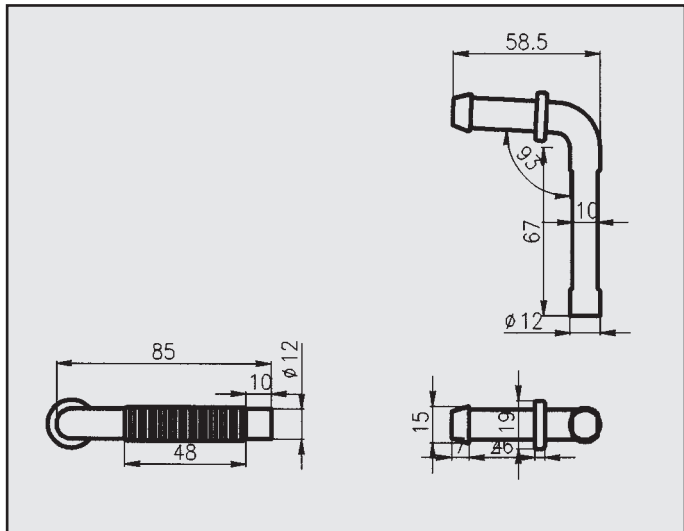
MASERATI ATTACCO COD. AT 400012
