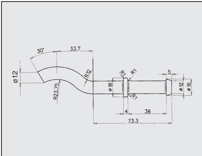
SEAT AROSA ATTACCO COD. AT 680804
