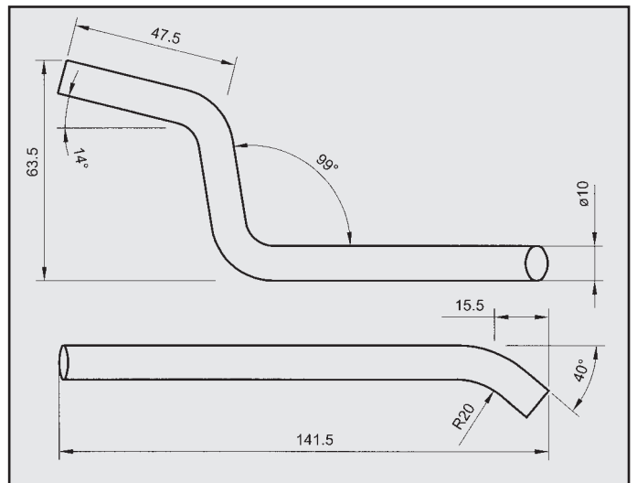
ROVER 213 ATTACCO COD. AT 620404
