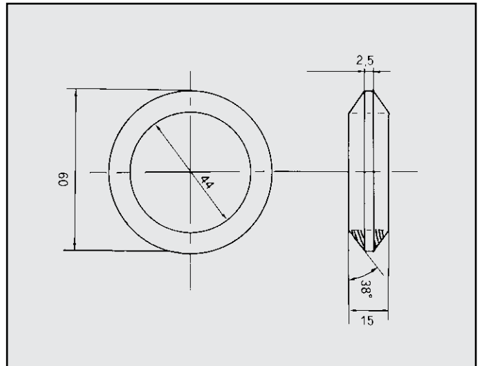
PEUGEOT 205 BENZINA ANELLO \varnothing esterno mm 60 \varnothing interno mm 44 COD. AN 540301
