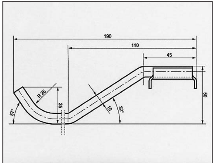
FORD FIESTA 1.1 E ATTACCO COD. AT 260327
