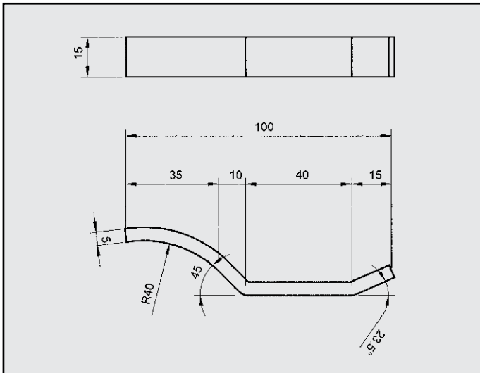
FIAT PANDA 4X4 ATTACCO COD. AT 240115
