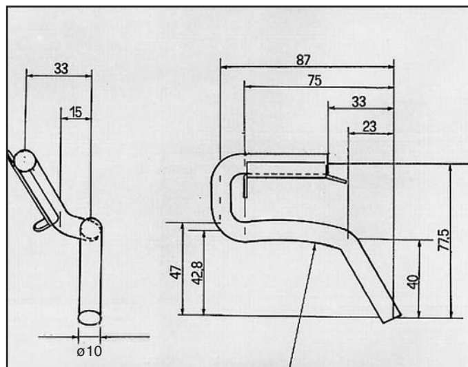
VECTRA 1400/1600 ATTACCO COD. AT 520804
