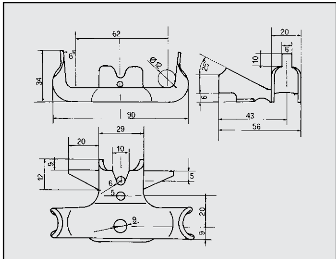
AUDI 80 1600/1800/1800 DIESEL ATTACCO per posteriore COD. AT 040304 893253609B 893253609H
