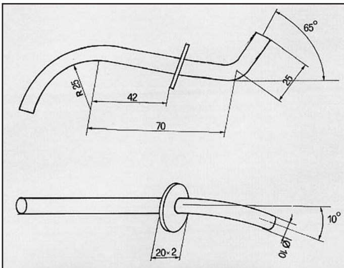
CRX 1500 ATTACCO COD. AT 280504
