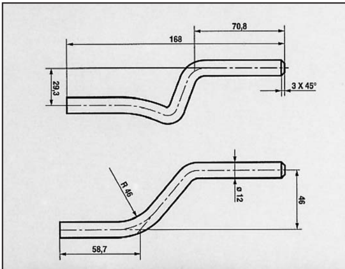
MERCEDES ATTACCO COD. AT 440008
