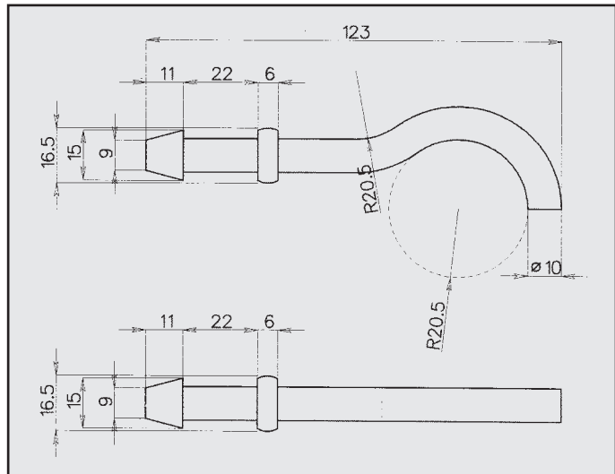
FORD MONDEO ATTACCO COD. AT 261222
