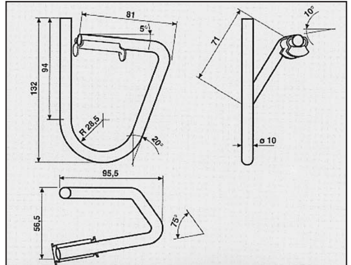
FORD FIESTA 1.6 XRL ATTACCO posteriore COD. AT 260320
