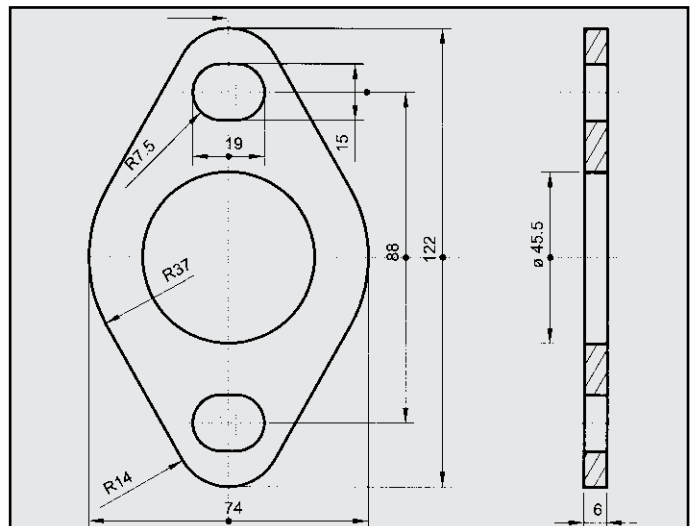
OPEL VECTRA FLANGIA COD. FL 520815
