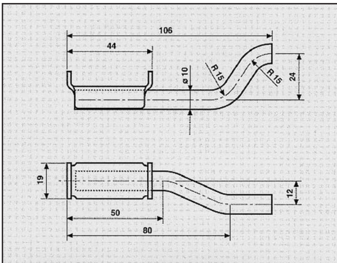
OPEL ATTACCO COD. AT 520813
