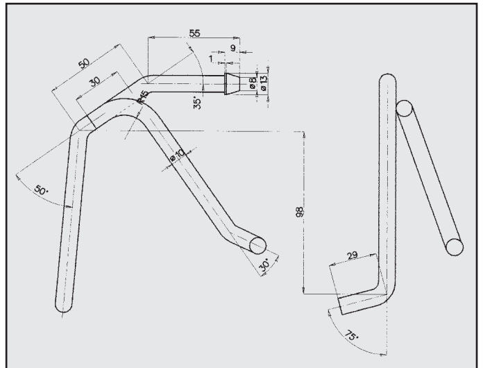
FORD FOCUS 1.6 ATTACCO COD. AT 261512
