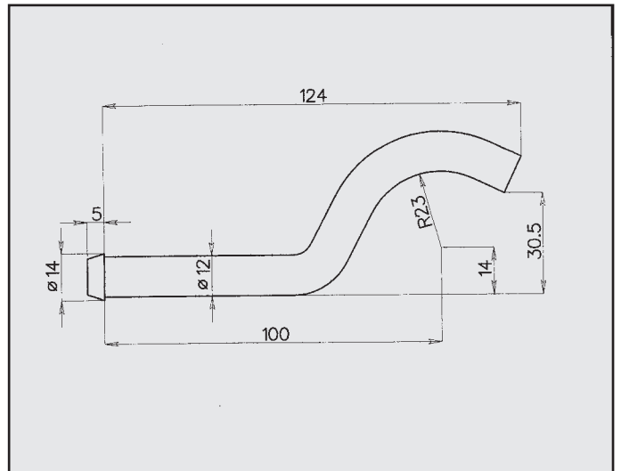
VOLKSWAGEN POLO ATTACCO X CENTRALE COD. AT 860314
