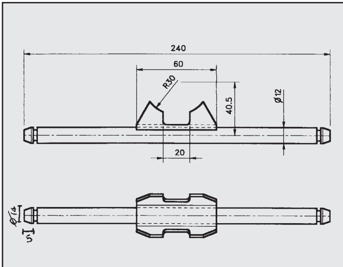
VOLKSWAGEN CORRADO ATTACCO COD. AT 860704
