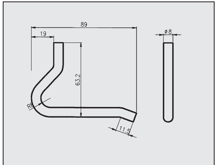
RENAULT CLIO 1.8 ATTACCO COD. AT 601307
