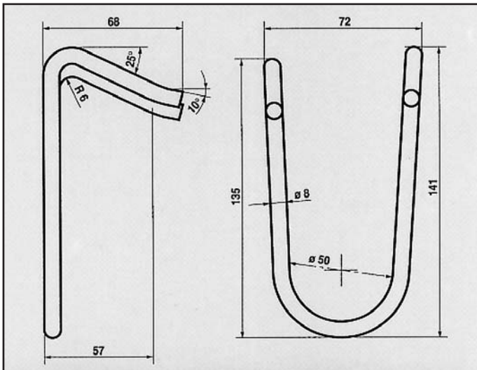
SEAT MALAGA-IBIZA 1.4/1.6 ATTACCO anteriore COD. AT 680504
