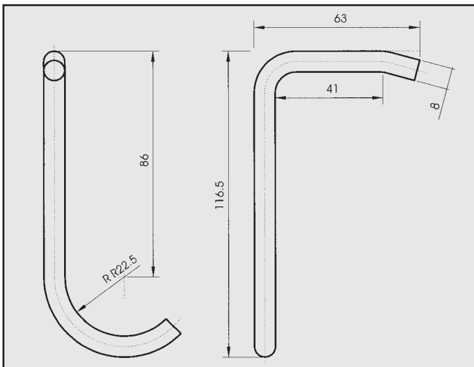
RENAULT CLIO 1.8 ATTACCO COD. AT 601304
