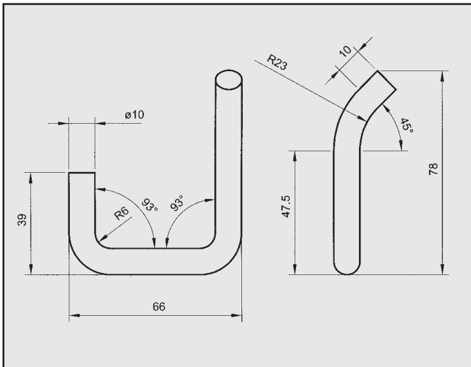
ROVER 213 ATTACCO COD. AT 620406
