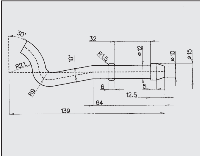
PEUGEOT ATTACCO COD. AT 540002
