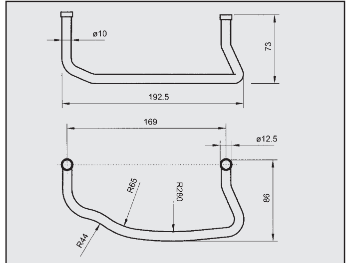
FORD ESCORT ATTACCO COD. AT 260260
