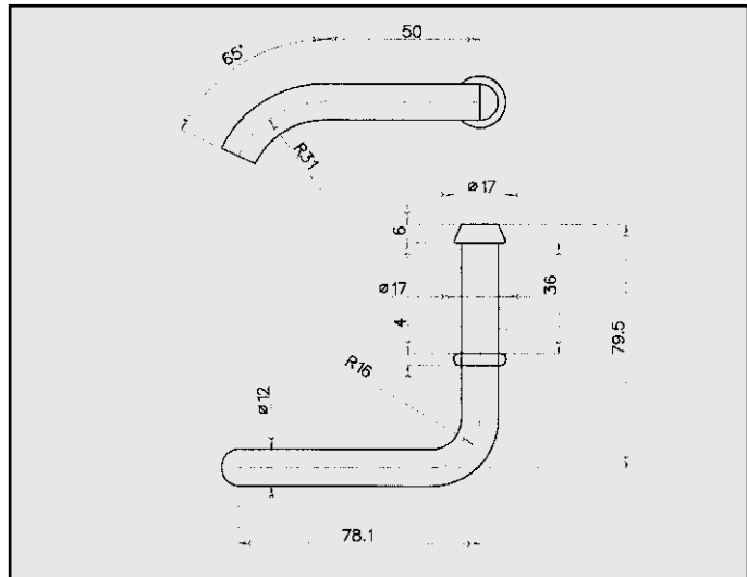
AUDI ATTACCO COD. AT 040006
