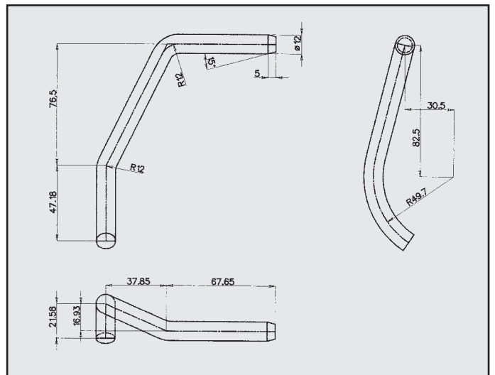
VOLKSWAGEN CADDY ATTACCO COD. AT 861302
