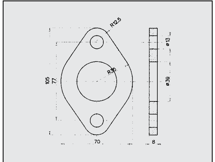
HYUNDAI ATHOS FLANGIA COD. FL 300303
