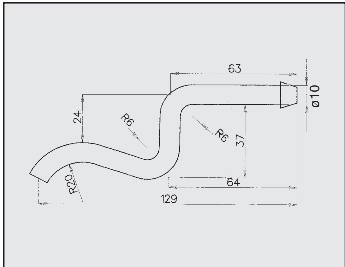
FORD FOCUS ATTACCO COD. AT 261505
