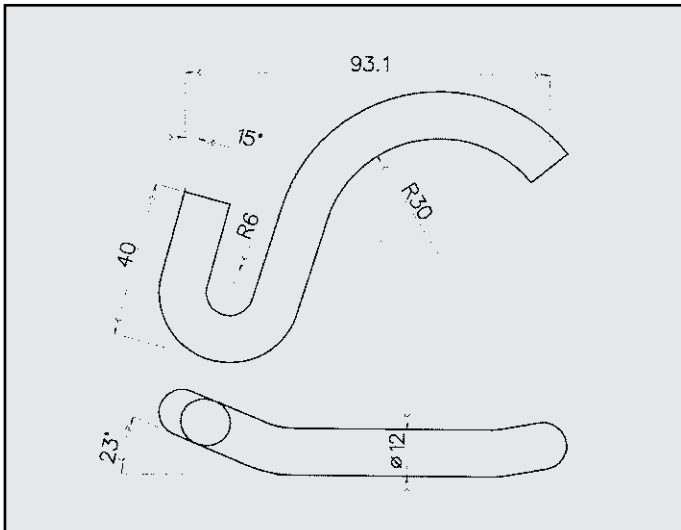
FIAT CROMA 2.0 IE ATTACCO COD. AT 242901
