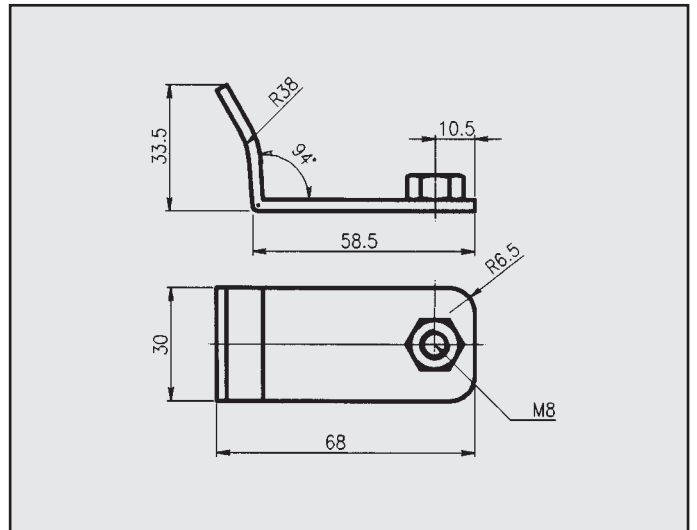
SUZUKI SJ 410 ATTACCO COD. AT 720303
