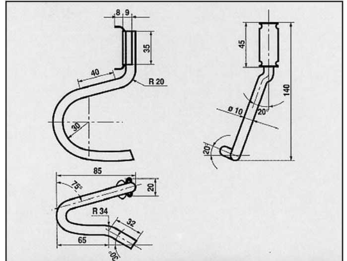
FORD SIERRA 2000/87 ATTACCO per posteriore COD. AT 260616
