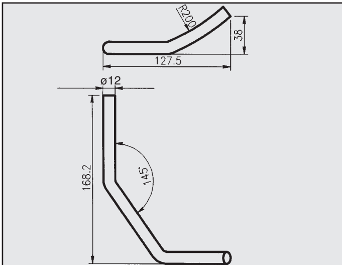
SEAT CORDOBA/ VARIO 1.4i KAT ATTACCO COD. AT 680606
