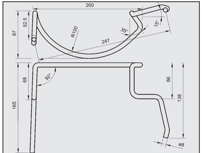
PEUGEOT 106 ATTACCO COD. AT 540805
