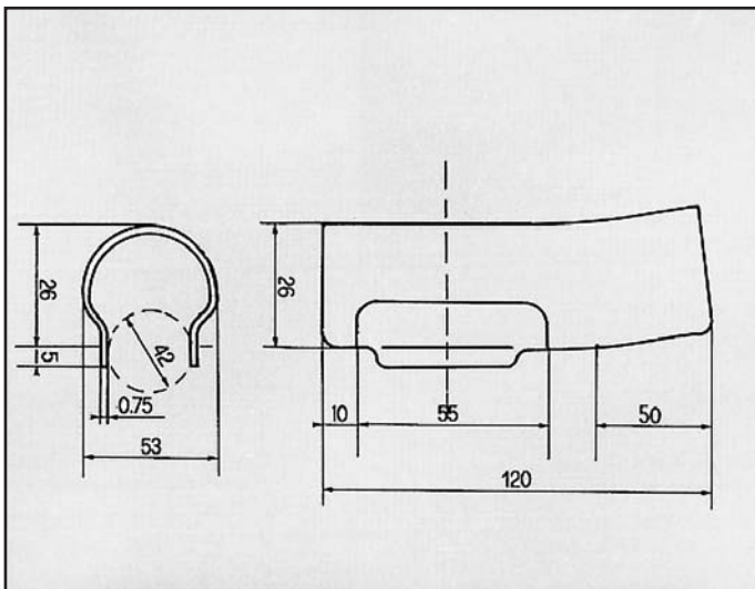
COROLLA CARTERINO COD. AT 800413
