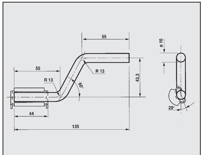
FORD SIERRA CAT ATTACCO COD. AT 260623
