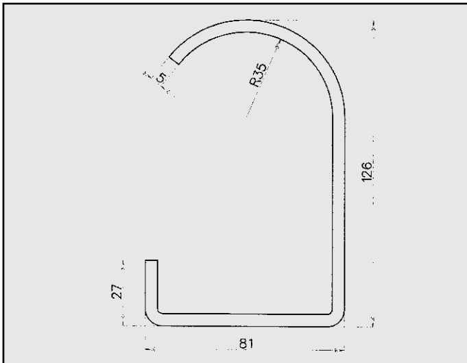
AUDI 100 ATTACCO COD. AT 040109
