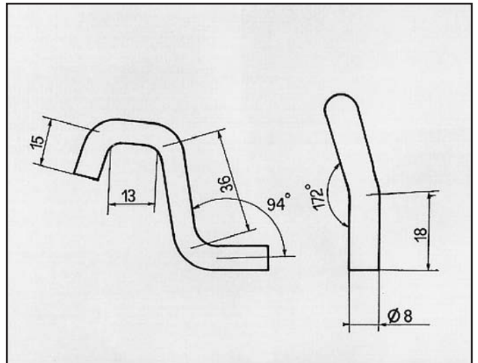
900 TURBO '84 ATTACCO COD. AT 640201
