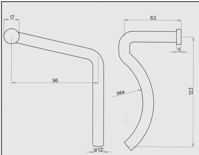
AUDI A6 ATTACCO COD. AT 040802
