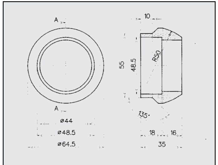
HYUNDAI PONY ANELLO COD. AN 300101
