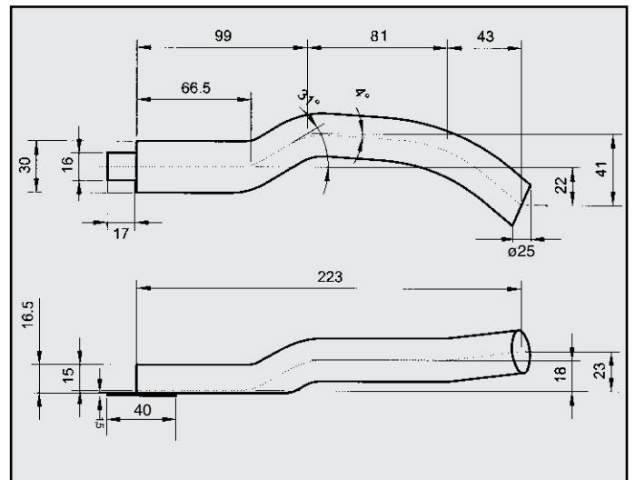
BMW 535 - 635 ATTACCO COD. AT 120215
