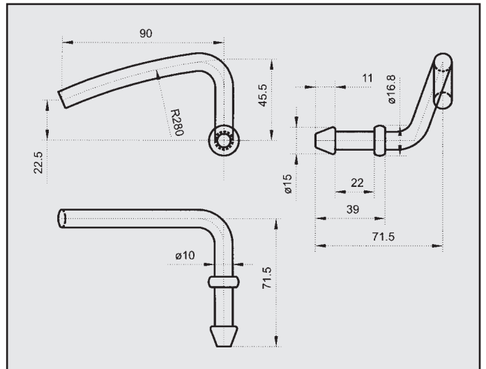
FORD FIESTA 1,2i CAT '95 ATTACCO posteriore COD. AT 260334
