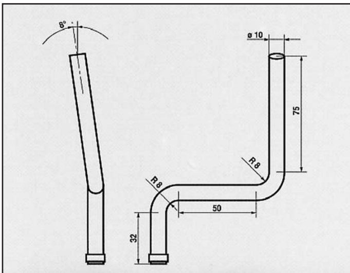
MAZDA 323 / 1986-87 ATTACCO per posteriore COD. AT 420604 52540100 B/C/F
