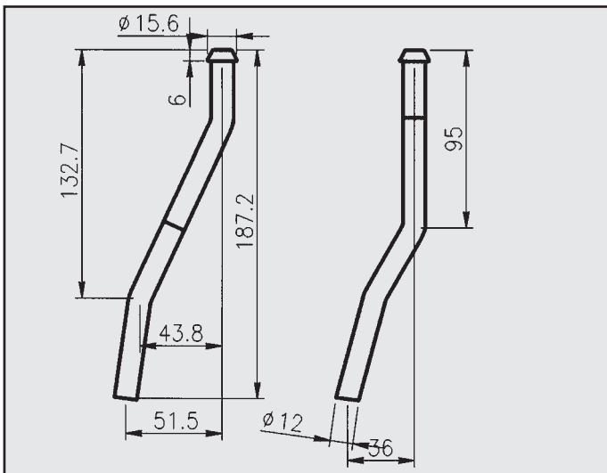
NISSAN PRIMERA 1.6 ATTACCO COD. AT 500415
