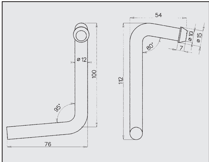
MASERATI ATTACCO COD. AT 400010
