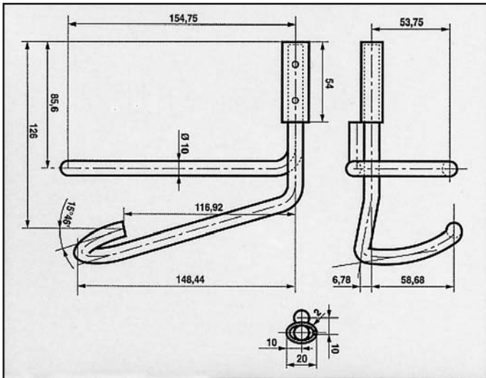
FORD SCORPIO 2.0 E ATTACCO COD. AT 260804
