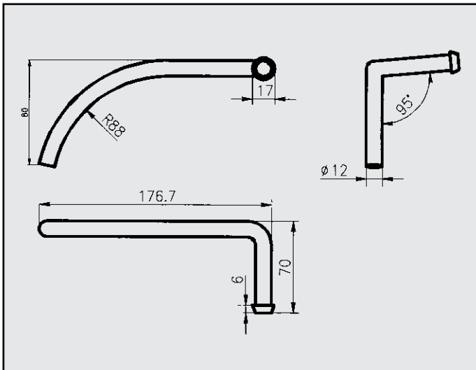
FIAT ULISSE 2.0 I.E. TD 1.9 2.1 ATTACCO COD. AT 242707
