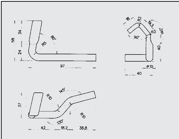
ALFA GTV ATTACCO COD. AT 020608
