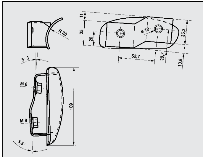
AUDI 100/1994 ATTACCO COD. AT 040105 DX
