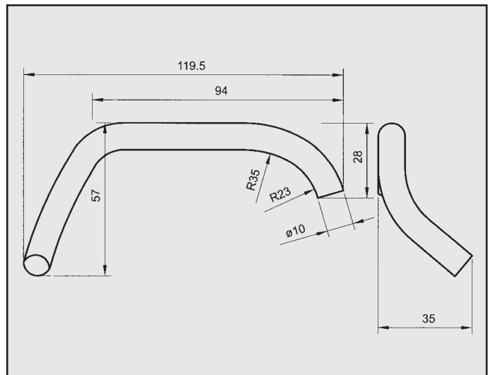
HONDA CIVIC ATTACCO COD. AT 280420
