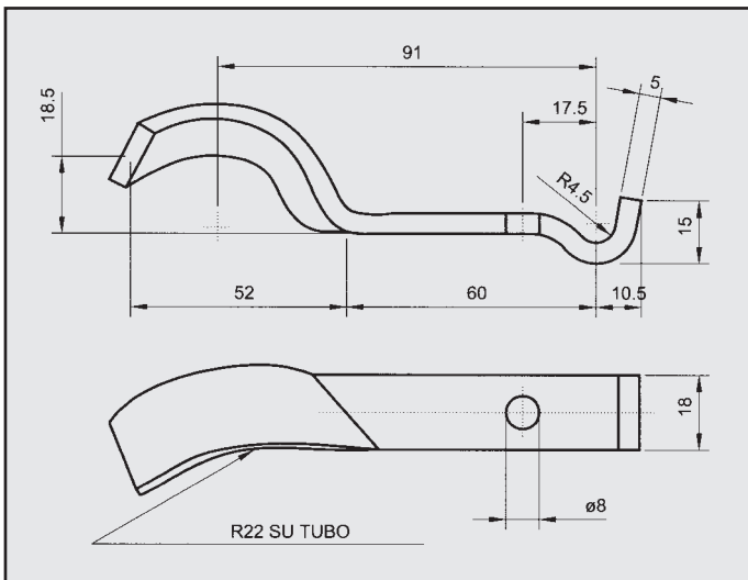
RENAULT 25 ATTACCO COD. AT 600603
