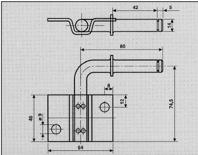
OPEL ATTACCO COD. AT 520003
