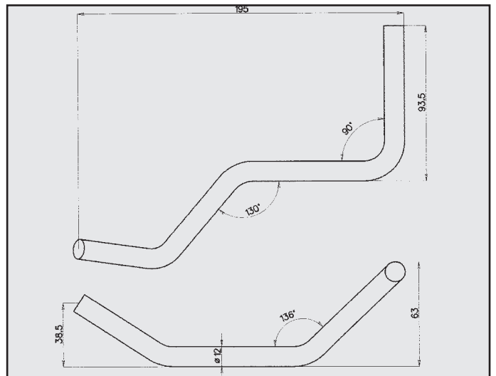
OPEL VECTRA ATTACCO COD. AT 520831
