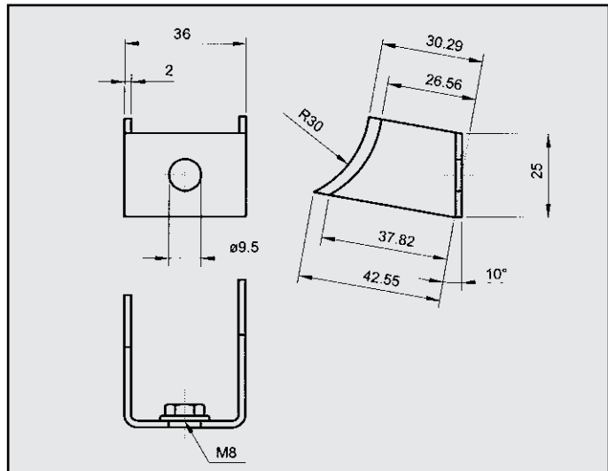
AUDI ATTACCO COD. AT 040106
