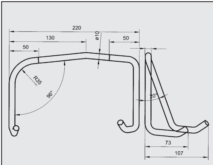
ROVER 416 ATTACCO COD. AT 620706
