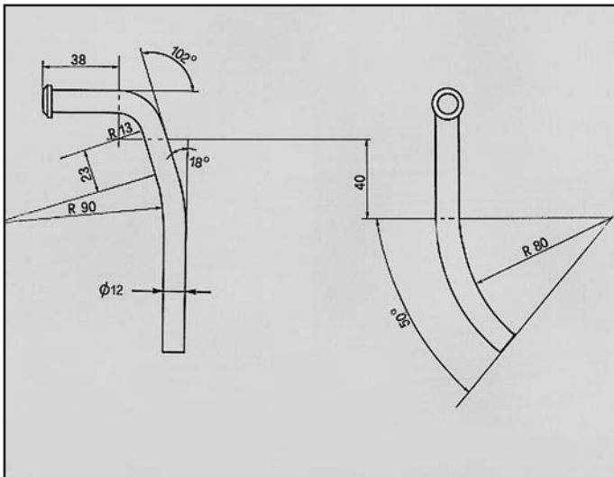
CAMRY 2 ATTACCO COD. AT 800105
