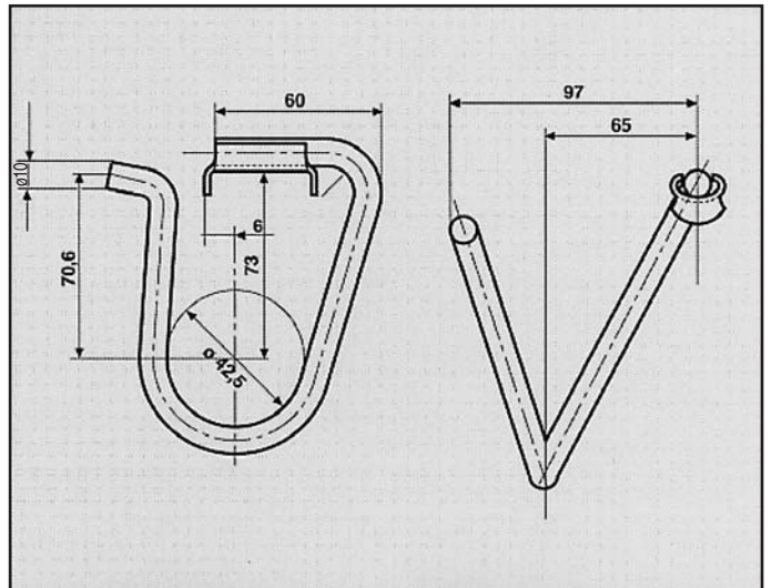
FORD FIESTA/ESCORT ATTACCO COD. AT 260326
