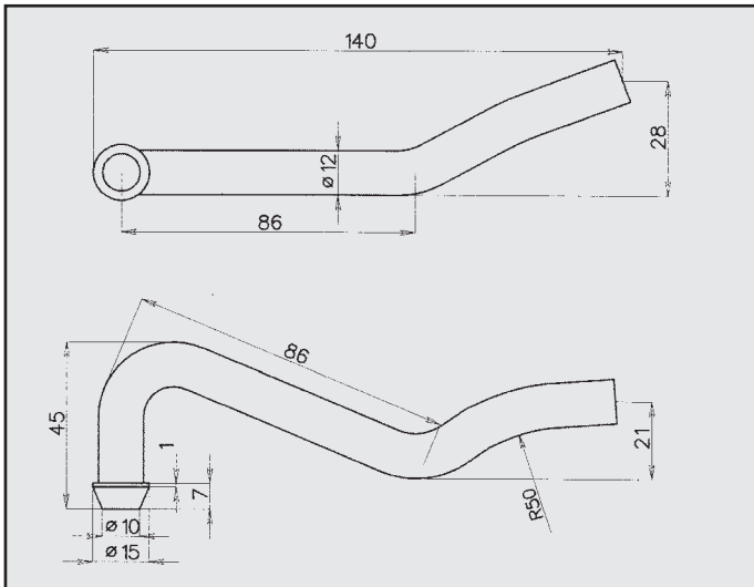
TOYOTA COROLLA 92 ATTACCO POSTERIORE COD. AT 800423
