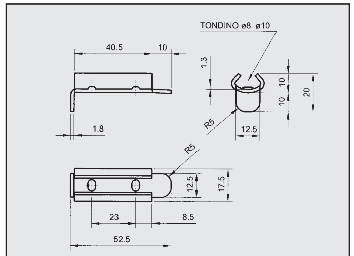
FORD PIASTRINA COD. PI 260101
