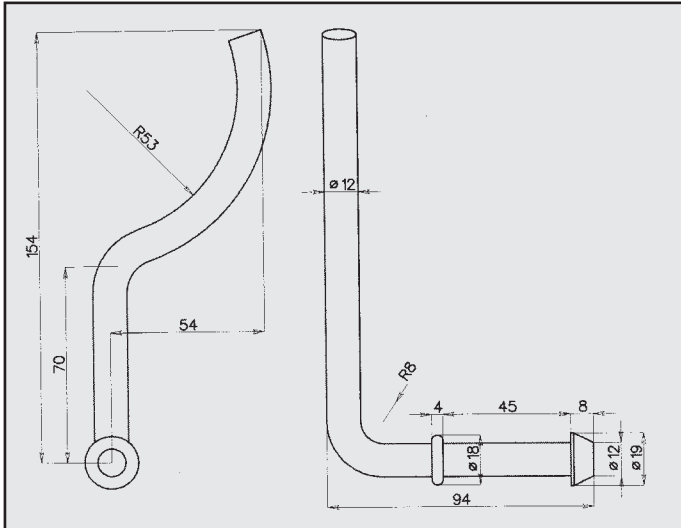
PEUGEOT 406 1.6-1.8 ATTACCO COD. AT 541103/SX
