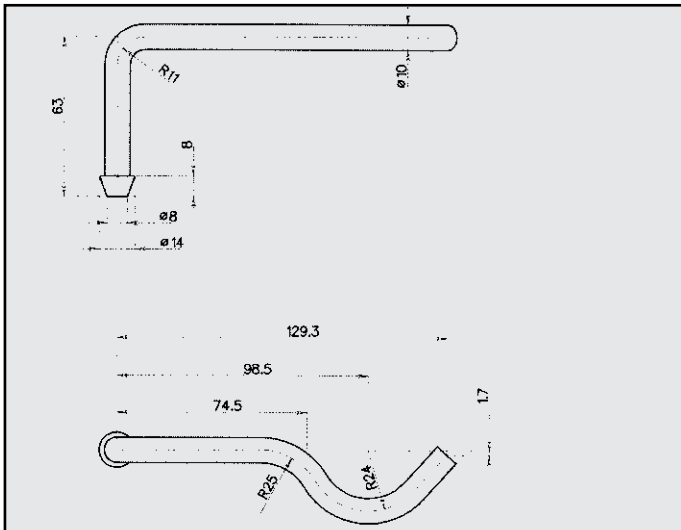
FIAT ATTACCO COD. AT 240015
