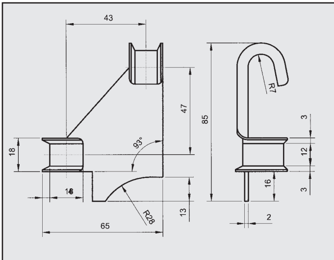
RENAULT R 20 1.6 - 2.0 '76 - '85 ATTACCO COD. AT 600602
