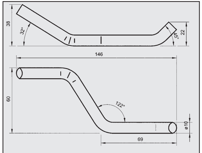
ROVER 416 ATTACCO COD. AT 620703
