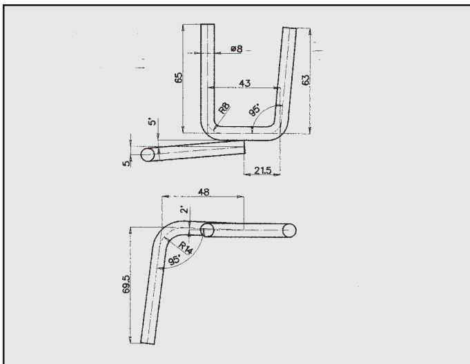
RENAULT LAGUNA 1800 ATTACCO COD. AT 601406
