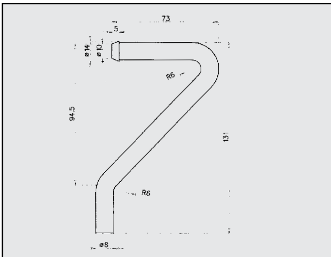
FIAT ULISSE ATTACCO COD. AT 242708
