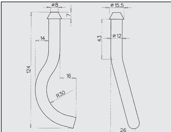
VOLKSWAGEN POLO ATTACCO COD. AT 860312
