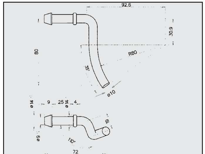
BMW 323 ATTACCO COD. AT 120116
