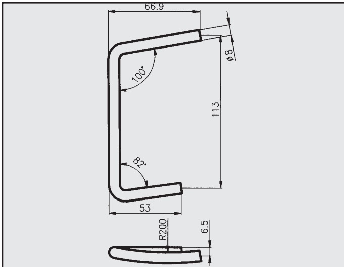
FORD ESCORT/ORION ATTACCO COD. AT 260220
