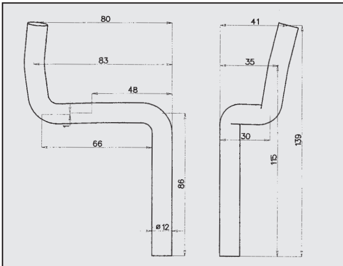
SAAB 900 ATTACCO COD. AT 640211
