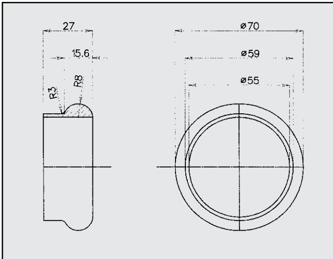
MITSUBISHI PAJERO 2.8 ANELLO COD. AN 460213
