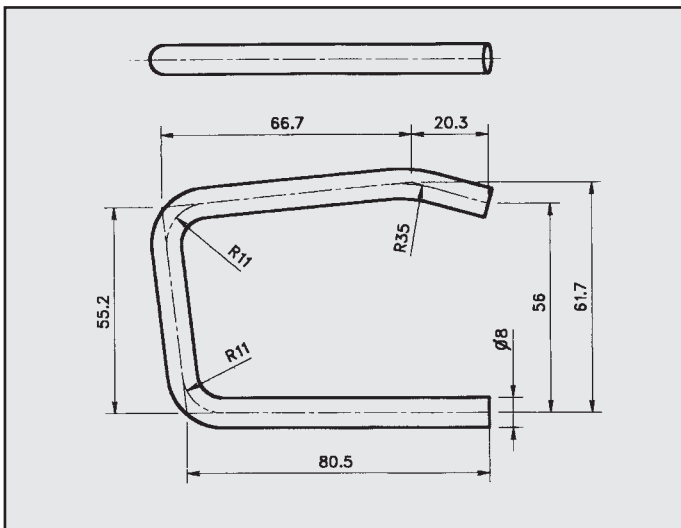
PEUGEOT 106 CAT ATTACCO COD. AT 540802
