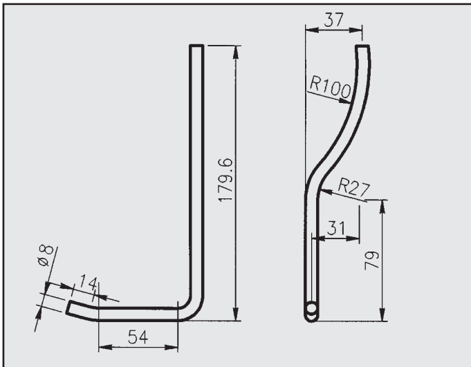
PEUGEOT 205 GT ATTACCO COD. AT 540302
