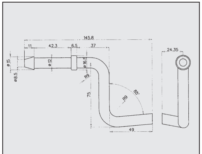
FORD FOCUS ATTACCO SUP. POSTERIORE COD. AT 261514
