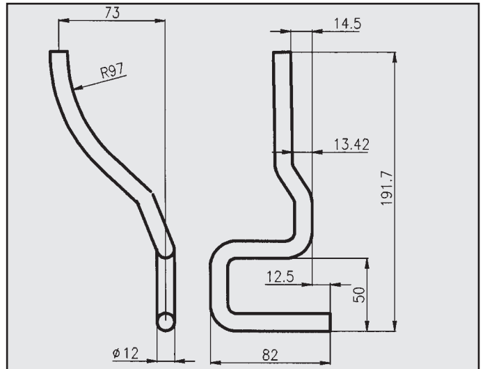
OPEL ASTRA ATTACCO COD. AT 520918
