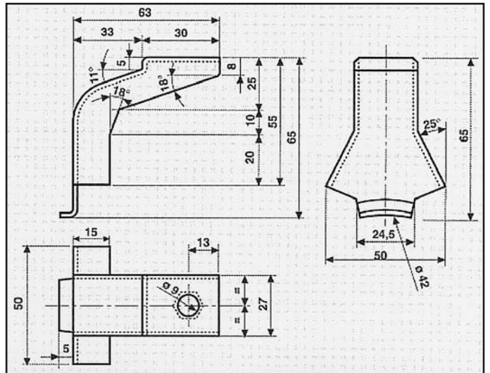
SUZUKI VITARA ATTACCO marmitta posteriore COD. AT 720104
