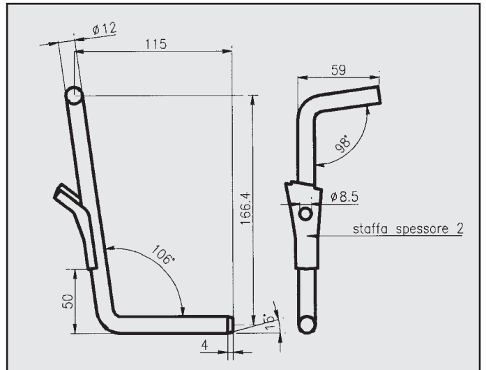
VOLKSWAGEN PASSAT 1.8 ATTACCO COD. AT 860211
