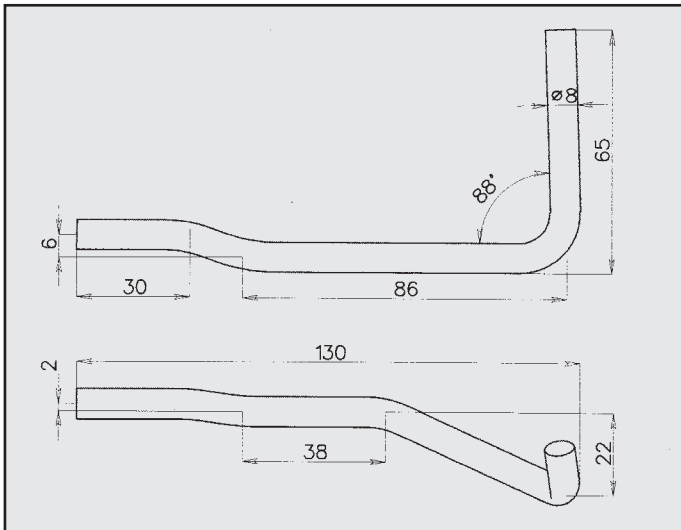
MICROCAR ATTACCO COD. AT 450101
