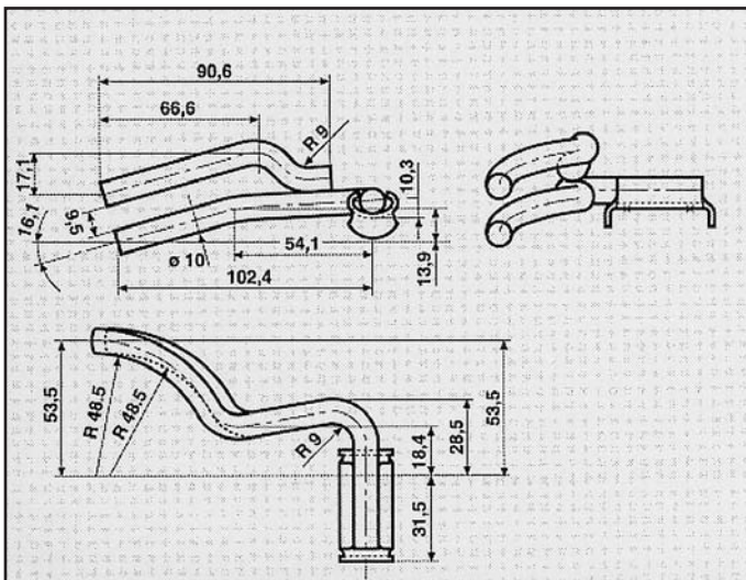
FORD ATTACCO posteriore COD. AT 260008
