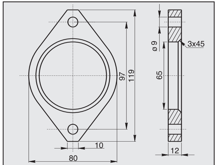
OPEL VECTRA TURBO DIESEL FLANGIA COD. FL 520825
