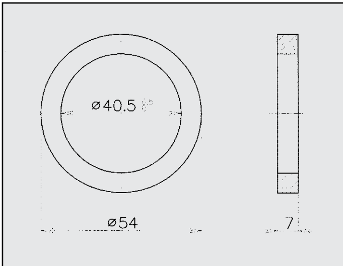
PEUGEOT ANELLO COD. AN 540003
