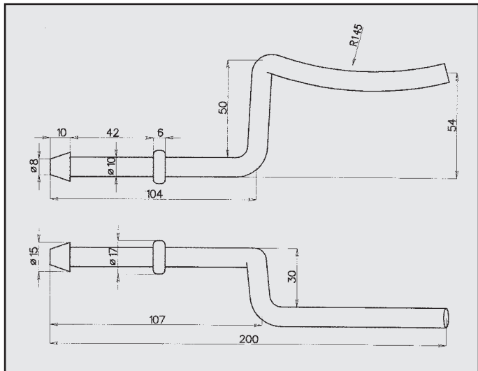
FORD FOCUS ATTACCO COD. AT 261506
