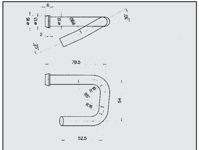
ALFA GTV ATTACCO COD. AT 020612
