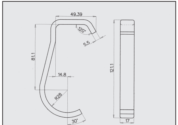
ALFA 167 ATTACCO COD. AT 021401
