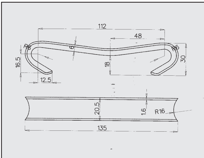
MERCEDES 300 TDI ATTACCO COD. AT 440210
