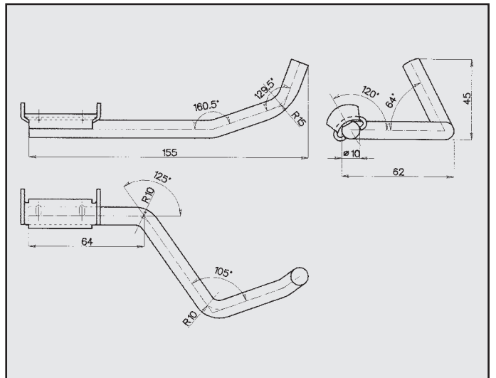
FORD ESCORT ATTACCO COD. AT 260281
