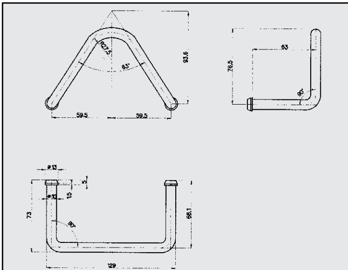
FIAT ATTACCO COD. AT 240016
