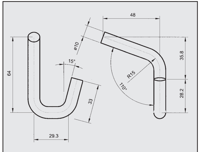
HONDA PRELUDE 1.8 EX ATTACCO posteriore COD. AT 280004
