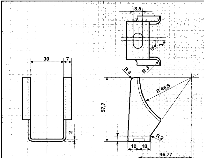
BMW ATTACCO COD. AT 120001
