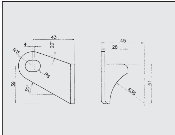
PEUGEOT 205 ATTACCO COD. AT 540321
