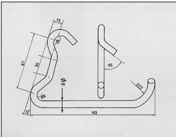
340/343/345 DLS81 ATTACCO per posteriore COD. AT 880102/L
