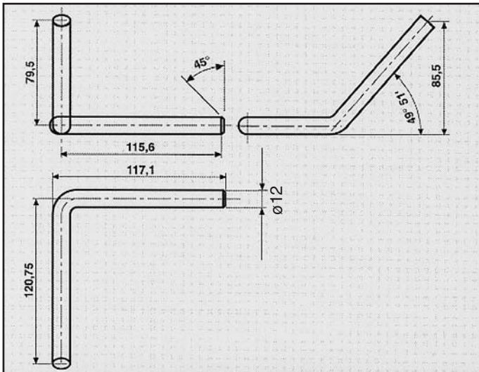
OPEL VECTRA/CALIBRA ATTACCO COD. AT 520811
