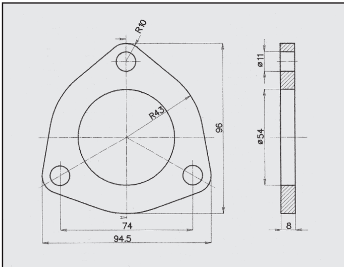
OPEL KADETT FLANGIA COD. FL 520115
