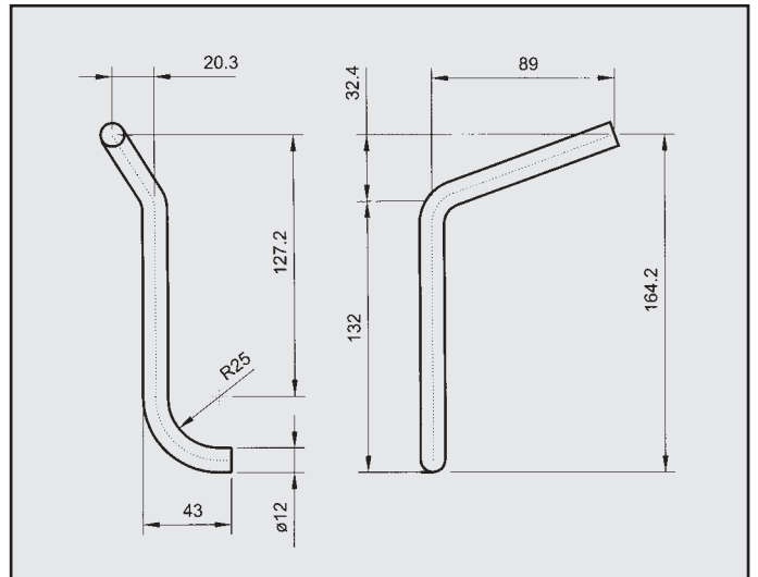
VOLKSWAGEN TRANSPORTER D. ATTACCO COD. AT 861103
