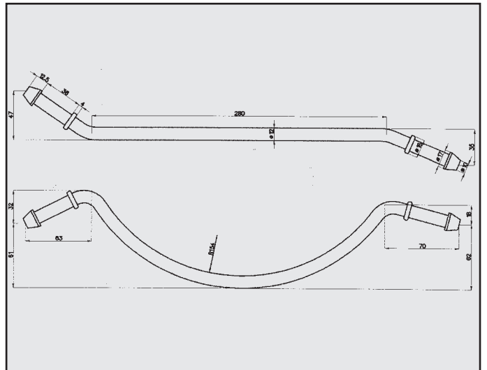
LANCIA K ATTACCO COD. AT 380906
