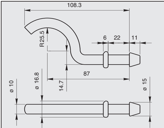
ALFA 155 16V TWIN SPARK 1.6 1.8 2.0 ATTACCO COD. AT 021014
