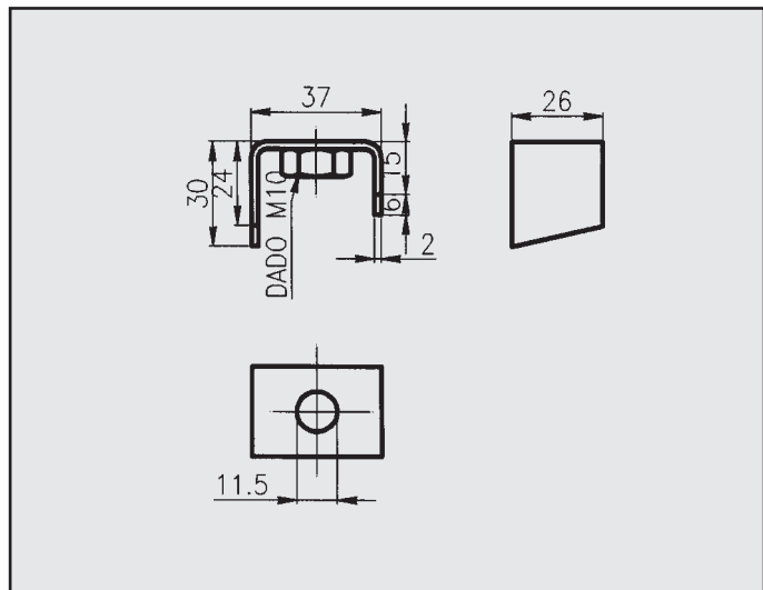
SAAB 900 ATTACCO COD. AT 640209
