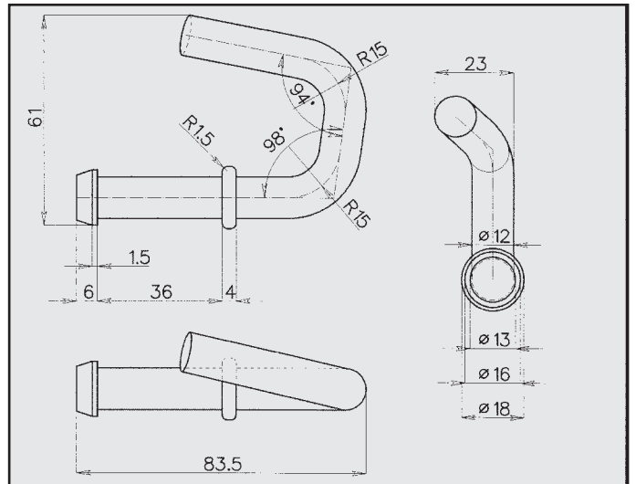
SKODA FABIA ATTACCO COD. AT 690401
