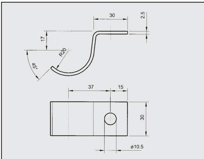
RENAULT R4 ATTACCO COD. AT 600801
