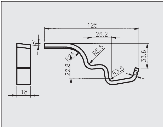
VOLVO 850 TDI ATTACCO COD. AT 880802
