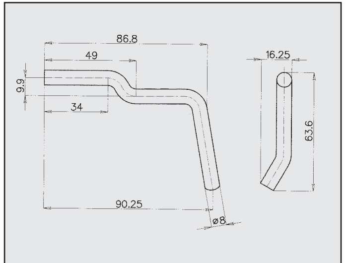
MICROCAR ATTACCO COD. AT 450104
