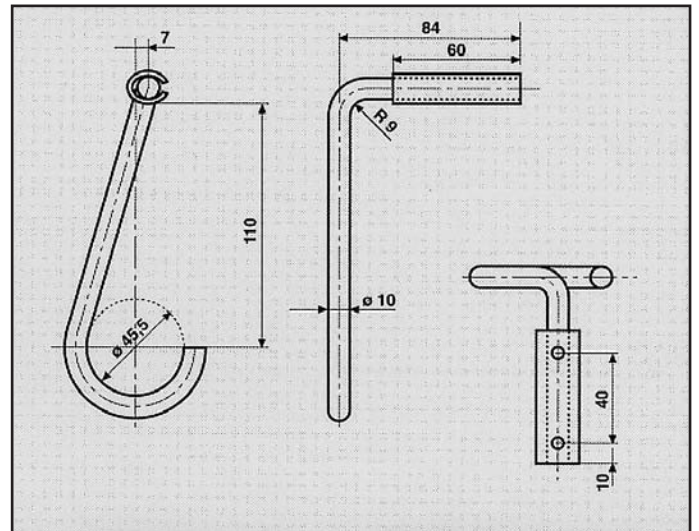
OPEL ATTACCO COD. AT 520011
