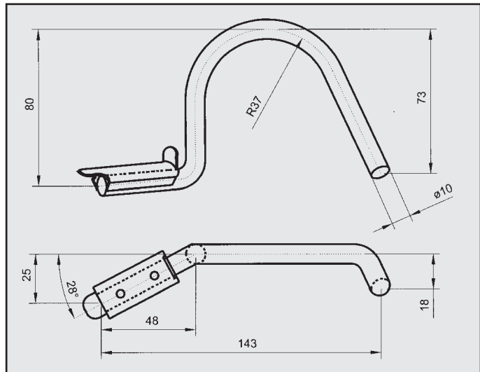
FORD SIERRA ATTACCO posteriore COD. AT 260609
