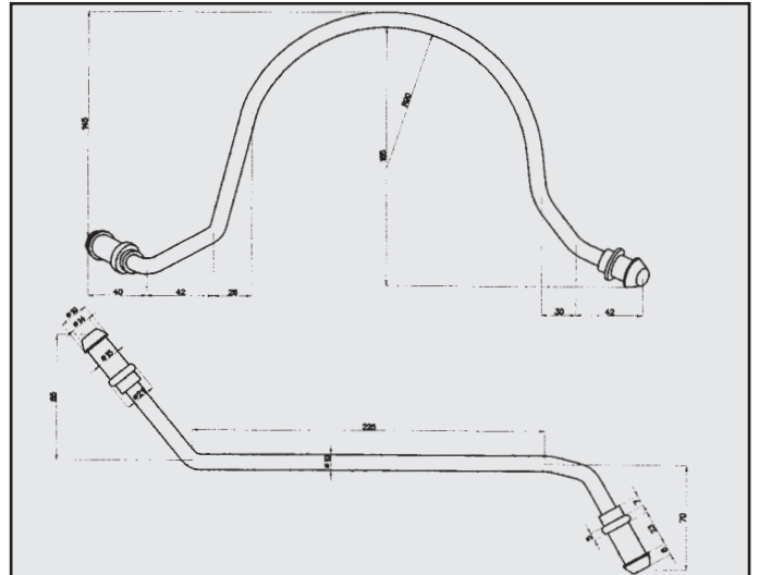
PEUGEOT 206 ATTACCO COD. AT 541201
