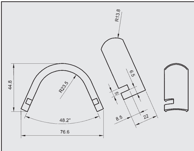
PEUGEOT 205 RALLY ATTACCO COD. AT 540316
