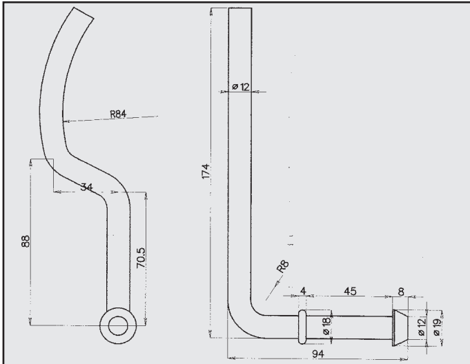
PEUGEOT 406 1.6-1.8 ATTACCO COD. AT 541103/DX
