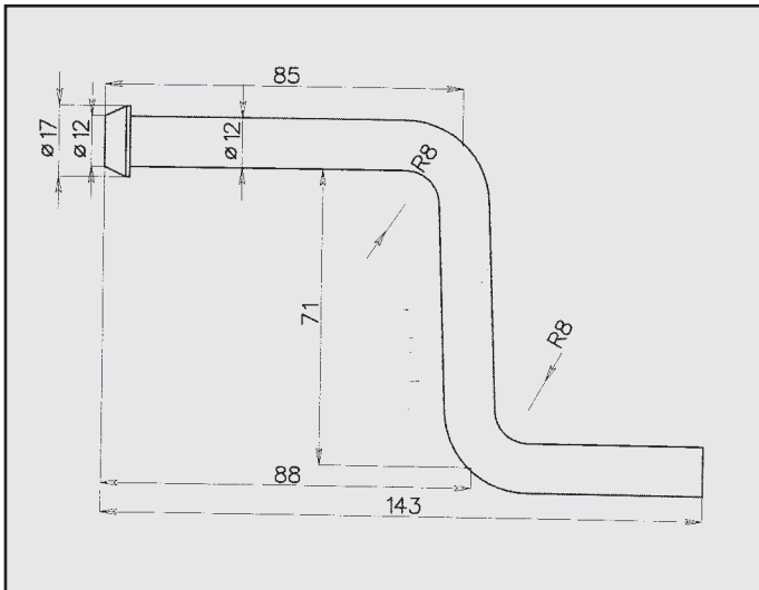
OPEL ASTRA ATTACCO COD. AT 520928
