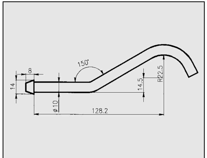
FIAT PALIO ATTACCO COD. AT 243004
