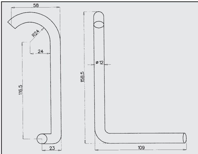
MERCEDES 200 ATTACCO COD. AT 440209
