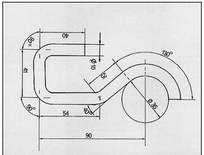
626 1600/2000 ATTACCO tubo posteriore COD. AT 420510
