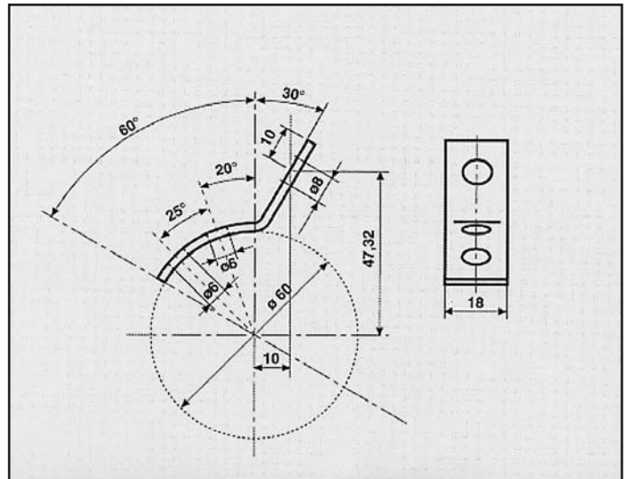
MERCEDES '93 ATTACCO COD. AT 440004
