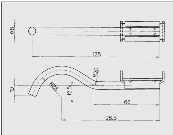
FORD FIESTA ATTACCO COD. AT 260362
