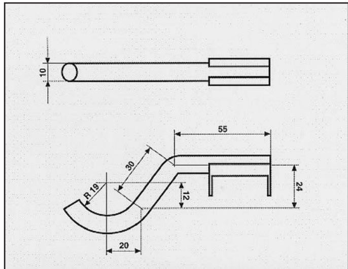
FORD ESCORT S.W./ORION 1.3 ATTACCO posteriore COD. AT 260238 6493599
