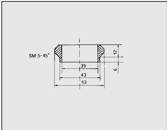
CITROEN GSA CLUB ANELLO \varnothing esterno mm 53 \varnothing interno mm 39 COD. AN 140401
