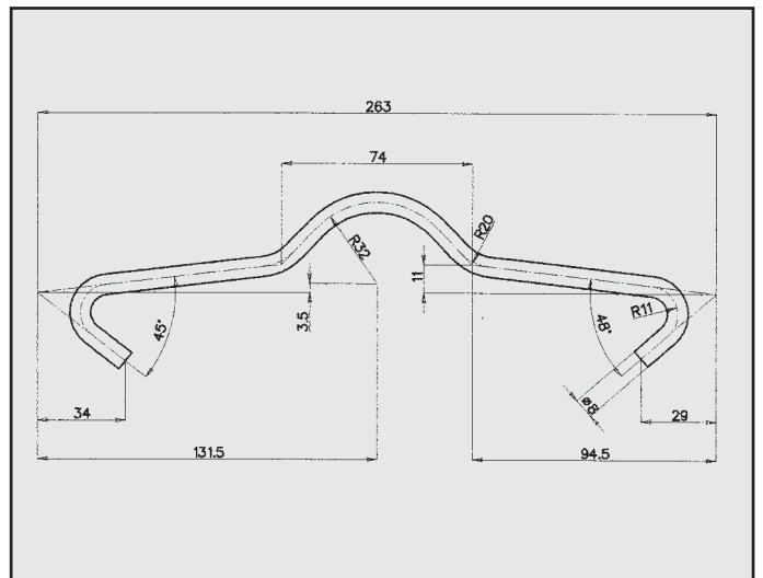
RENAULT MEGANE STAFFA CENTRALE COD. AT 601611
