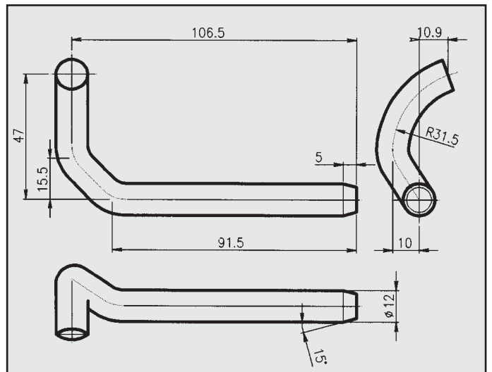
VOLKSWAGEN ATTACCO COD. AT 860006
