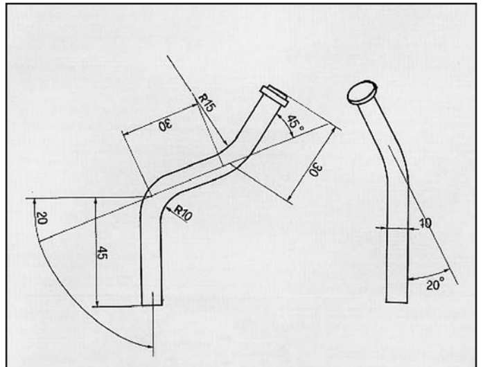
NEW CITY 1.3 ATTACCO COD. AT 280802
