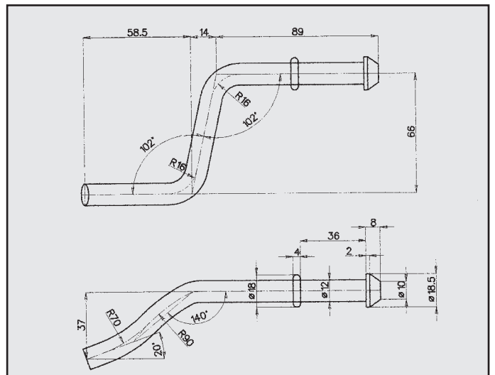
MERCEDES 190 ATTACCO COD. AT 440305
