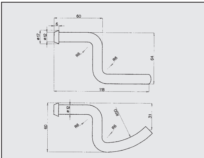
TOYOTA YARIS 1.0 16V ATTACCO COD. AT 801201
