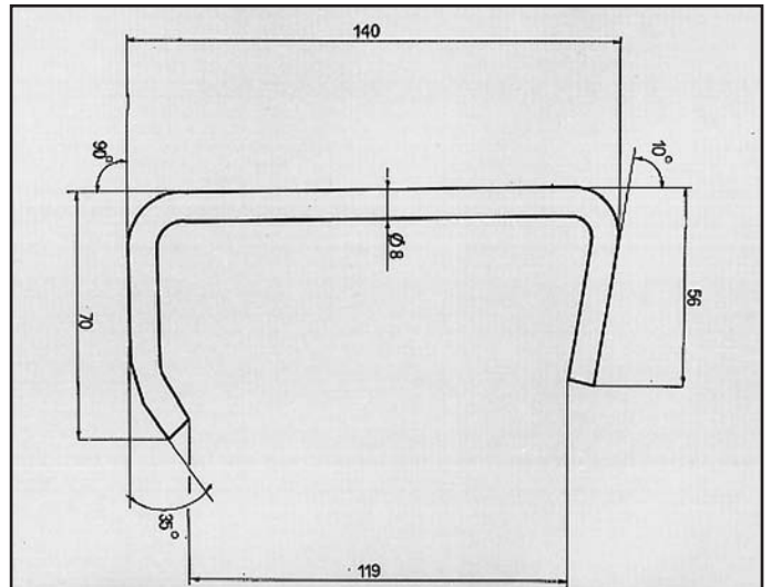
ACTY ATTACCO COD. AT 280203
