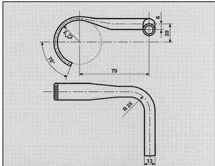
OPEL ATTACCO COD. AT 520004
