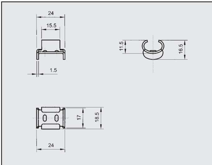
FORD PIASTRINA COD. PI 260103
