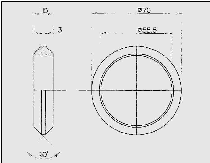
PEUGEOT 306 ANELLO COD. AN 540906
