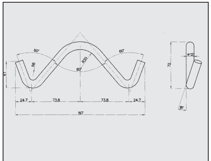
MERCEDES ATTACCO COD. AT 440016
