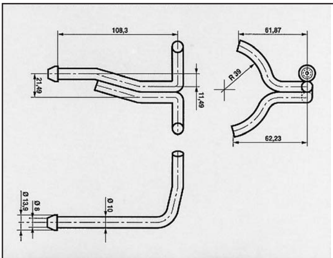
FORD SCORPIO 95 ATTACCO COD. AT 260806
