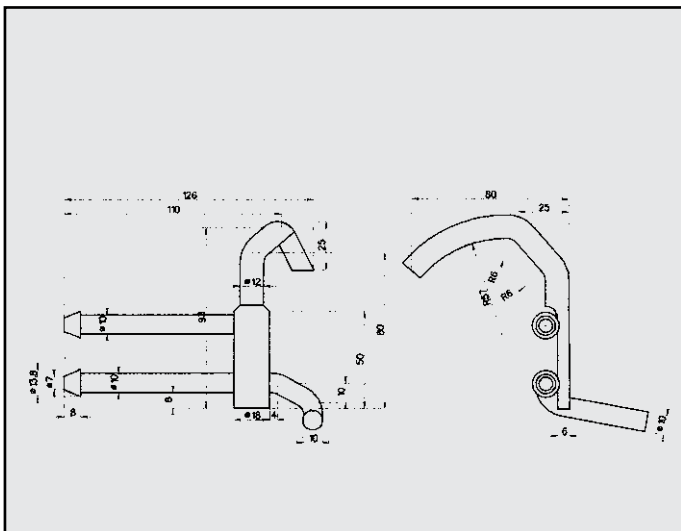
FIAT PALIO 1.2 1.6 ATTACCO POSTERIORE COD. AT 243002
