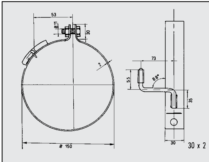
BOSI FASCETTA COD. F 100001
