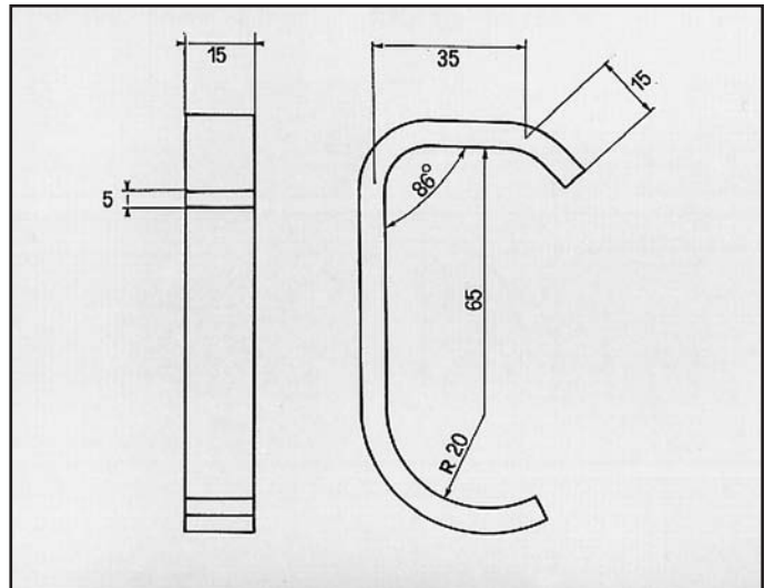
IBIZA DIESEL 1700 ATTACCO COD. AT 680104
