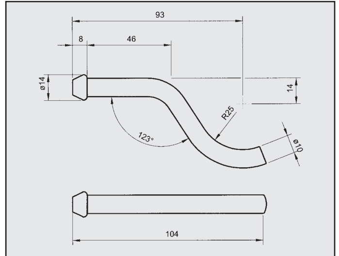
FORD ESCORT ATTACCO COD. AT 260259
