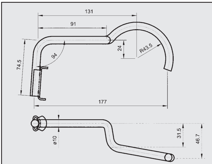
FORD FIESTA 1.8 D CAT ATTACCO posteriore COD. AT 260331
