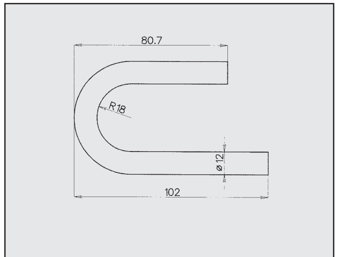
OPEL OMEGA ATTACCO COD. AT 520616
