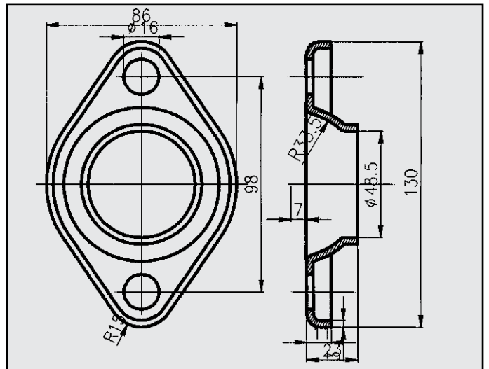
TOYOTA FLANGIA COD. FL 800001
