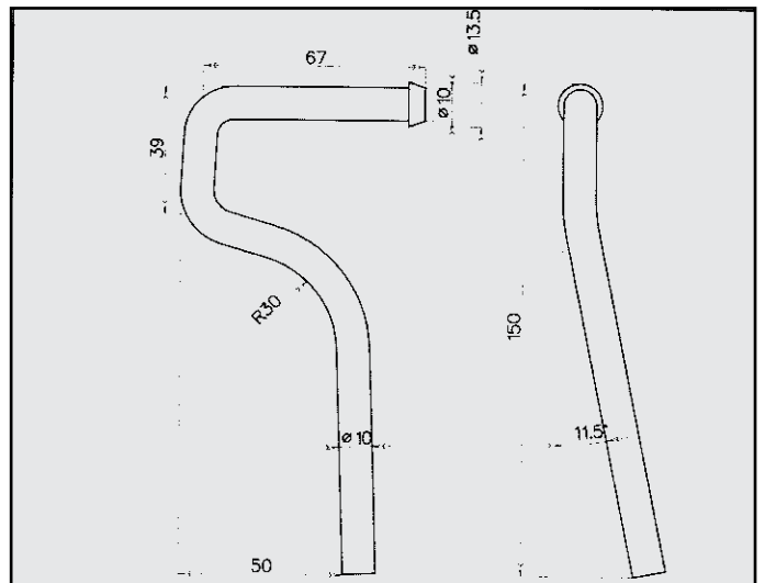
FIAT PALIO 1.2 ATTACCO COD. AT 243006
