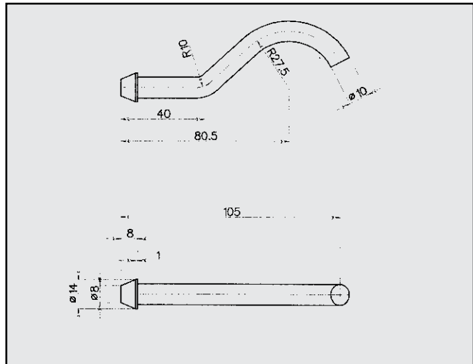
DAEWOO NUBIRA ATTACCO COD. AT 160311
