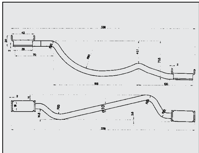
CITROEN XANTIA 1.8-2.0 ATTACCO POSTERIORE COD. AT 141006
