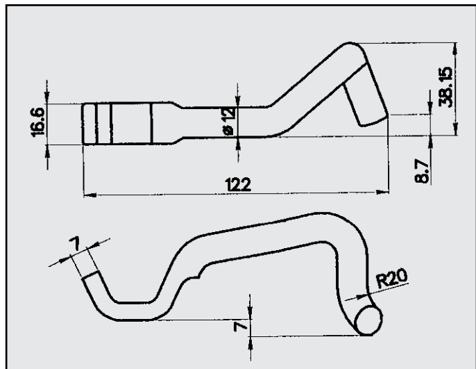
AUDI 100 2.2 ATTACCO COD. AT 040108
