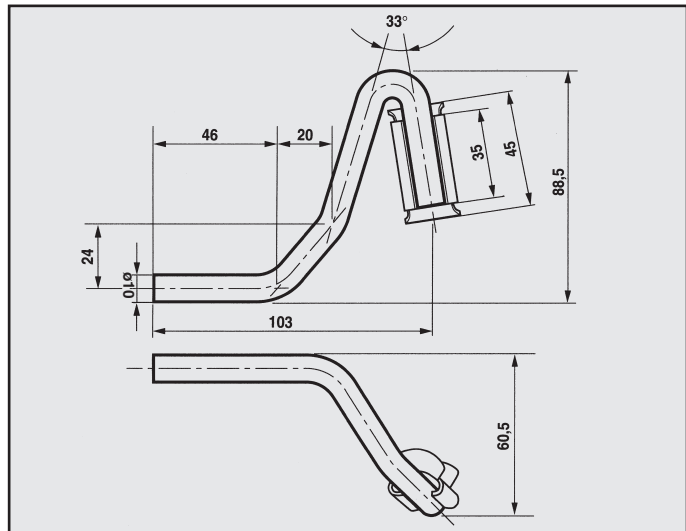
CITROEN ZX 1900 ATTACCO COD. AT 140905 96070794
