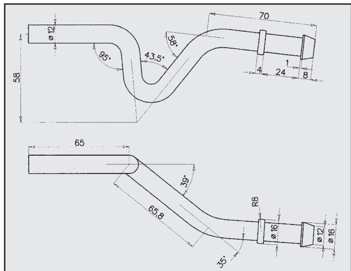
OPEL ATTACCO COD. AT 520018
