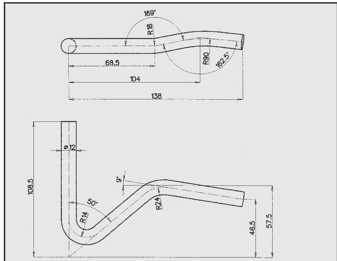
OPEL ASTRA ATTACCO COD. AT 520933/SX
