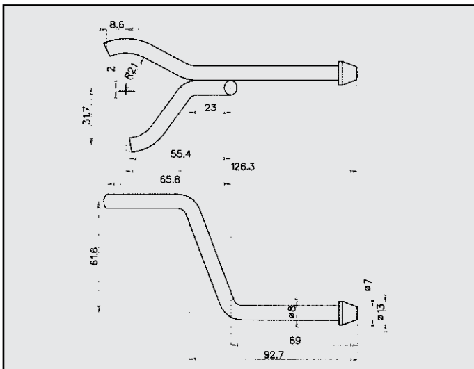
FIAT PANDA 1.1 ATTACCO COD. AT 240117
