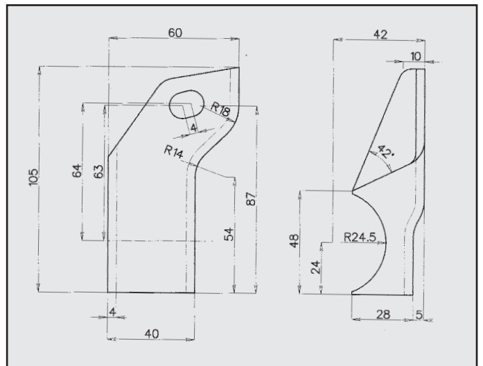
PEUGEOT 206 ATTACCO COD. AT 541215
