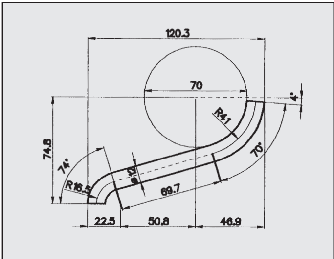
FORD ATTACCO COD. AT 260018
