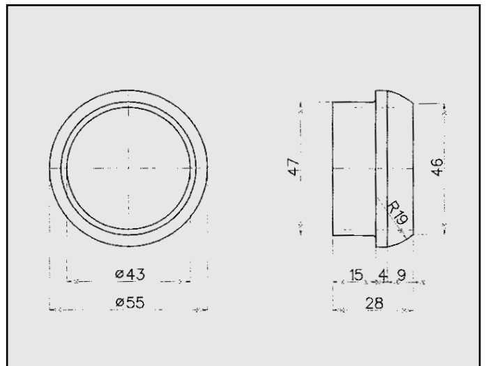
HYUNDAI ANELLO COD. AN 300108
