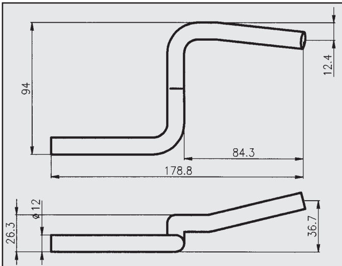
OPEL VECTRA ATTACCO COD. AT 520821
