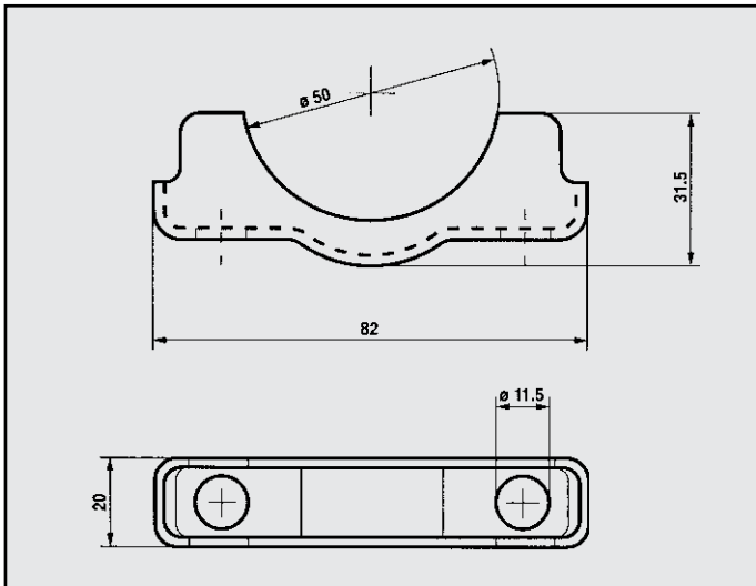
FORD FASCETTA A CAVALLOTO \varnothing 50 COD. F 260001
