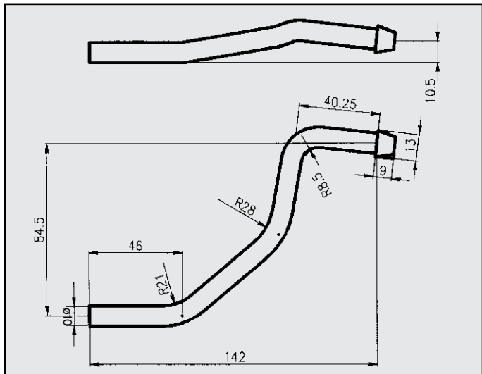
BMW 320 i ATTACCO COD. AT 120402
