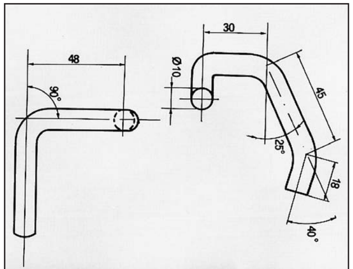
PRELUDE 4 WS ATTACCO COD. AT 280604
