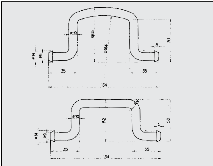
DAEWOO LANOS 1.4/1.6 ATTACCO COD. AT 160201 DX-SX
