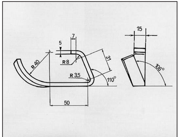
IBIZA ATTACCO sinistro COD. AT 680105
