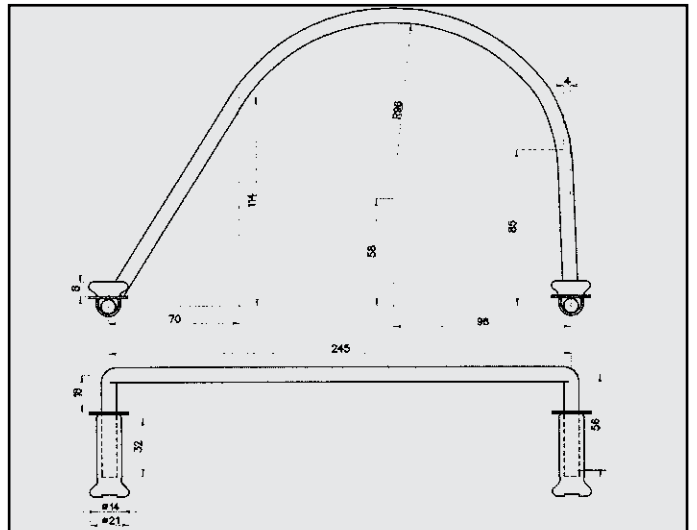
FIAT ULISSE ATTACCO COD. AT 242702
