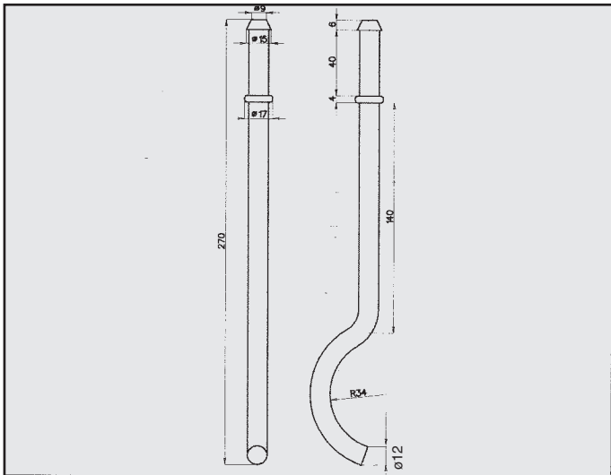
MASERATI ATTACCO COD. AT 400014
