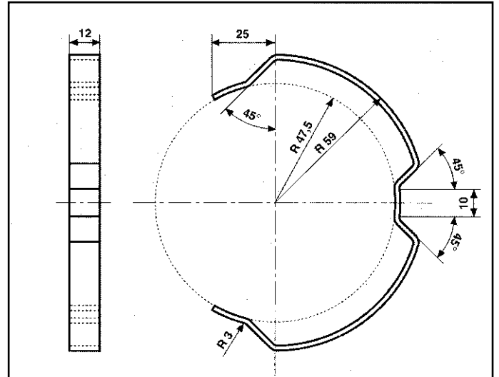
BMW ATTACCO COD. AT 120004
