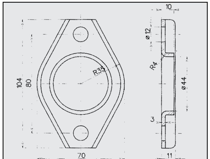
SUZUKI SWIFT FLANGIA COD. FL 720204
