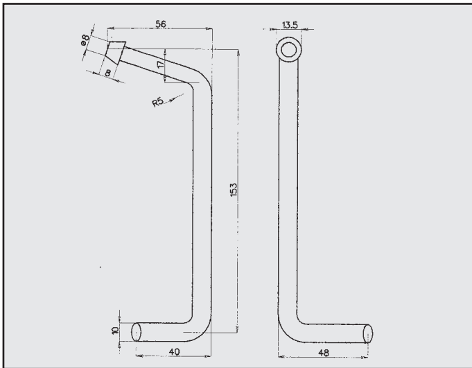
FORD FOCUS ATTACCO COD. AT 261504
