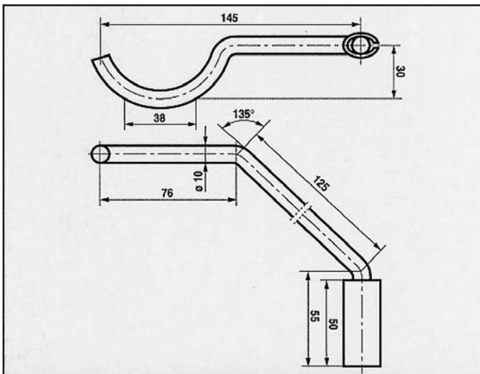
FORD SIERRA 2.0 E ATTACCO COD. AT 260620
