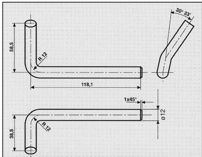
OPEL VECTRA/CALIBRA ATTACCO COD. AT 520810
