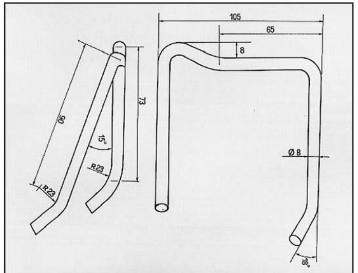
SUPER 5/EXPRESS ATTACCO per centrale COD. AT 600113
