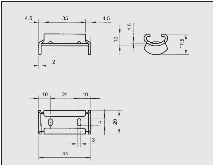
FORD PIASTRINA COD. PI 260102
