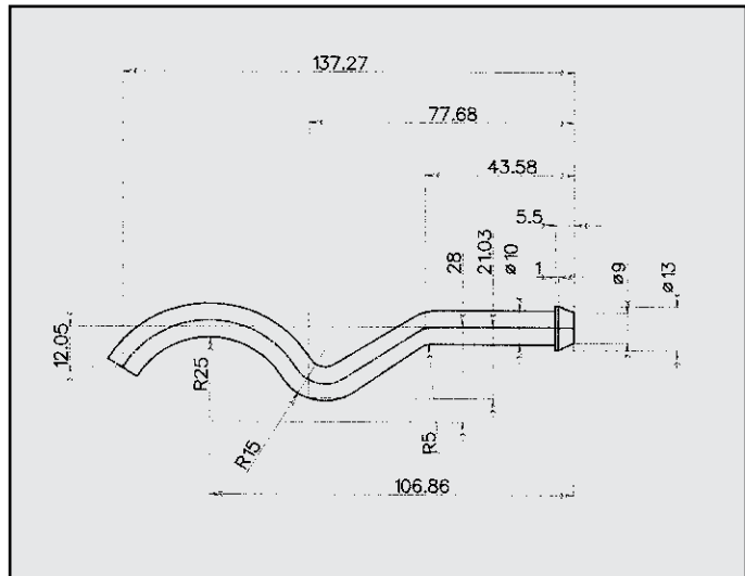
FIAT ATTACCO COD. AT 240013
