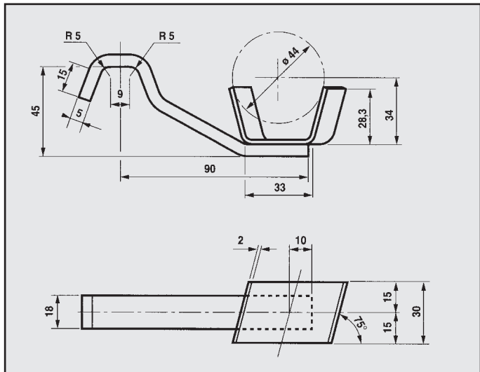
LANCIA DEDRA 1.6 IE ATTACCO COD. AT 380809
