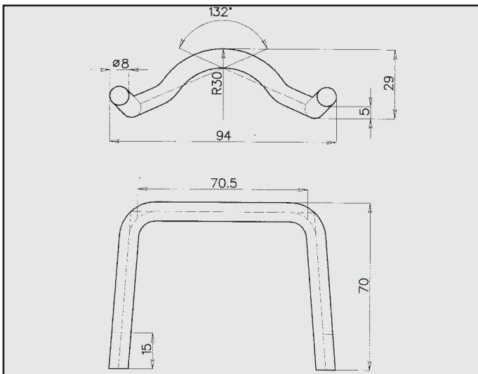
TICO ATTACCO COD. AT 790009
