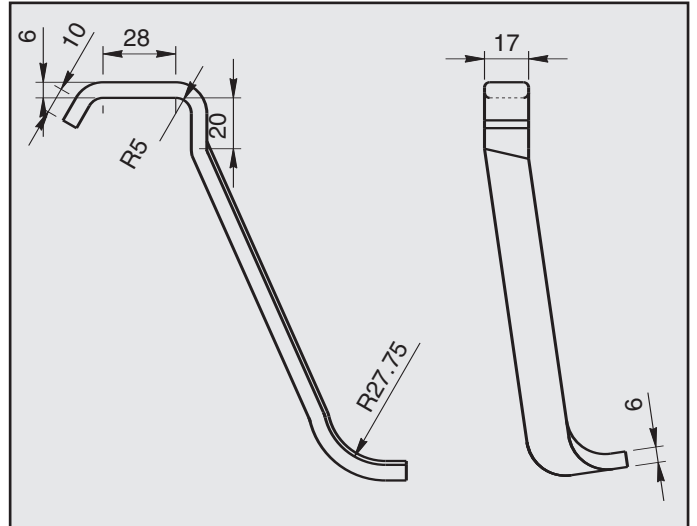
ALFA SPIDER ATTACCO COD. AT 021301
