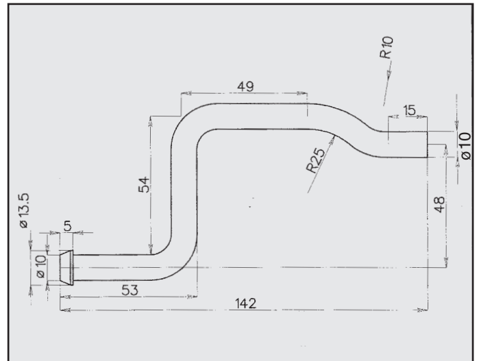
KIA SEPHIA 1.6 ATTACCO COD. AT 310106
