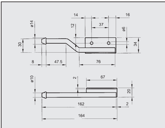
MASERATI ATTACCO COD. AT 400003
