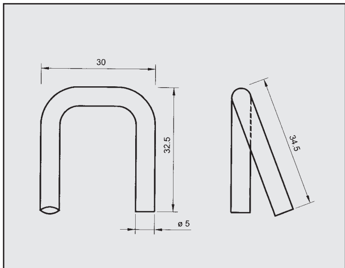
VOLVO 440 "88" ATTACCO COD. AT 880403
