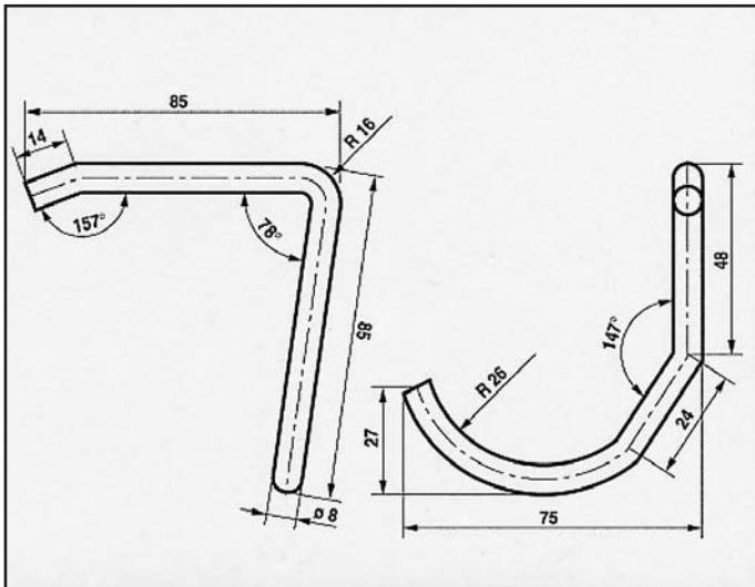
RENAULT R21 2.1 D ATTACCO anteriore COD. AT 601006
