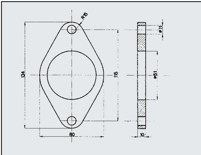
FORD FOCUS FLANGIA COD. FL 261515
