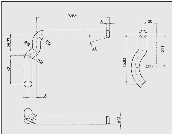
VOLKSWAGEN ATTACCO COD. AT 860033
