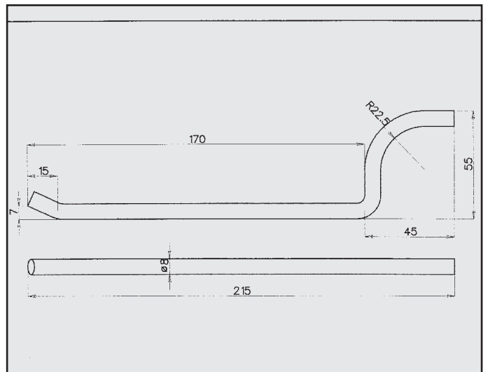
TICO ATTACCO COD. AT 790006
