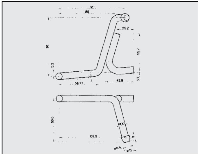
BMW 320 i ATTACCO COD. AT 120403
