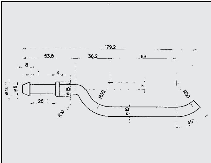
BMW ATTACCO COD. AT 120017
