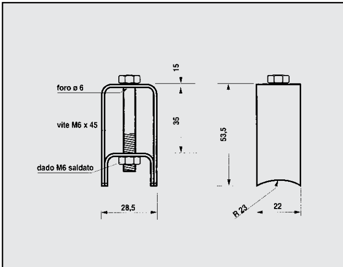
FIAT ATTACCO COD. AT 240001
