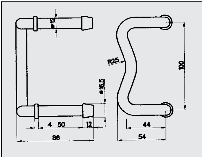
AUDI - VW ATTACCO COD. AT 040002
