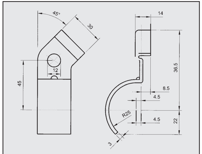
RENAULT 2.5 TD CAT ATTACCO COD. AT 600604
