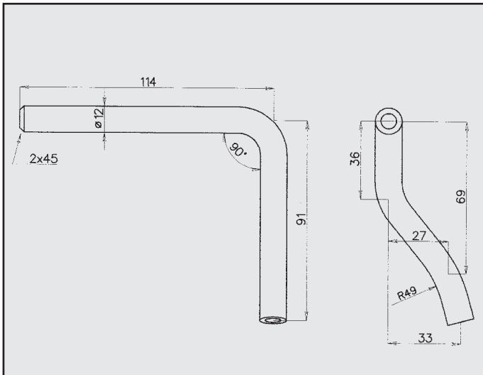
OPEL ATTACCO SX COD. AT 520020
