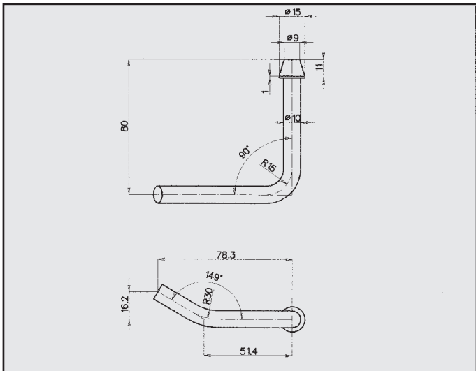
TOYOTA ATTACCO COD. AT 800008
