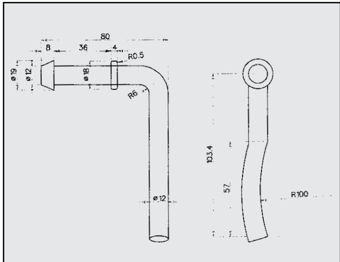
FIAT SCUDO ATTACCO COD. AT 243202
