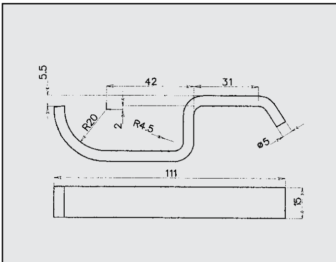
FIAT 600 ATTACCO COD. AT 243103
