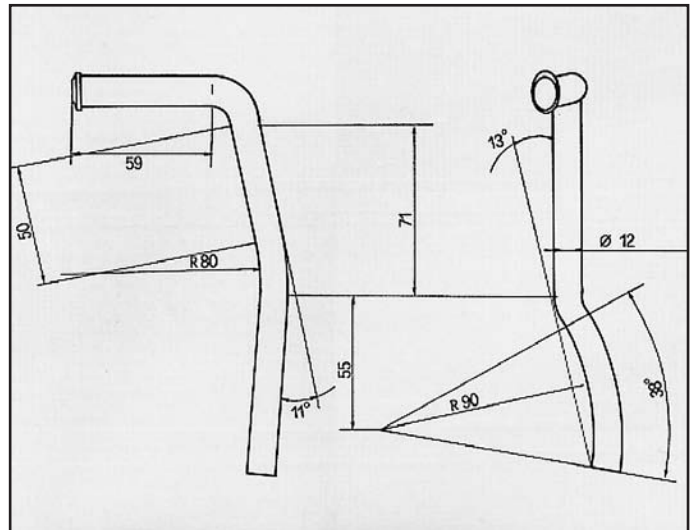
CAMRY ATTACCO COD. AT 800101
