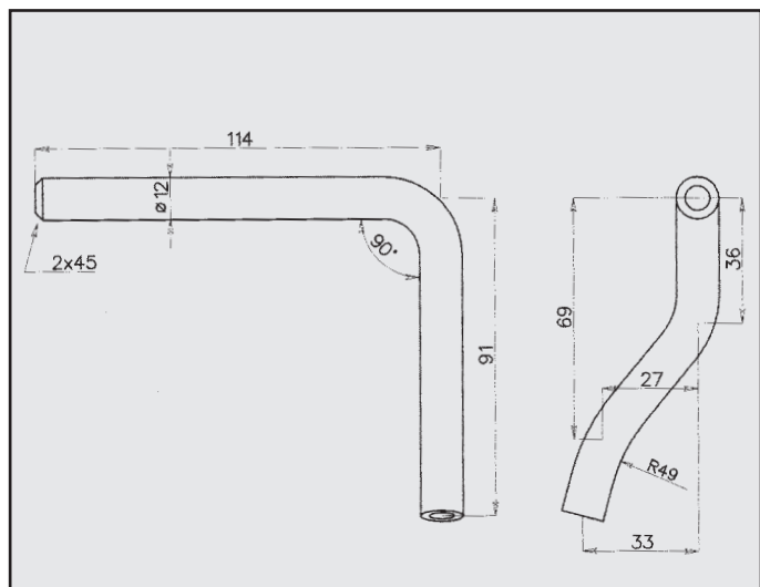
OPEL ATTACCO SX COD. AT 520019
