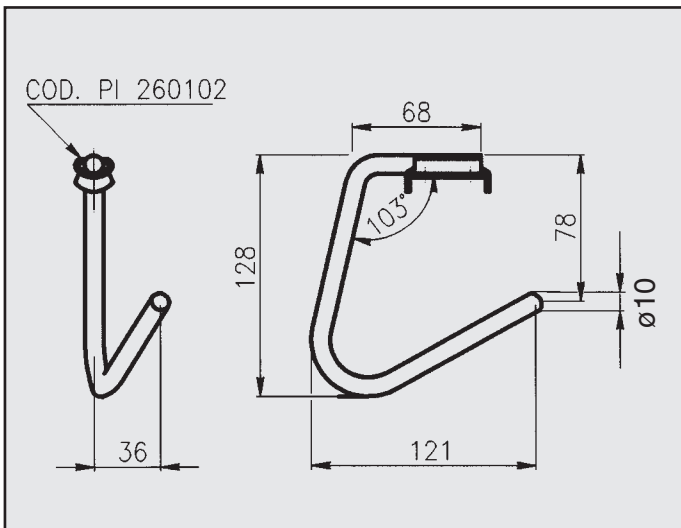
FORD COURIER ATTACCO COD. AT 261303
