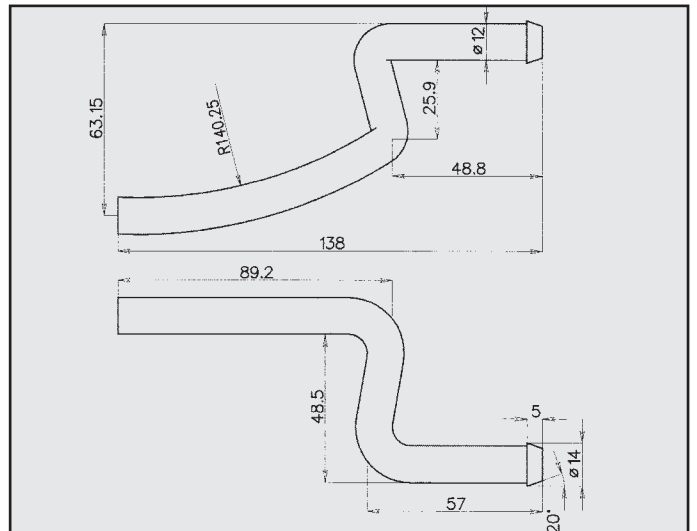
SEAT ATTACCO COD. AT 680005
