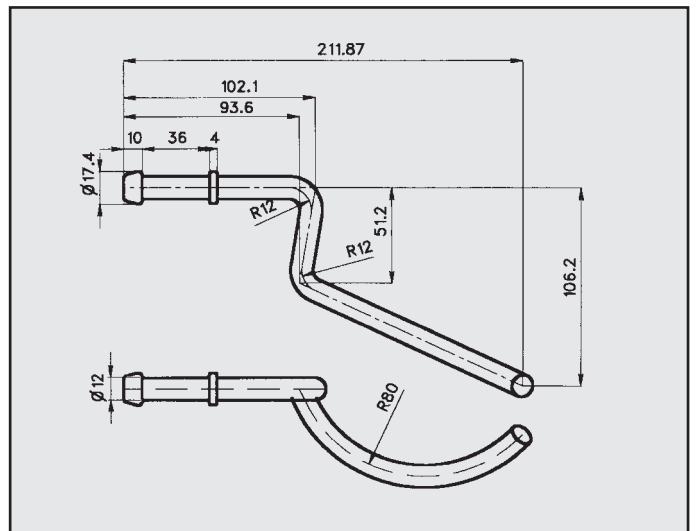
VOLKSWAGEN SHARAN 95 ATTACCO COD. AT 861202
