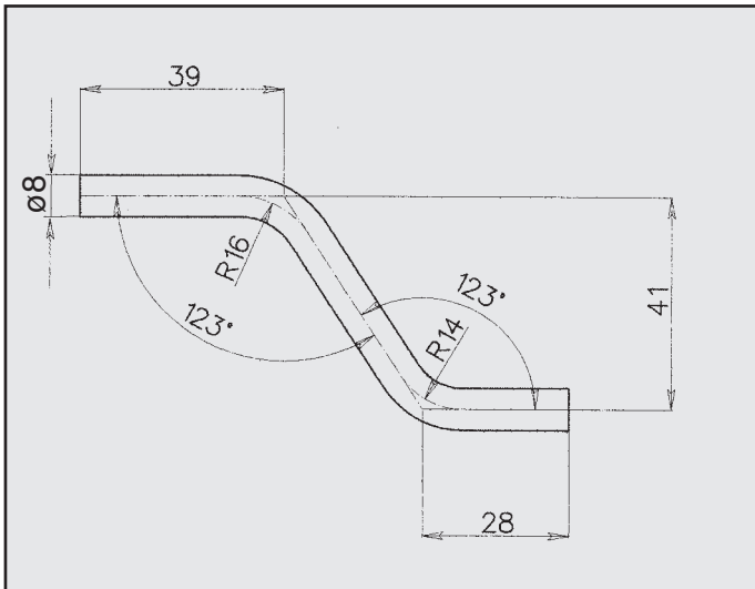
MOTO GUZZI GRISO 571 ATTACCO COD. AT 270202
