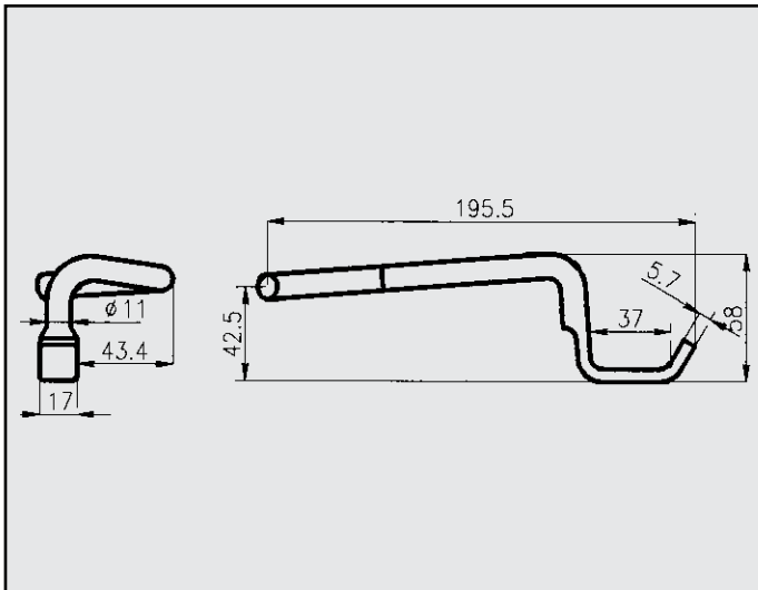
FIAT 600 ATTACCO COD. AT 243101
