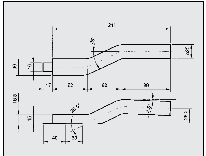
BMW 535 635 ATTACCO COD. AT 120214
