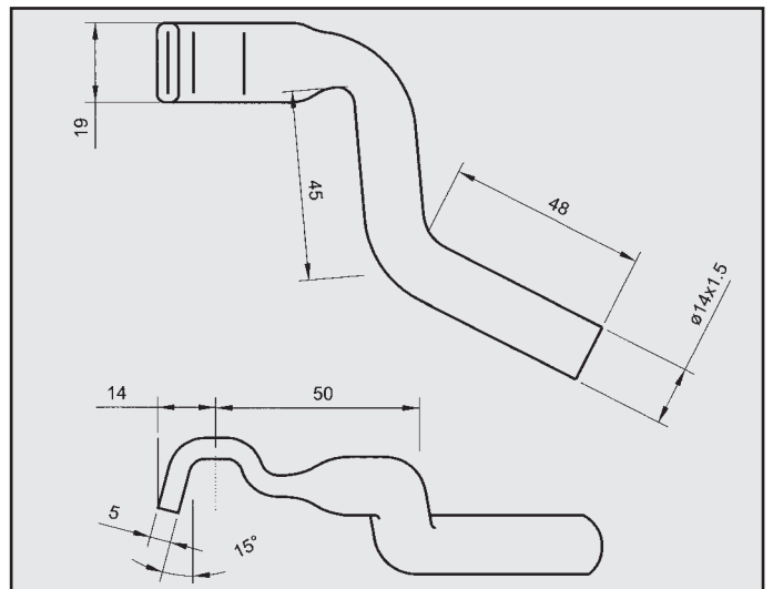
SAAB 900 ATTACCO COD. AT 640203 / AN
