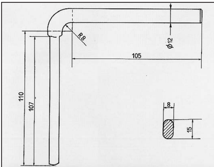
MR II 1600 GT ATTACCO COD. AT 800502
