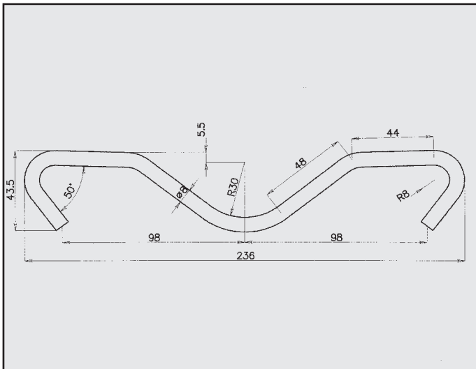
RENAULT MEGANE ATTACCO COD. AT 601607
