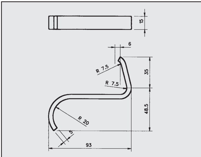
SEAT MARBELLA ATTACCO marmitta posteriore COD. AT 680302
