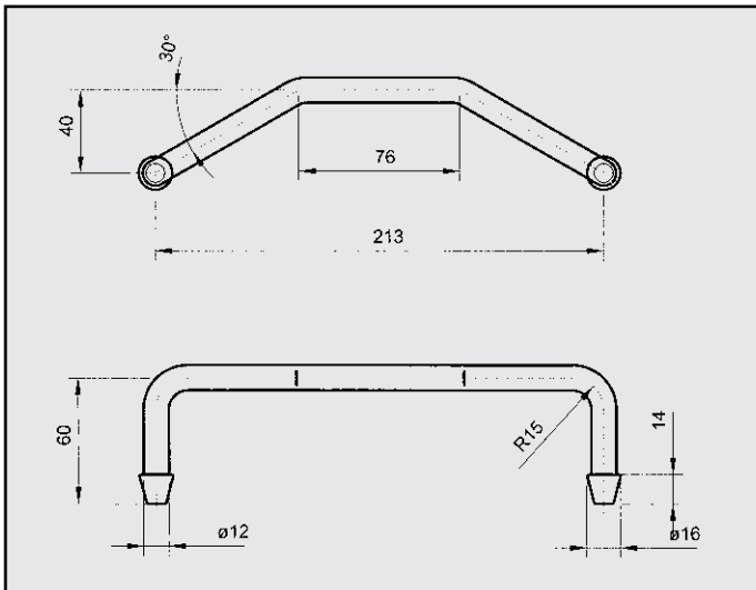
FIAT IVECO S 2000 ATTACCO COD. AT 242501
