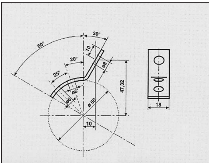
MERCEDES '93 ATTACCO COD. AT 440003
