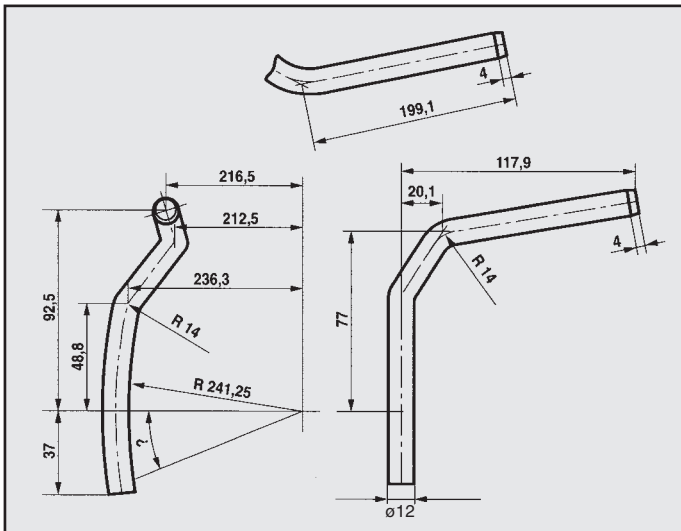
VOLKSWAGEN TRANSPORTER 2.4 D ATTACCO COD. AT 861101
