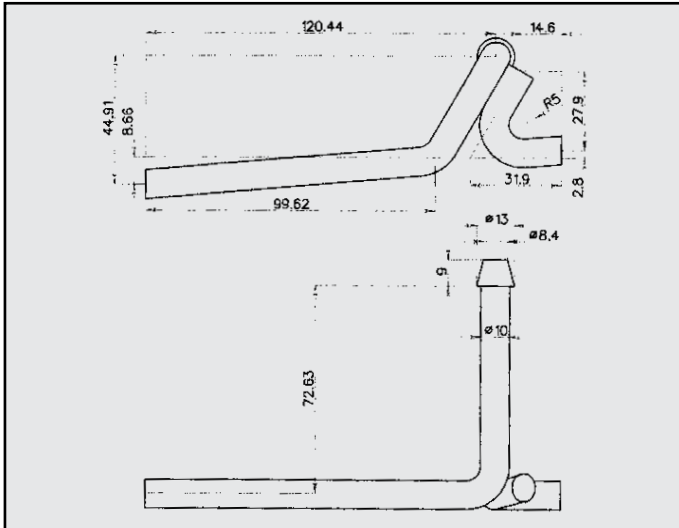
BMW 320I ATTACCO COD. AT 120404
