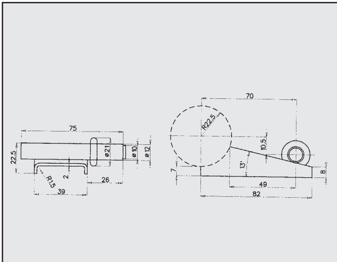
RENAULT CLIO ATTACCO COD. AT 601309
