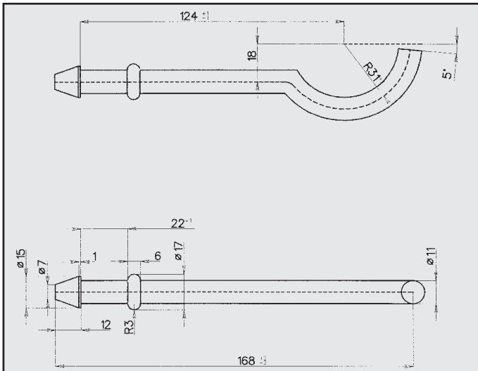
FORD ATTACCO COD. AT 260022
