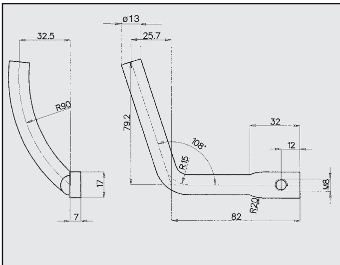
TICO ATTACCO COD. AT 790007
