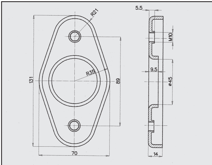
OPEL KADETT FLANGIA COD. FL 520114
