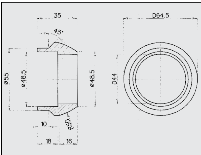
HYUNDAI ANELLO COD. AN 300001
