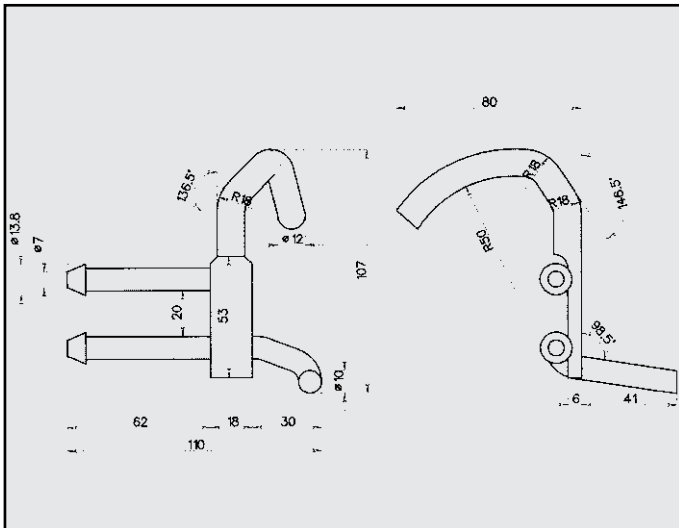
FIAT DOBLO' ATTACCO COD. AT 243407
