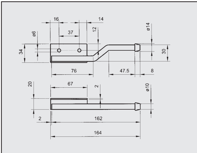
MASERATI ATTACCO COD. AT 400002
