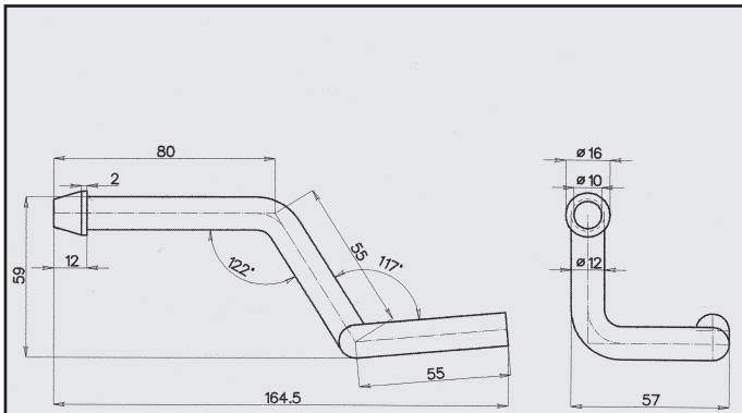
ALFA 156 1.6/1.8/2.0 DADO COD. AT 021208
