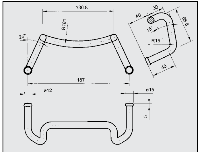
FIAT IVECO S 2000 STAFFA POSTERIORE COD. AT 242503
