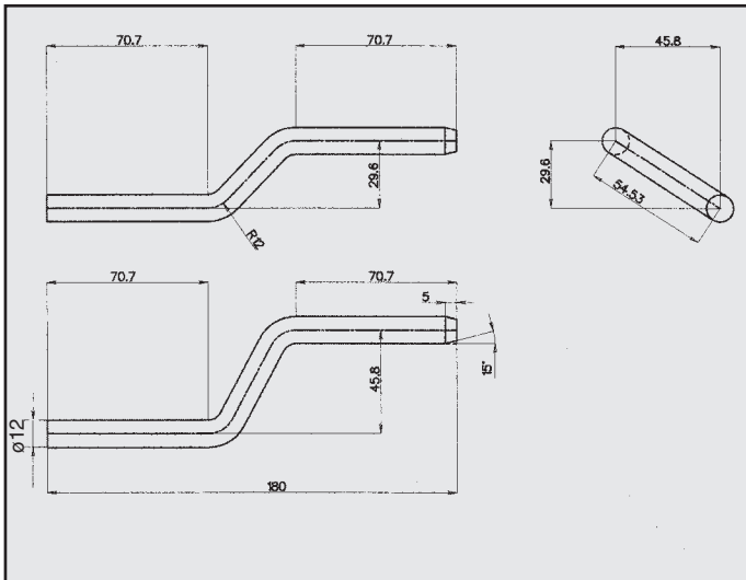
MERCEDES ATTACCO COD. AT 440001
