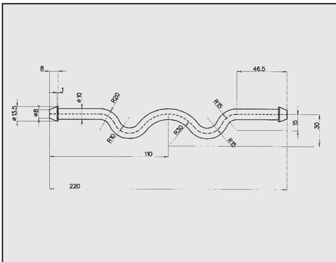
FORD FOCUS 1.6 ATTACCO COD. AT 261511
