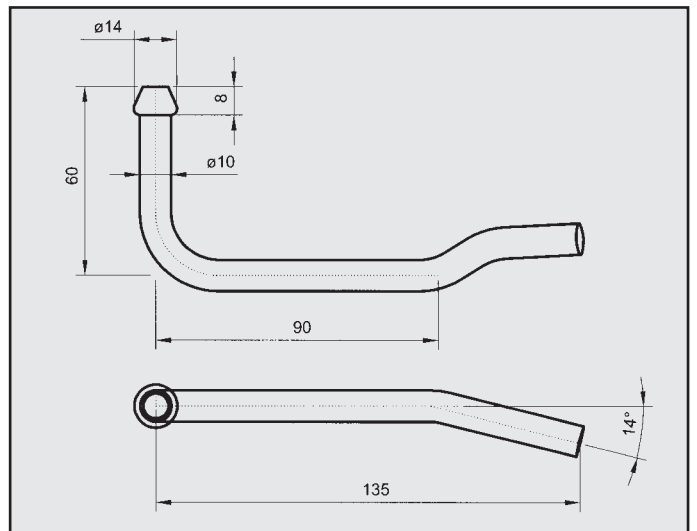
NISSAN PRIMERA 2.0 SLX ATTACCO COD. AT 500406
