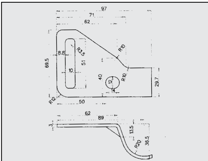
DACIA ATTACCO COD. AT 150003
