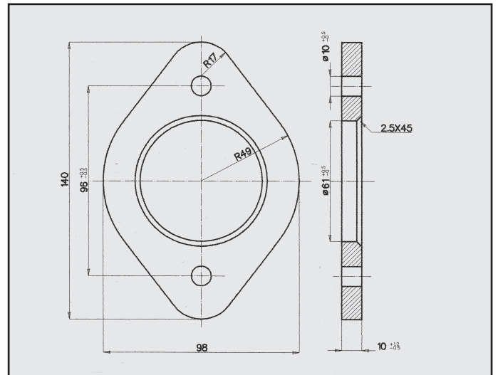
OPEL VECTRA FLANGIA COD. FL 520834
