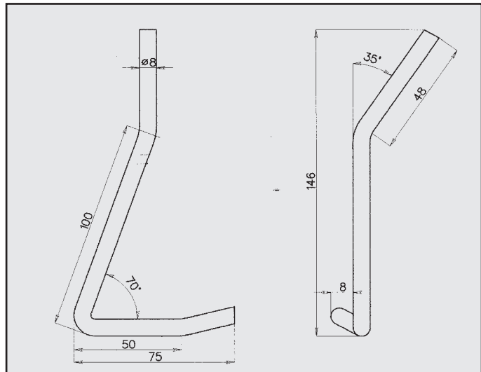
PEUGEOT 104 ZS ATTACCO COD. AT 540203
