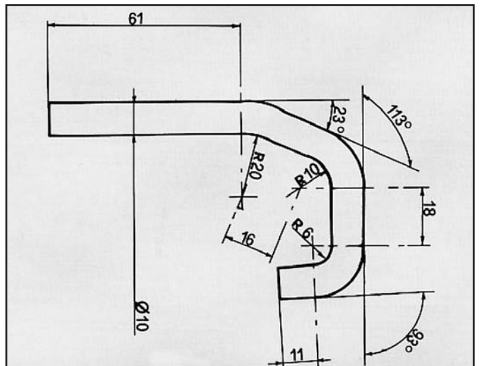
CIVIC 1300/1500 ATTACCO COD. AT 280406
