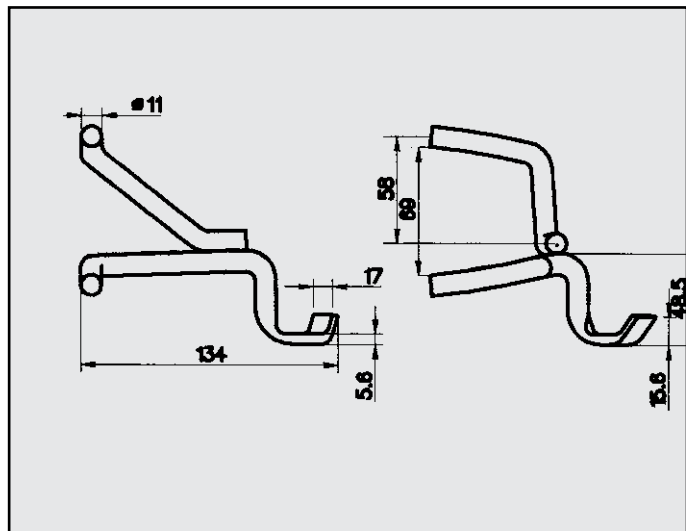
FIAT 600 ATTACCO COD. AT 243106
