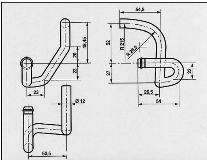
SEAT CORDOBA ATTACCO COD. AT 680601
