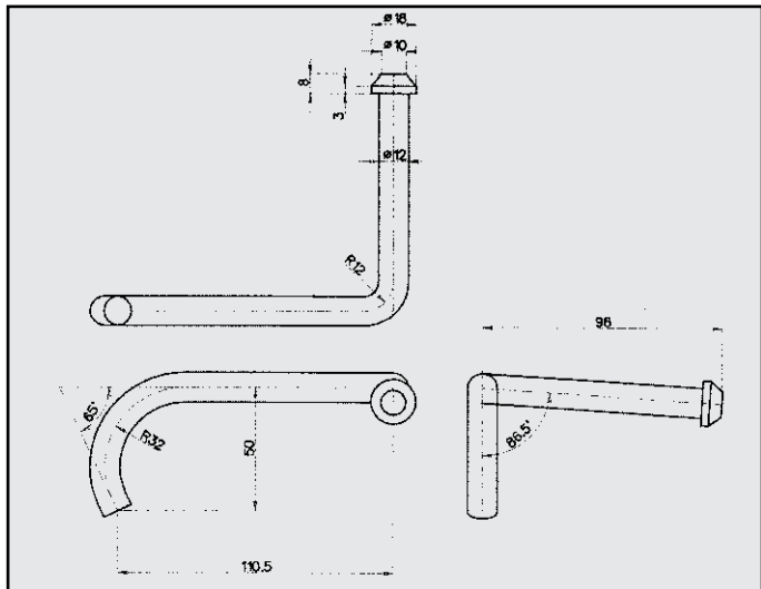
FIAT SCUDO ATTACCO COD. AT 243204
