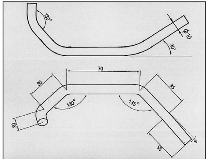
CRX ATTACCO COD. AT 280506
