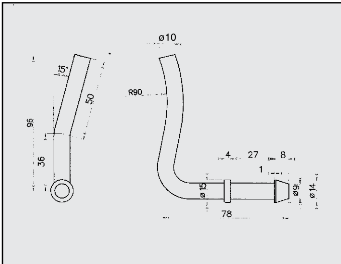
BMW 318 TE ATTACCO COD. AT 120601
