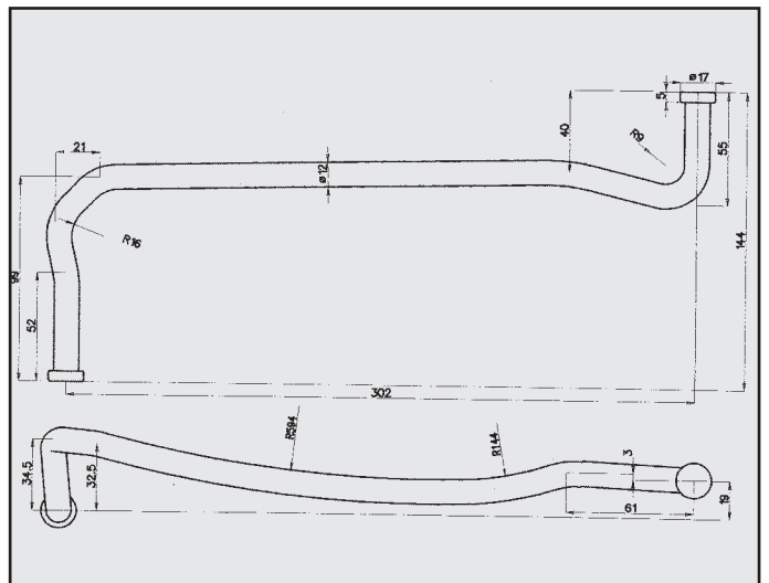
TOYOTA CAMRY ATTACCO COD. AT 800109
