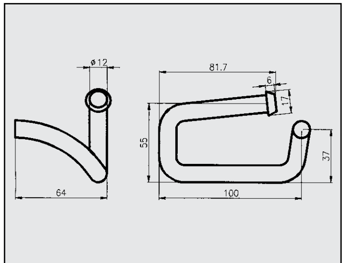
FIAT ULISSE ATTACCO COD. AT 242705
