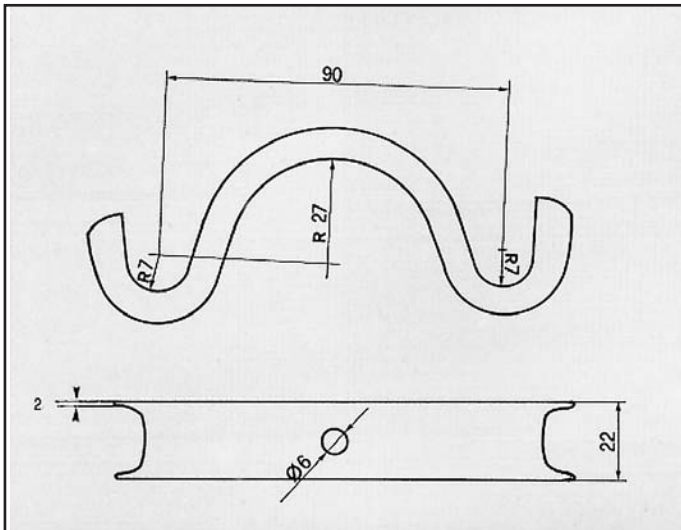
JETTA 1100/1300/1500/1600 D/1600 TD ATTACCO per posteriore COD. AT 860401
