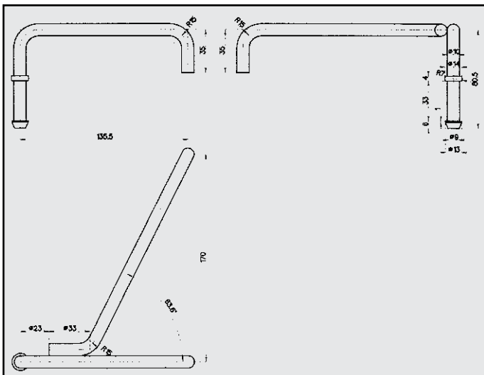
BMW ATTACCO COD. AT 120022
