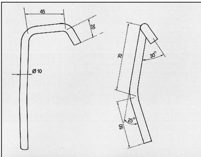
NEW CITY 1.3 ATTACCO COD. AT 280801
