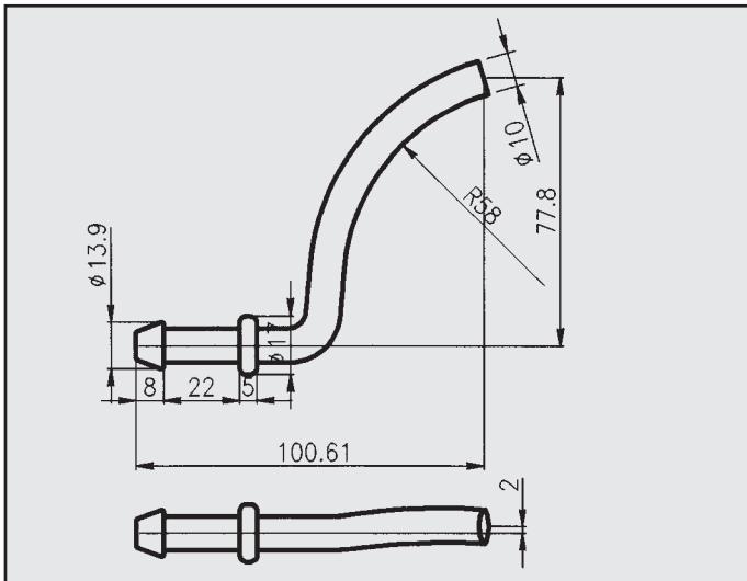
FORD ESCORT ATTACCO COD. AT 260272/DX
