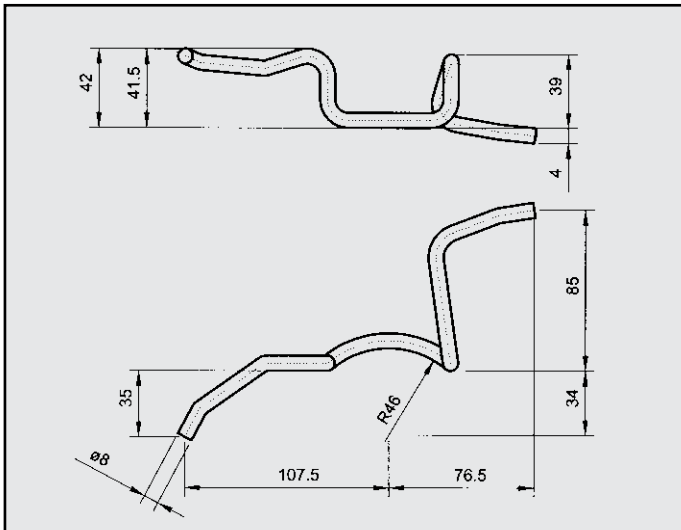
CITROEN C15 ATTACCO COD. AT 140001
