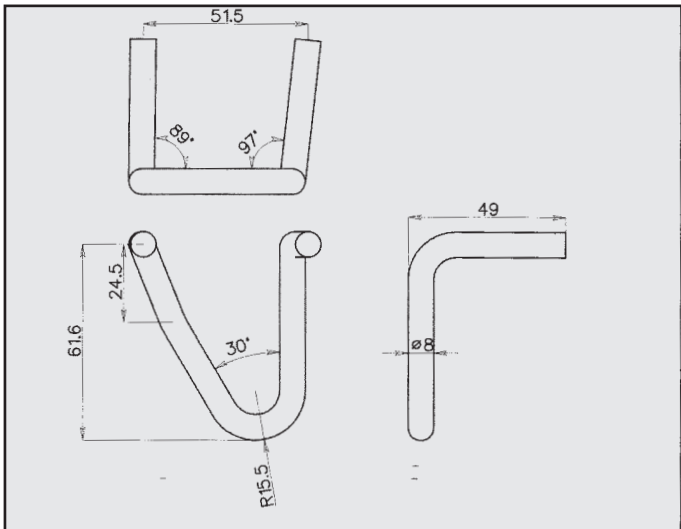
RENAULT CLIO ATTACCO COD. AT 601303
