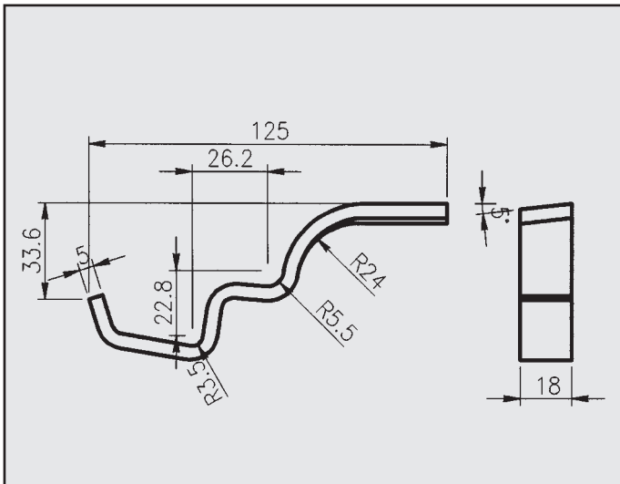
VOLVO 850 TDI ATTACCO COD. AT 880803
