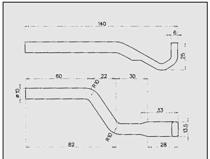
FIAT MAREA ATTACCO COD. AT 242813
