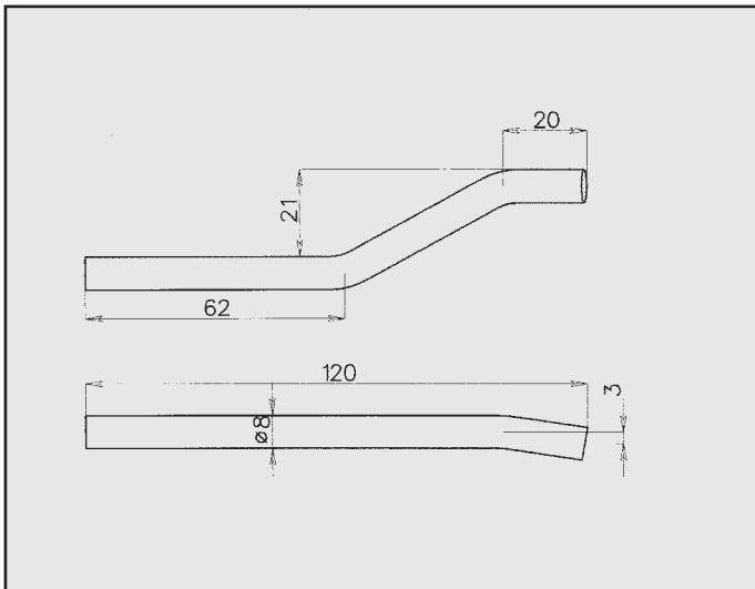
MICROCAR ATTACCO COD. AT 450102
