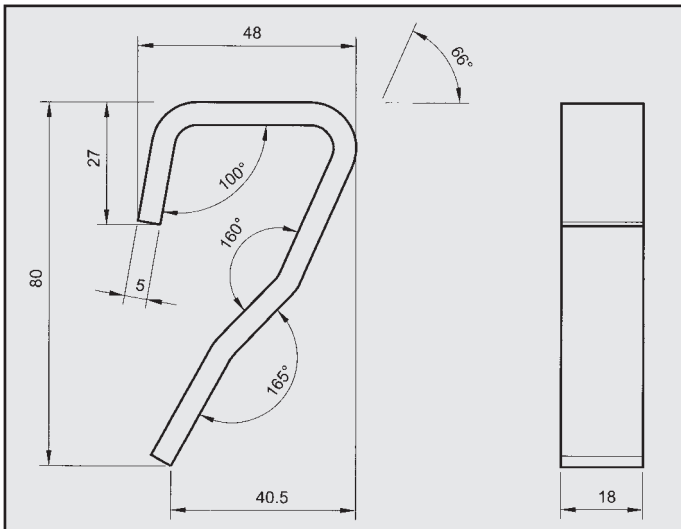
OPEL KADETT ATTACCO COD. AT 520109
