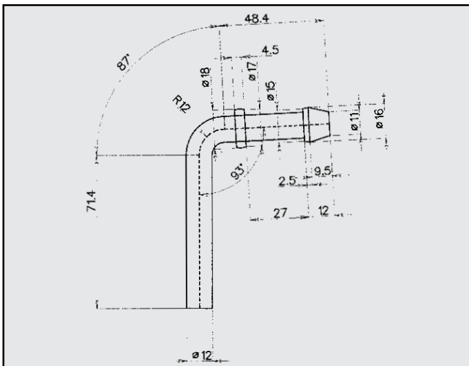
FIAT ATTACCO COD. AT 240011
