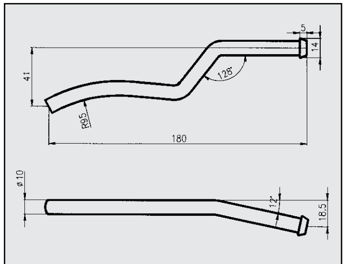
FIAT BRAVO/BRAVA ATTACCO COD. AT 242318
