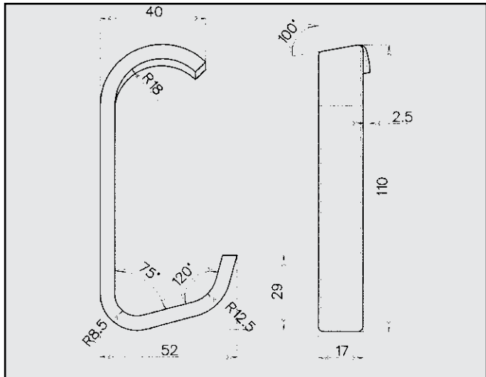
FIAT PANDA ATTACCO COD. AT 240118
