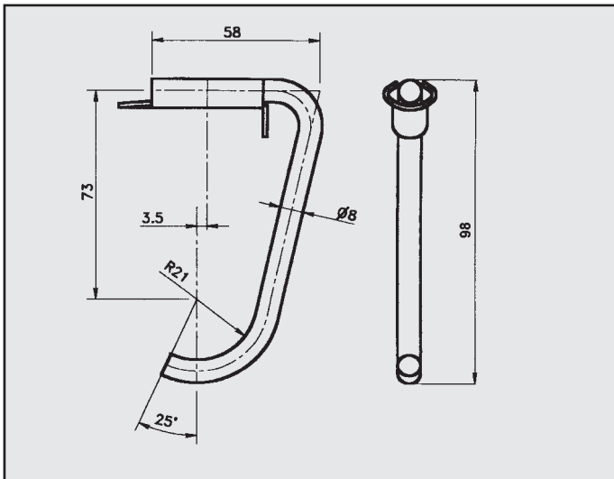
OPEL ASTRA 1/90 ATTACCO COD. AT 520902
