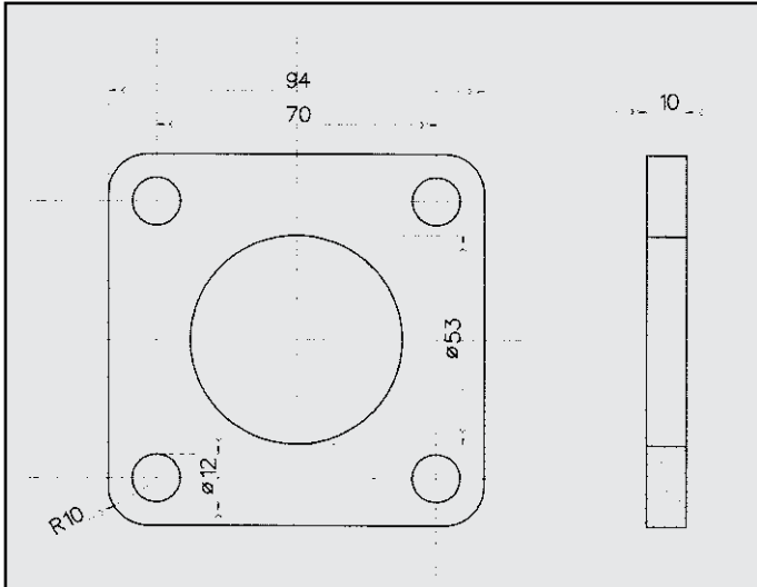
VOLKSWAGEN GOLF FLANGIA COD. FL 860125
