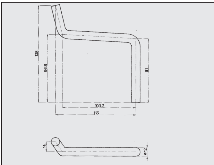
RENAULT CLIO ATTACCO COD. AT 601321
