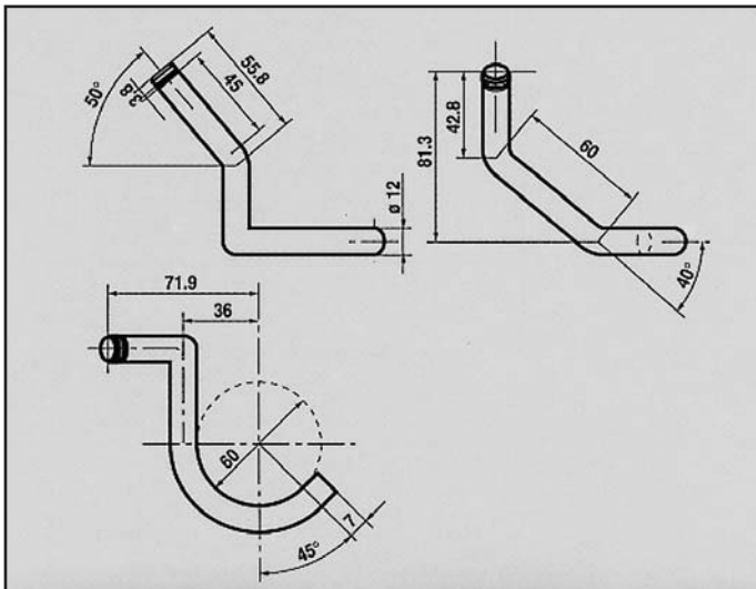
OPEL VECTRA 2000 E ATTACCO COD. AT 520806
