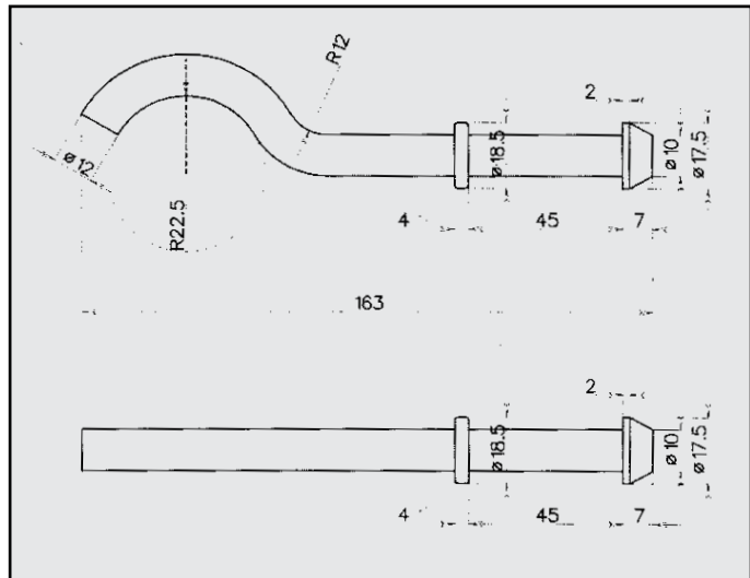
CITROEN C2 ATTACCO COD. AT 141501
