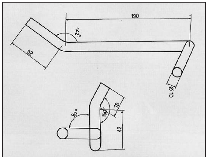
OMEGA 2000 ATTACCO COD. AT 520603
