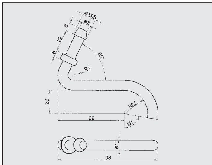
FORD FIESTA ATTACCO COD. AT 260357
