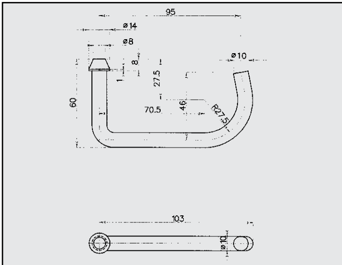
DAEWOO NUBIRA 1.6 ATTACCO COD. AT 160307
