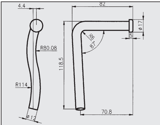
OPEL OMEGA ATTACCO COD. AT 520613
