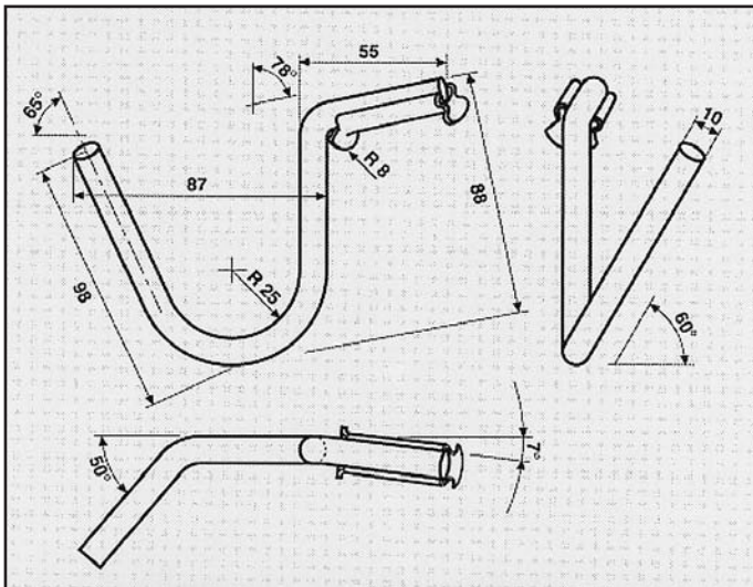
FORD SIERRA 1800 ATTACCO posteriore COD. AT 260619
