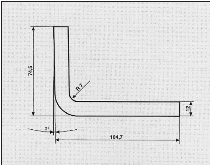
OPEL ASTRA 1700 DIESEL S.W. ATTACCO centrale COD. AT 520901
