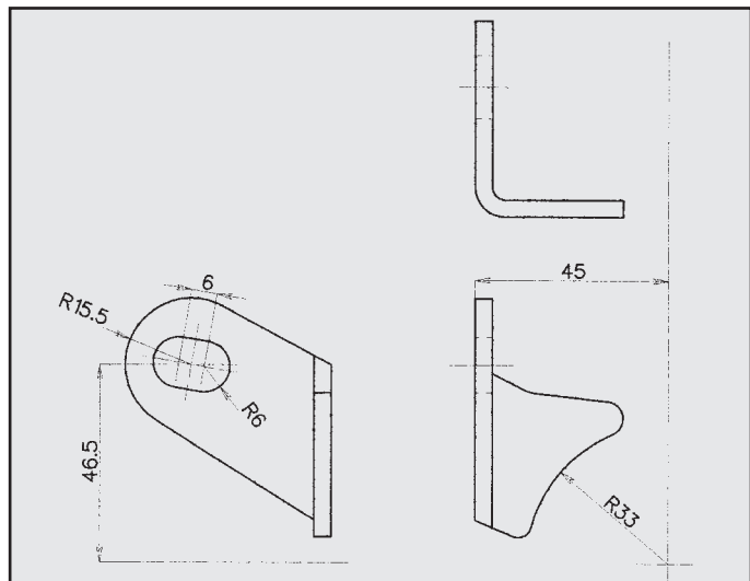
PEUGEOT 205 ATTACCO COD. AT 540322
