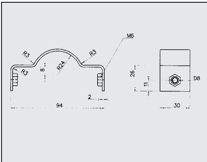
FIAT MULTIPLA ATTACCO COD. AT 242612
