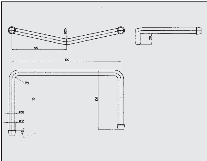
ROVER 75 ATTACCO COD. AT 621201
