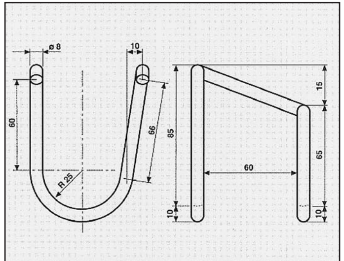
RENAULT 21 1.4/1.7/2.0/2.0i/2.1D/2.1 TD 3 volumi 05/89 NEVADA 1.4/1.7/2.0/2.1D/2.7TD/06/86 COD. AT 601003 ATTACCO posteriore 7700768594
