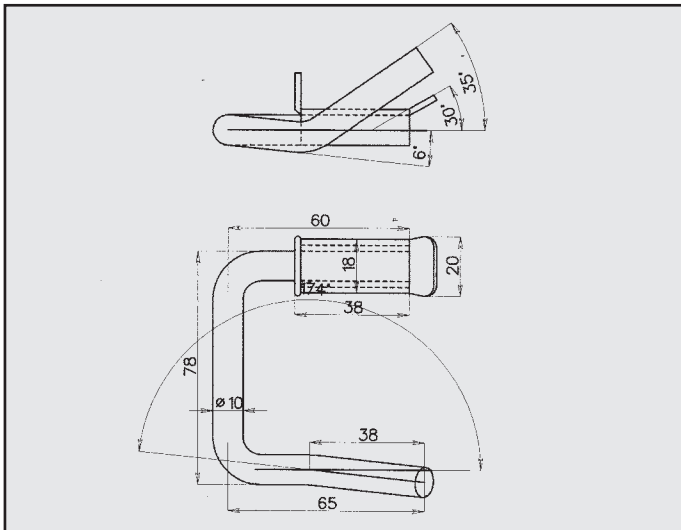
OPEL KADETT ATTACCO COD. AT 520108
