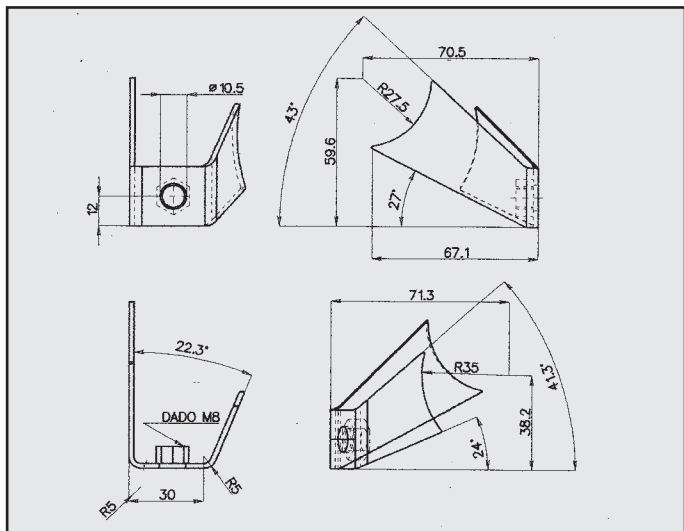
RENAULT CLIO ATTACCO COD. AT 601316
