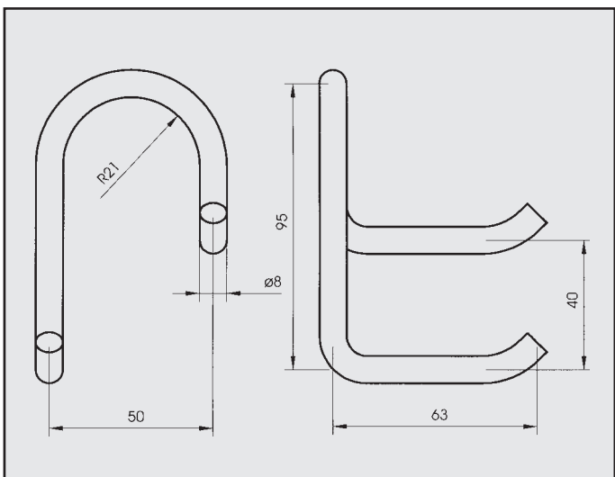
RENAULT ATTACCO COD. AT 600003
