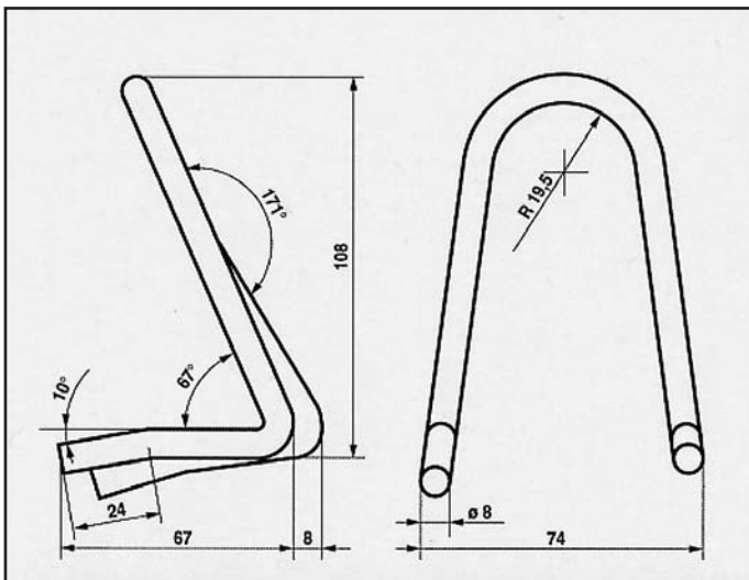
SEAT TERRA ATTACCO posteriore COD. AT 680403
