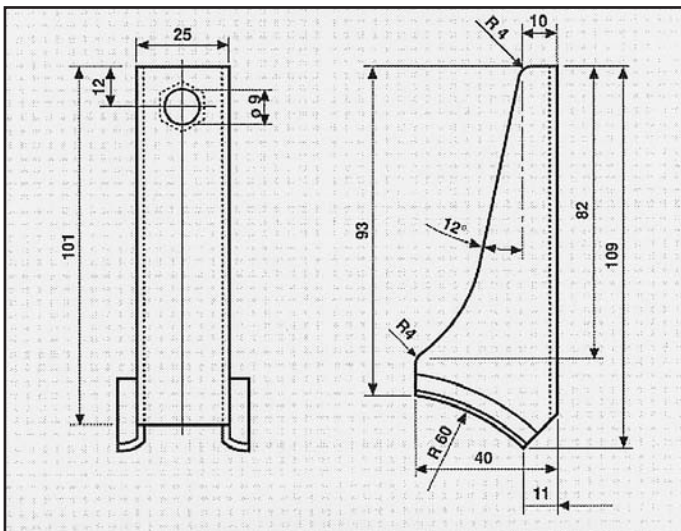
SUZUKI VITARA ATTACCO marmitta posteriore COD. AT 720103
