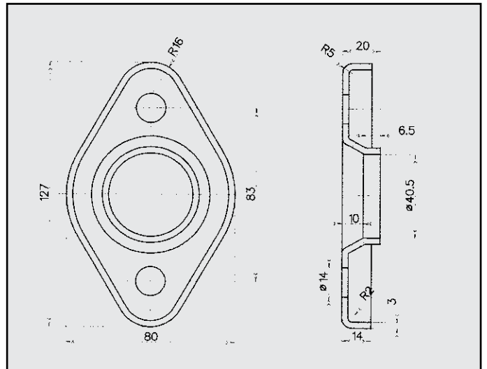
TOYOTA YARIS 1.0 16V FLANGIA COD. FL 801203
