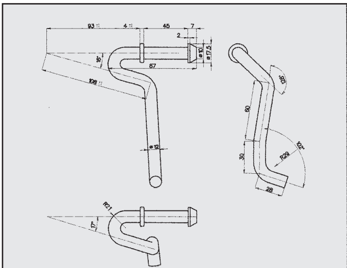
OPEL ATTACCO COD. AT 520022
