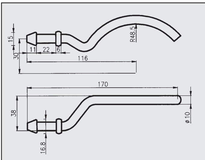
FORD FIESTA ATTACCO COD. AT 260352
