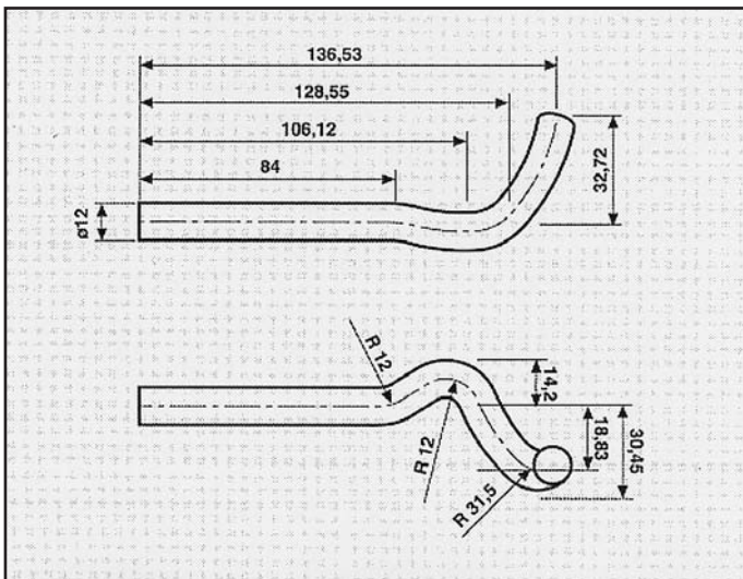
VOLKSWAGEN BUS T4/93 ATTACCO COD. AT 860601
