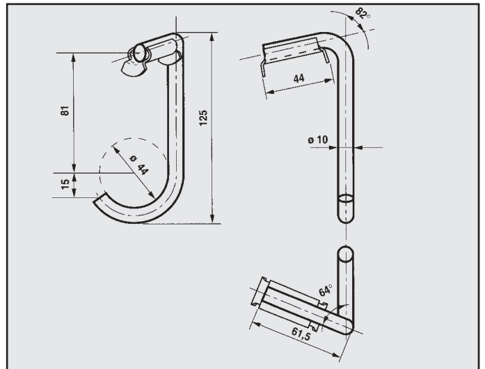
FORD ESCORT 1.8 D ATTACCO COD. AT 260251
