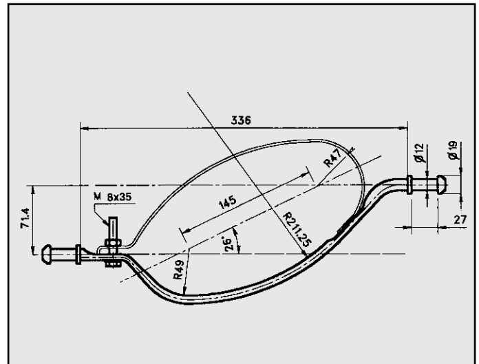
CHRYSLER VOYAGER FASCETTA COD. F 130101
