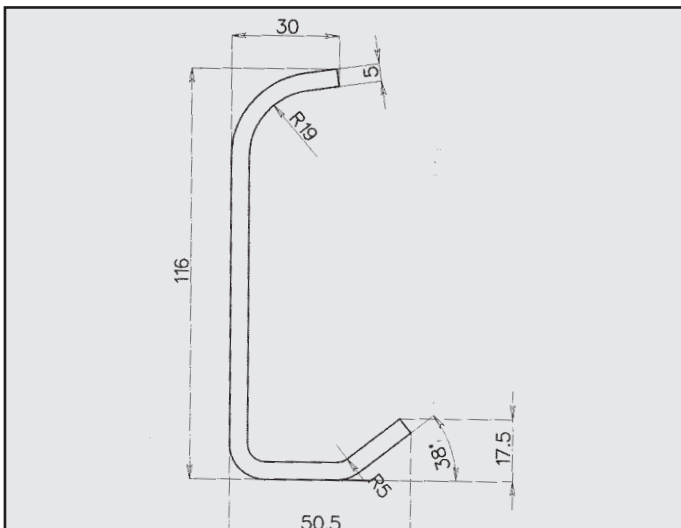
LANCIA Y 10 FIRE ATTACCO COD. AT 381003
