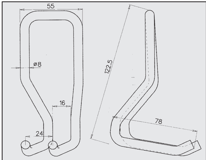
LANCIA DELTA ATTACCO COD. AT 380338
