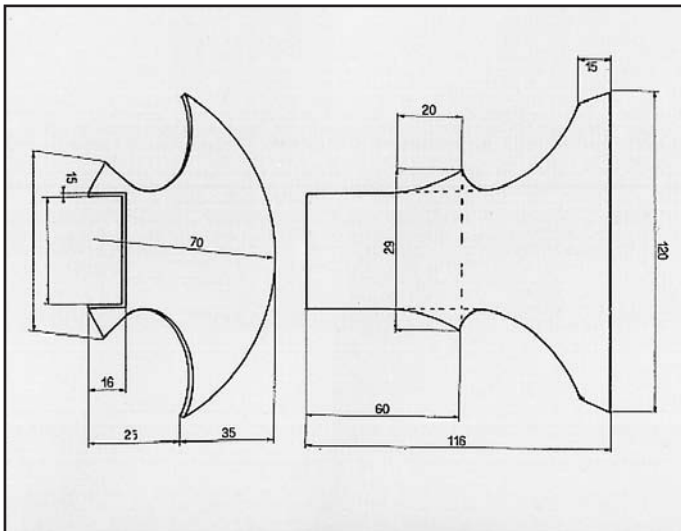
TALBOT 1307 ATTACCO COD. AT 780102 0049138807 0049309007 48036Z 48224A
