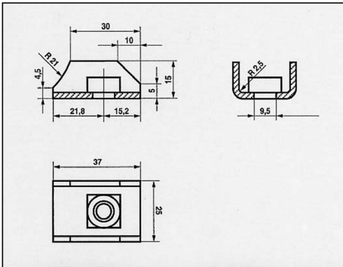
VOLKSWAGEN SYNCRO VR6 ATTACCO COD. AT 860801
