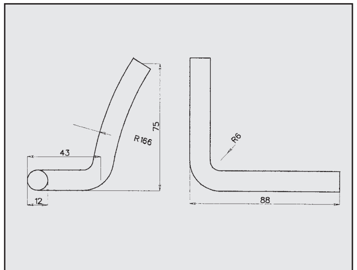
SEAT AROSA ATTACCO COD. AT 680803
