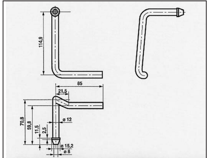
FORD TRANSIT ATTACCO COD. AT 261004
