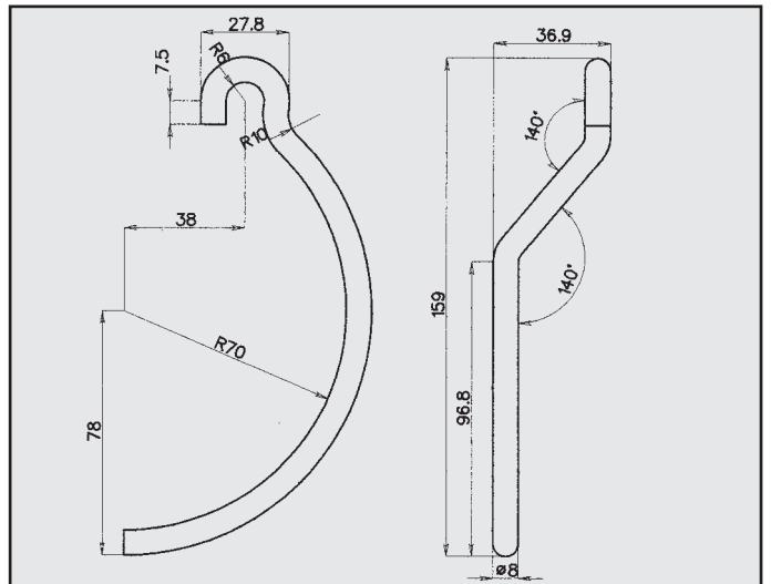
OPEL ATTACCO DX COD. AT 520025/DX
