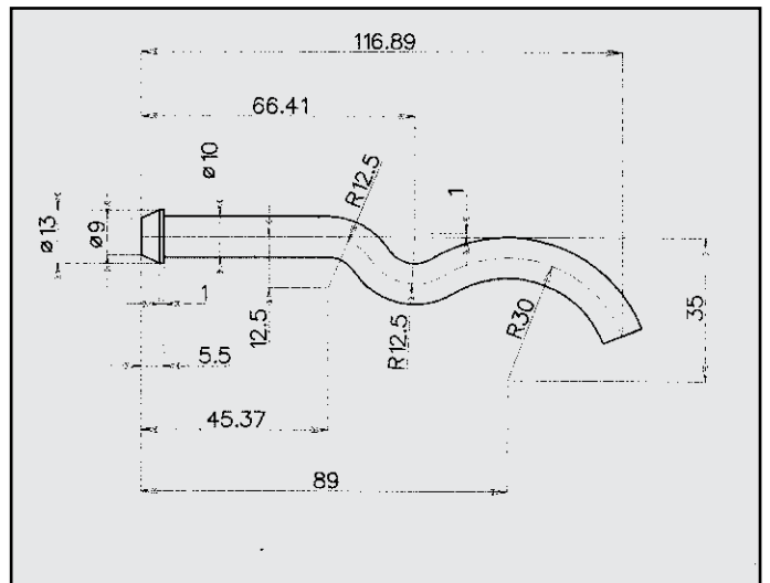
FIAT ATTACCO COD. AT 240020
