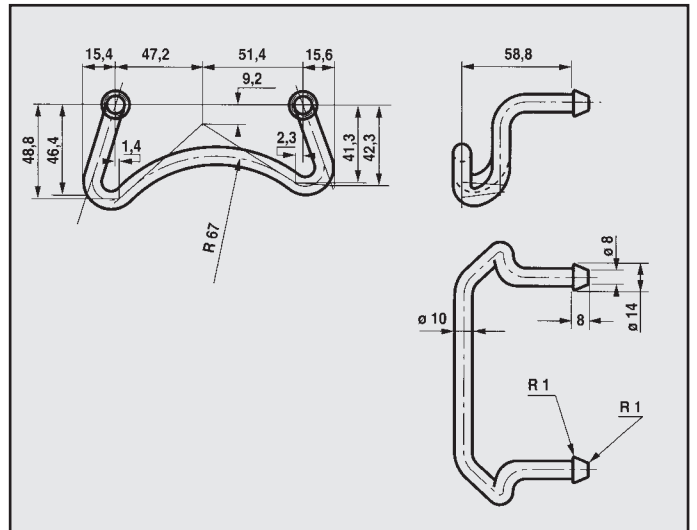
FORD SCORPIO 1995 ATTACCO COD. AT 260814
