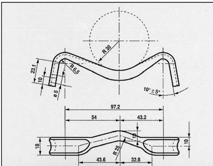
OPEL VECTRA 2000 E ATTACCO COD. AT 520807
