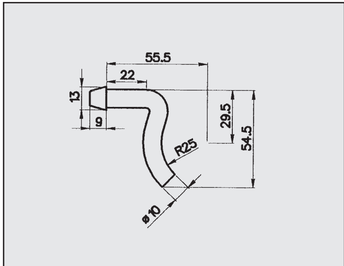
FORD ATTACCO COD. AT 260019
