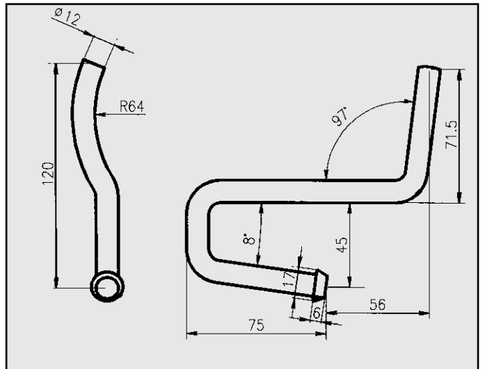
FIAT ULISSE ATTACCO COD. AT 242704
