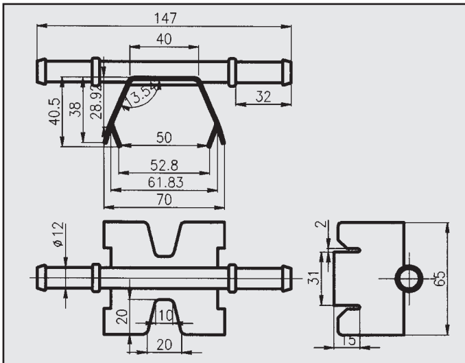
SKODA OCTAVIA ATTACCO COD. AT 690201
