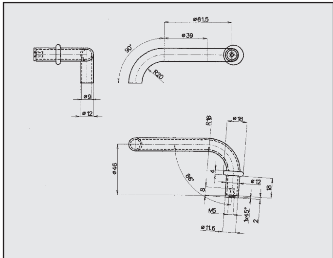
RENAULT CLIO ATTACCO COD. AT 601313
