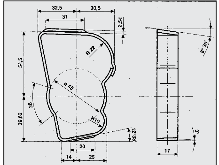
BMW ATTACCO COD. AT 120005
