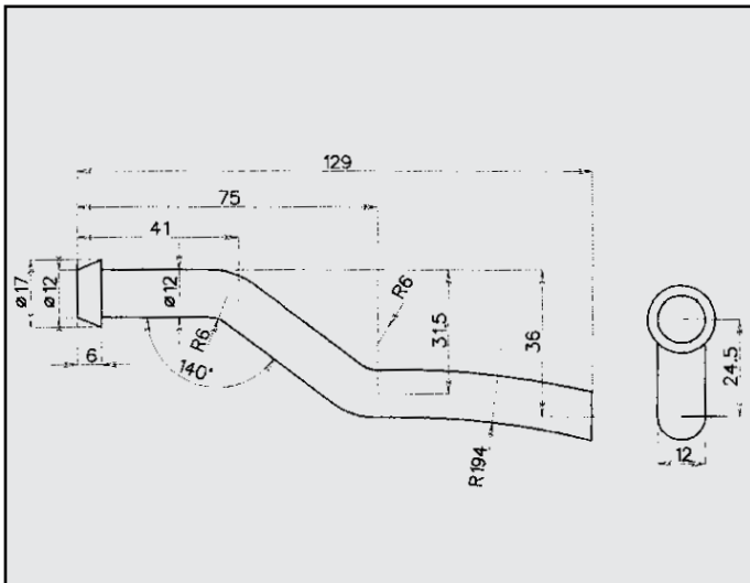
DAEWOO MATIZ ATTACCO COD. AT 160102
