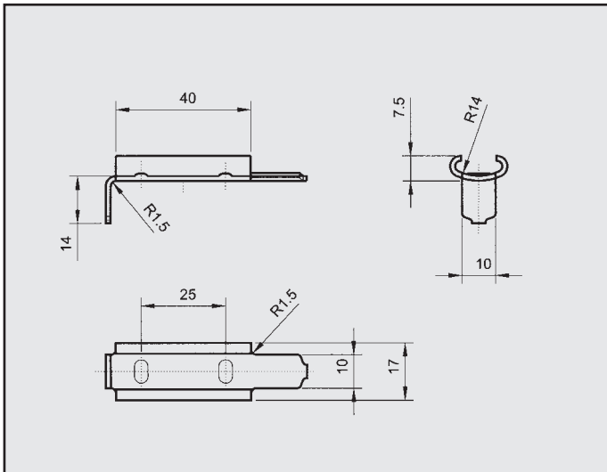
OPEL PIASTRINA COD. PI 520013
