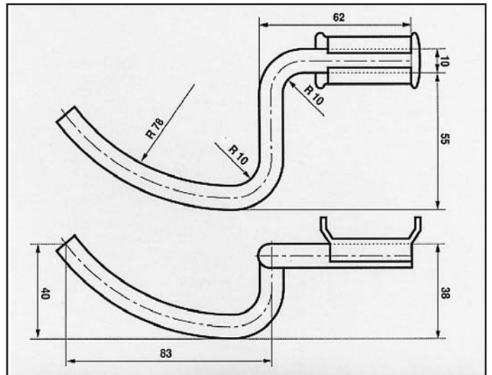
FORD SIERRA 2000 ATTACCO posteriore COD. AT 260622
