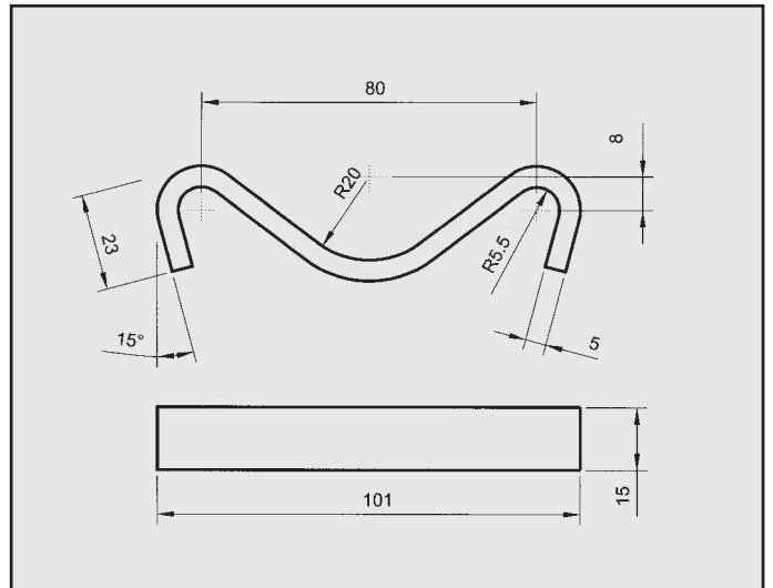
SEAT IBIZA 900 ATTACCO COD. AT 680118
