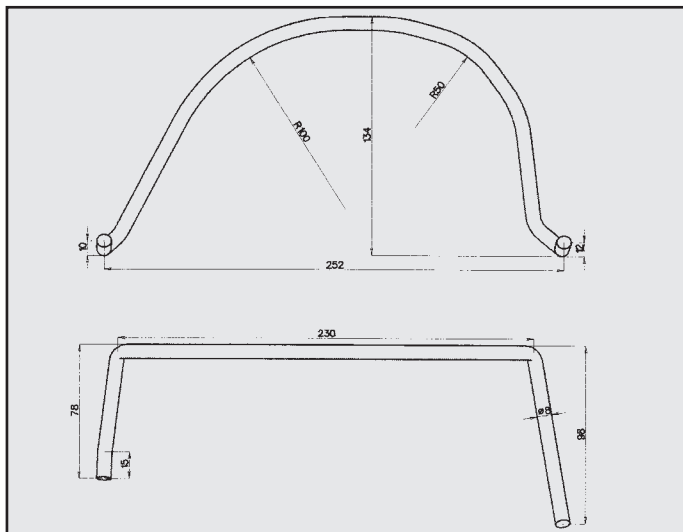
PEUGEOT 106 ATTACCO COD. AT 540807
