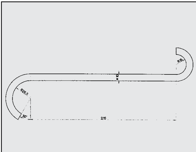
DAIHATSU ATTACCO COD. AT 180008
