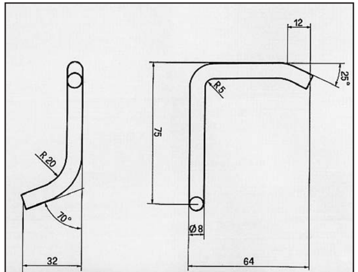
SAMBA 1100 ATTACCO tubo COD. AT 780402
