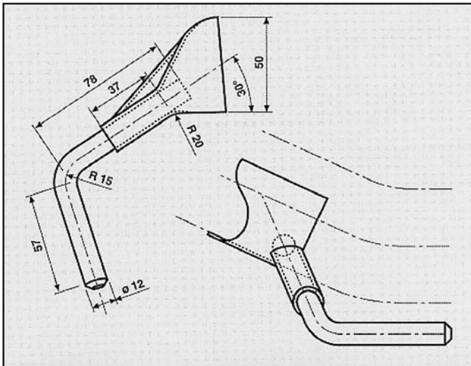
MERCEDES ATTACCO COD. AT 440007
