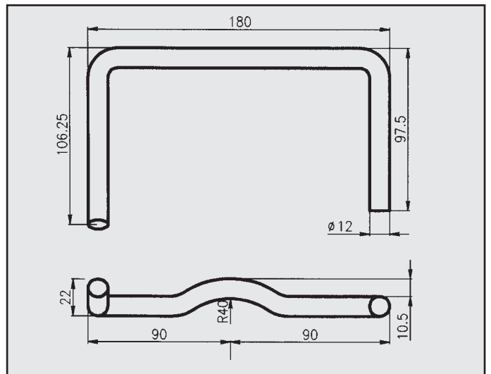
OPEL VECTRA 95 2.0 16V ATTACCO centrale COD. AT 520818
