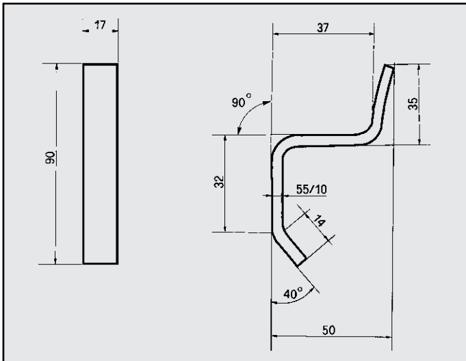
Y10 TURBO ATTACCO COD. AT 080202
