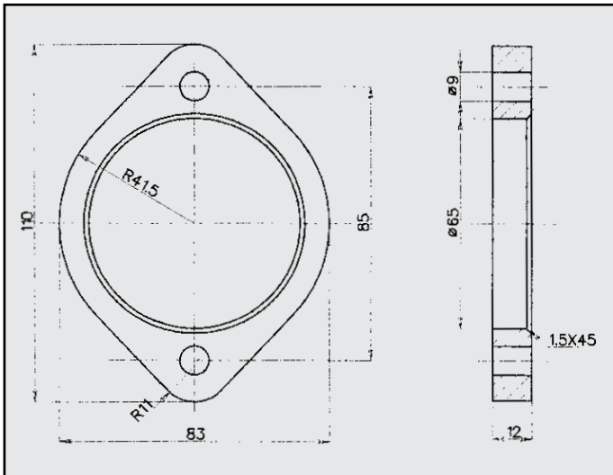
POST. BMW 320 FLANGIA COD. FL 120406
