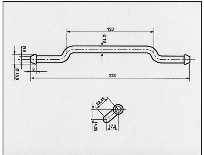
FORD SCORPIO 95 ATTACCO COD. AT 260807
