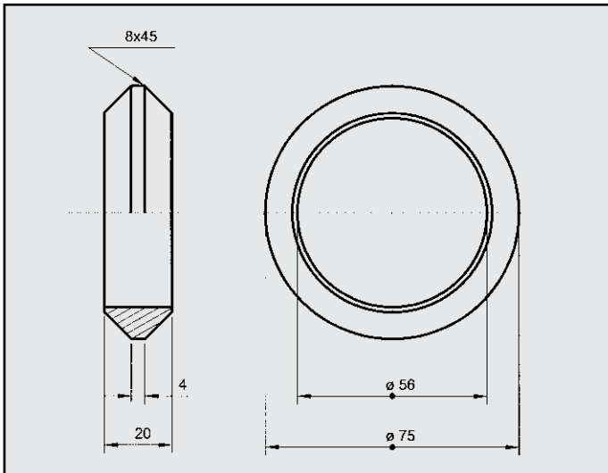
RENAULT R 19 ANELLO COD. AN 600908
