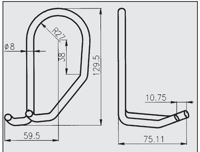
LANCIA DELTA 1.9 - 1.9 TD ATTACCO COD. AT 380814
